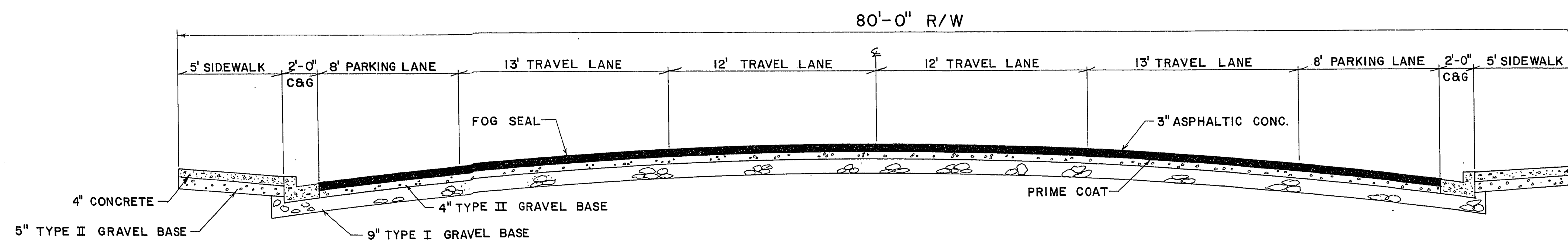
Proposed Typical Cross-section
