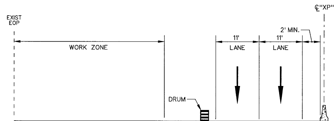
SECTION C-Y
