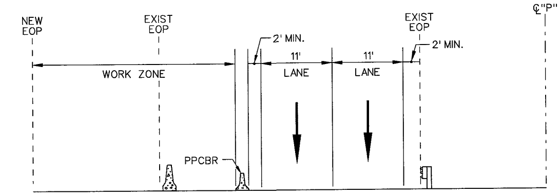
SECTION D-H
