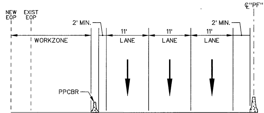
SECTION E-F
