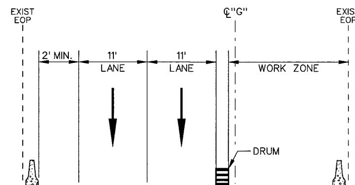
SECTION C-Z
