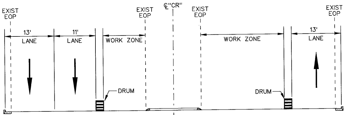
SECTION D-P
