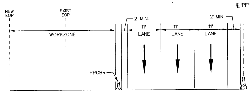
SECTION D-X
