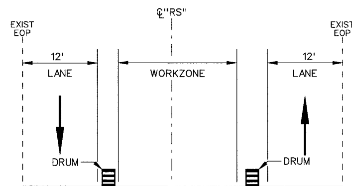
SECTION E-H
