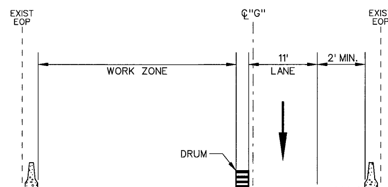
SECTION D-B
