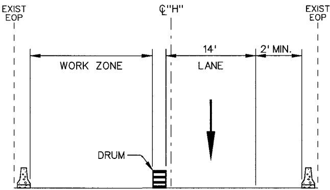
SECTION C-W
