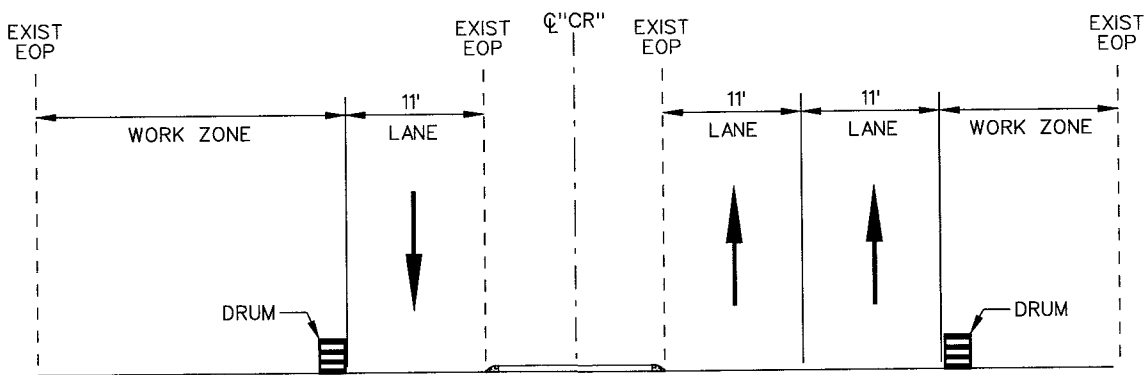
SECTION D-N
