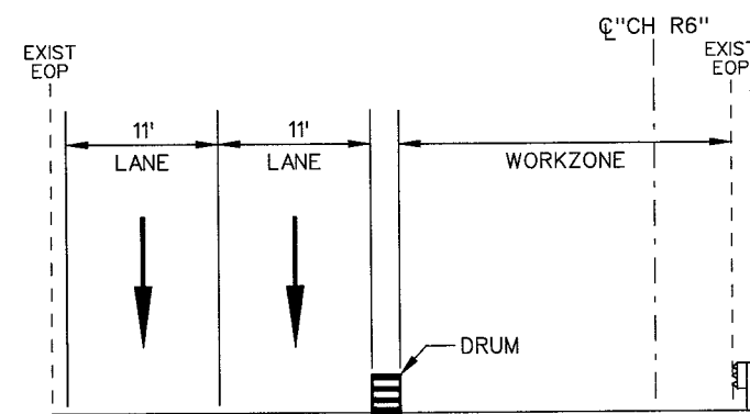
SECTION D-Z
