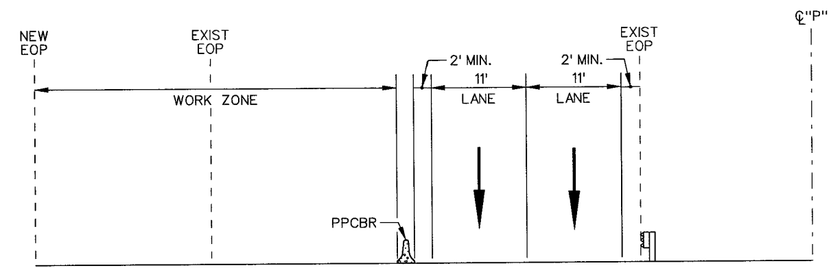
SECTION D-F
