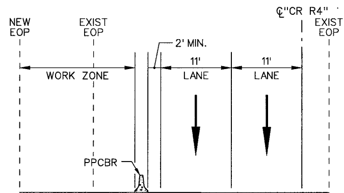
SECTION D-K
