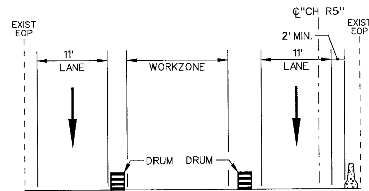
SECTION D-Y
