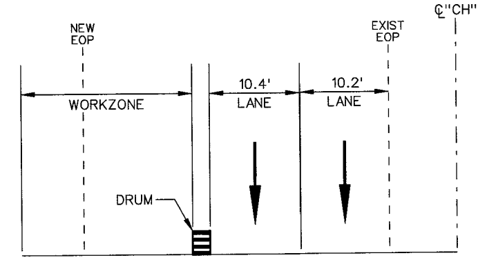
SECTION D-U
