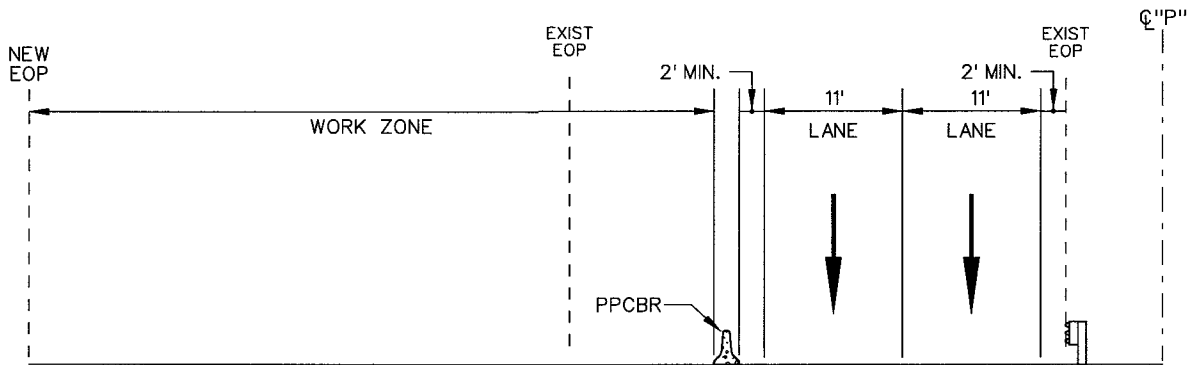
SECTION C-U
