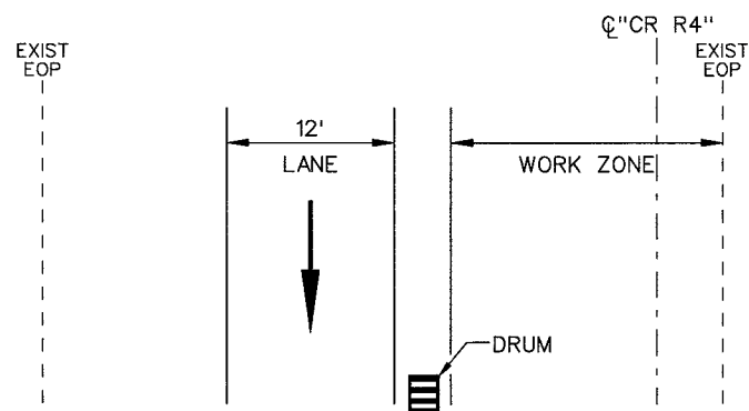
SECTION D-L
