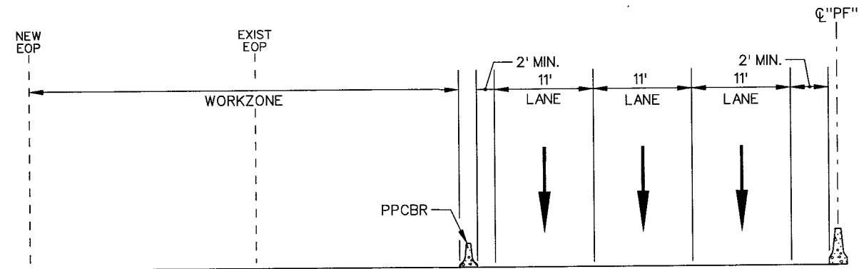
SECTION D-R
