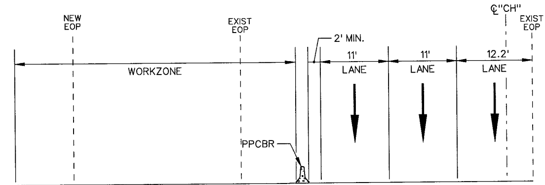
SECTION D-W
