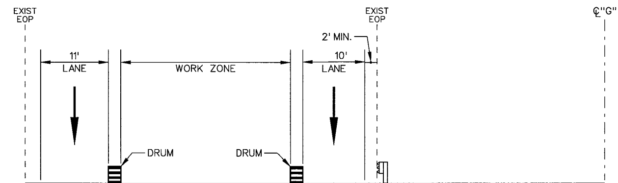
SECTION D-C
