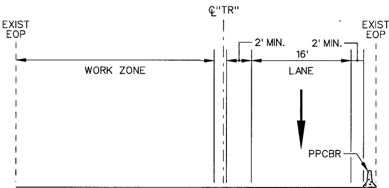
SECTION C-R
