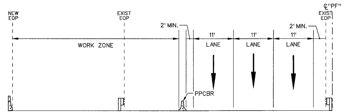
SECTION D-M
