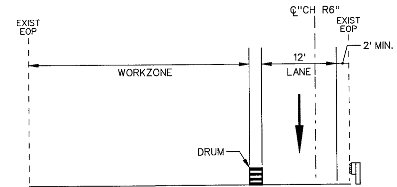
SECTION E-C
