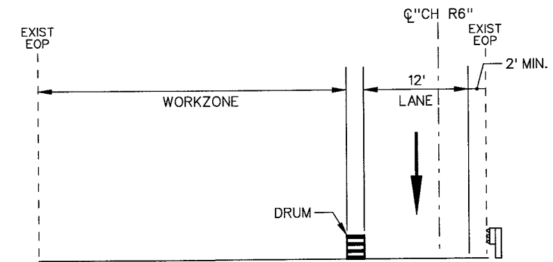
SECTION E-C
