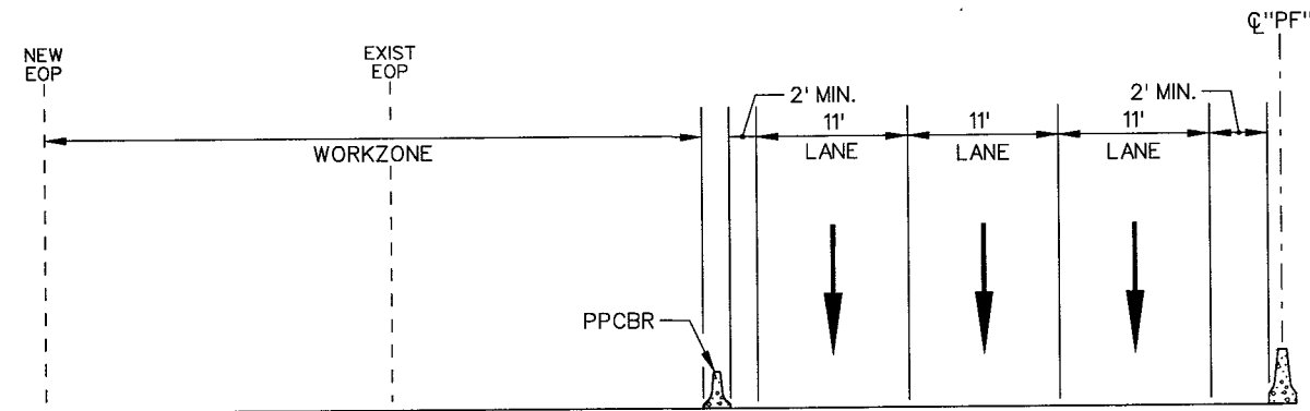
SECTION D-R
