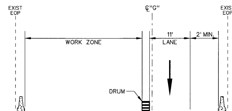
SECTION D-B
