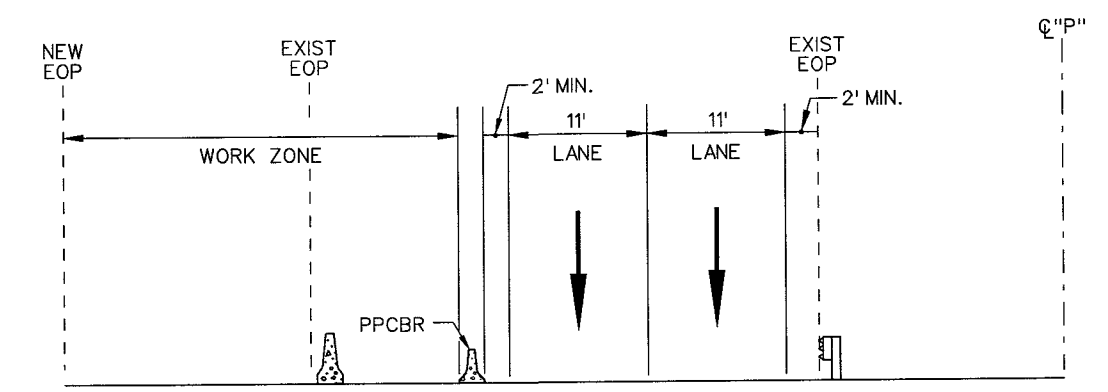
SECTION D-H
