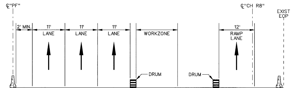
SECTION B-O
