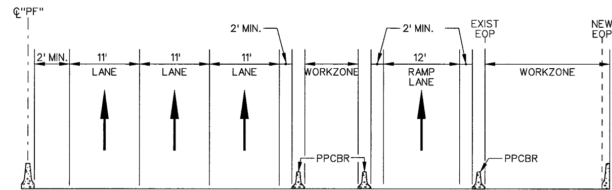
SECTION B-M
