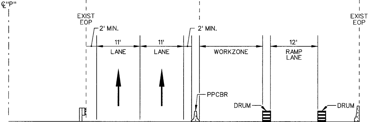
SECTION C-B
