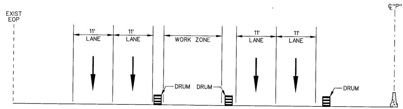
SECTION C-L
