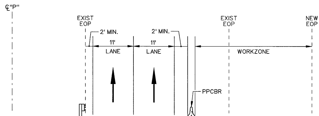
SECTION B-W
