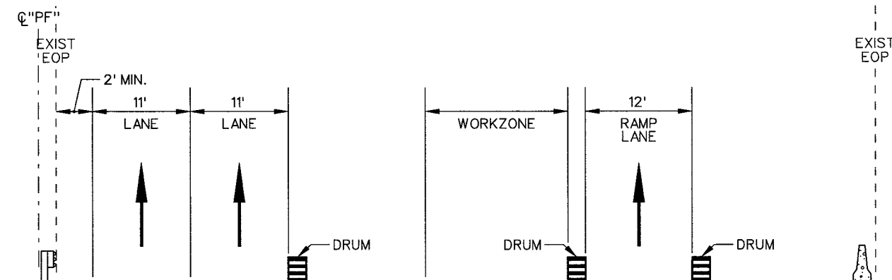
SECTION B-Q
