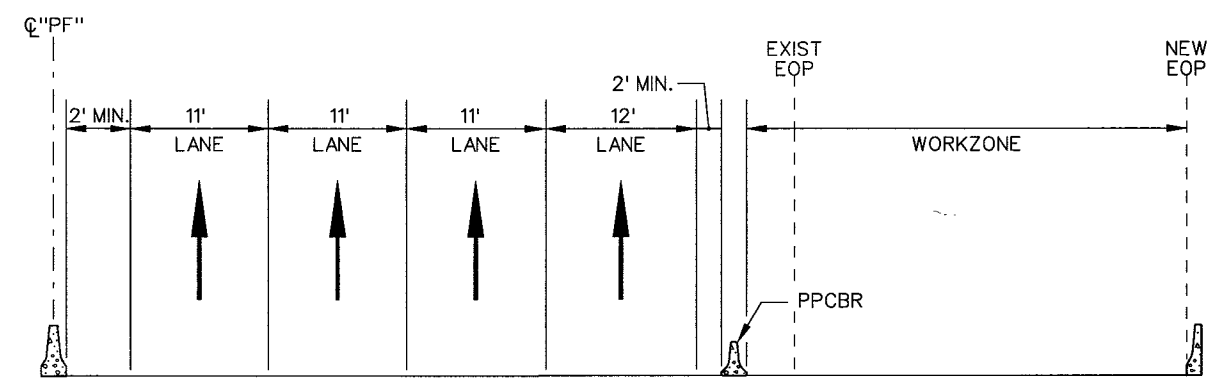
SECTION B-N
