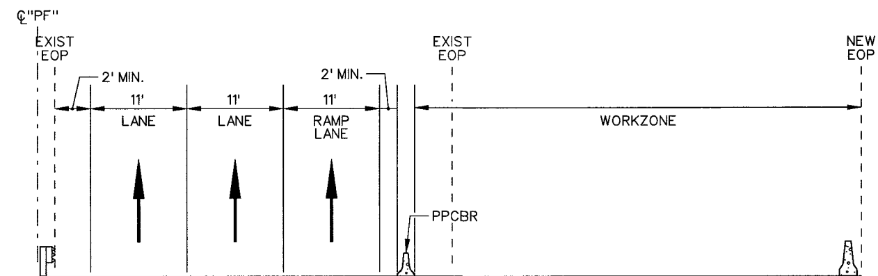
SECTION B-P
