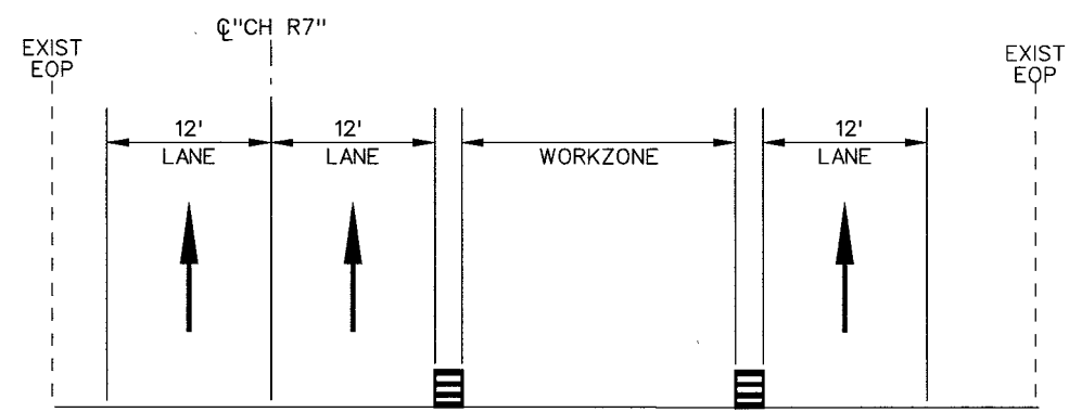
SECTION B-S
