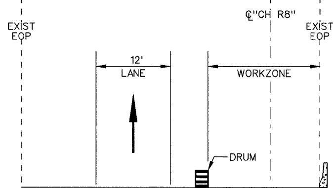
SECTION B-J
