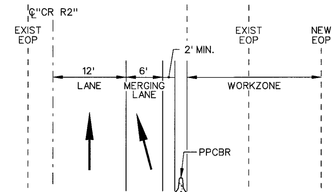
SECTION B-Y
