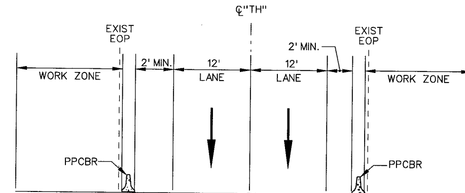
SECTION C-P
