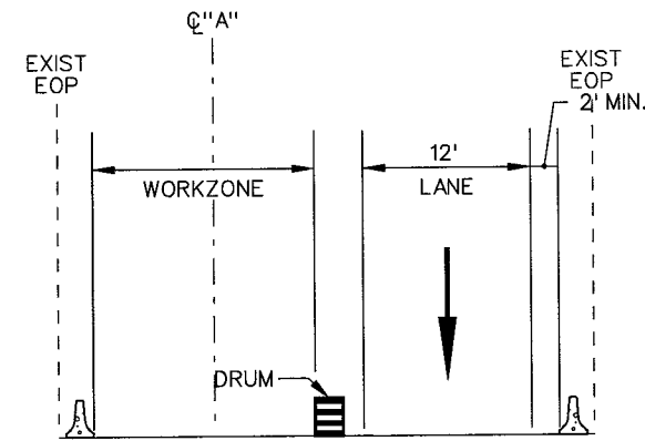
SECTION C-G
