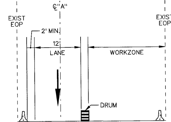
SECTION C-H
