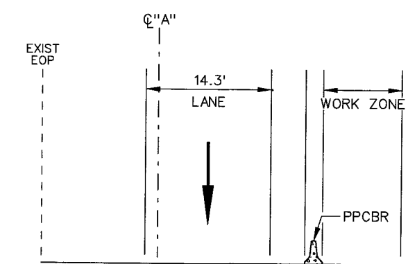
SECTION C-O
