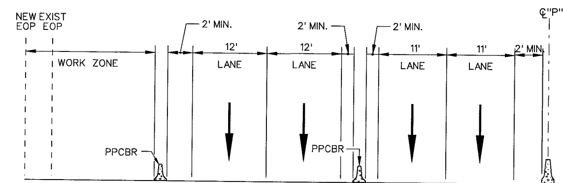
SECTION C-Q
