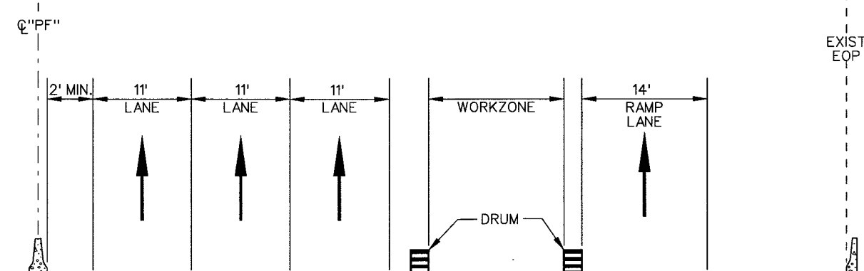
SECTION B-L
