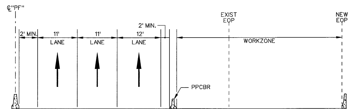
SECTION B-K
