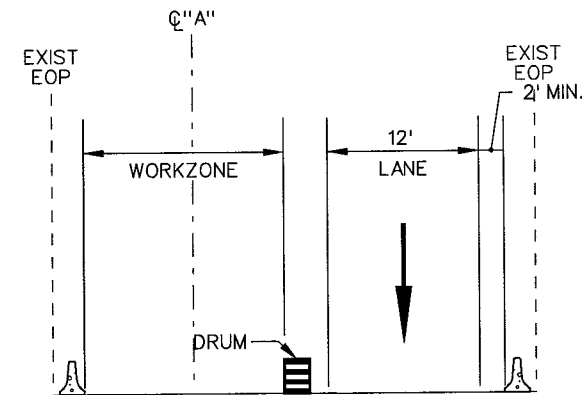
SECTION C-G
