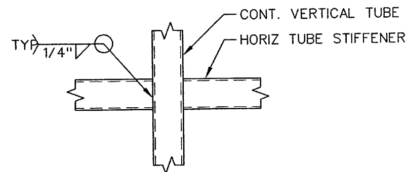
4 TUBE STIFFENER JOINT DETAIL (VIEW FROM INSIDE)
