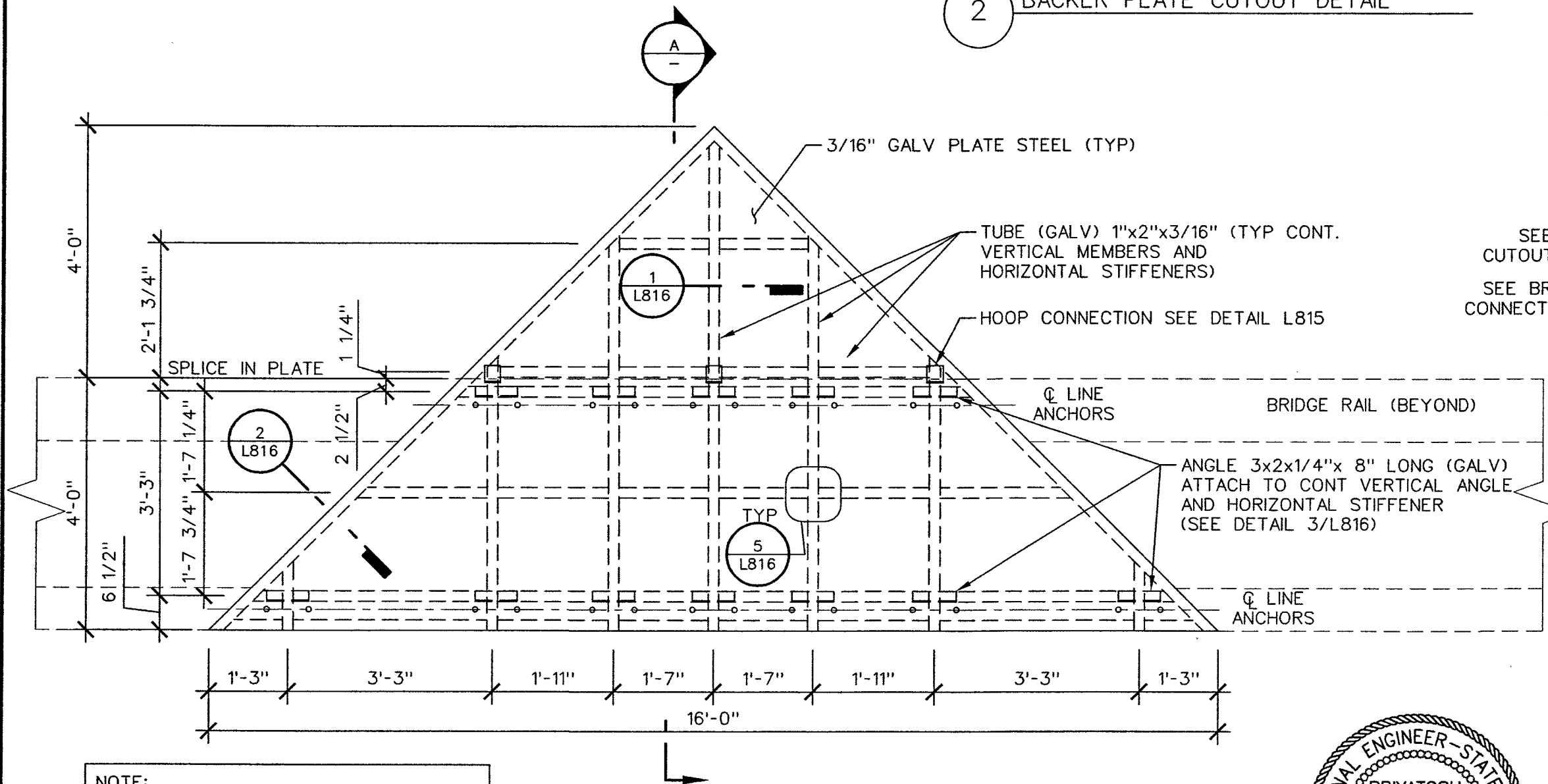
1A TRIANGULAR PANEL FRAMING DETAIL BRIDGE RAIL CONDITION 1
