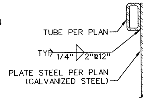
2 TUBE CONNECTION DETAIL
