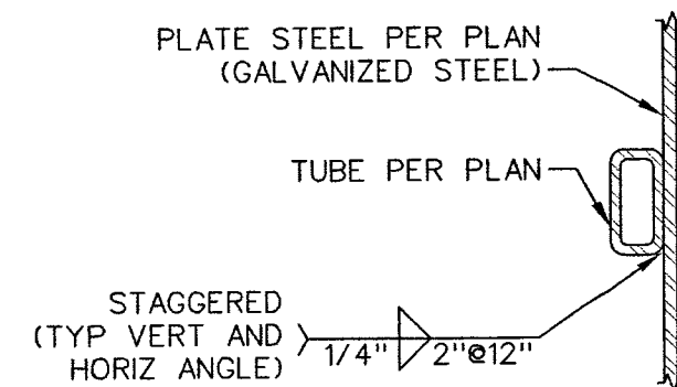
1 TUBE CONNECTION DETAIL
