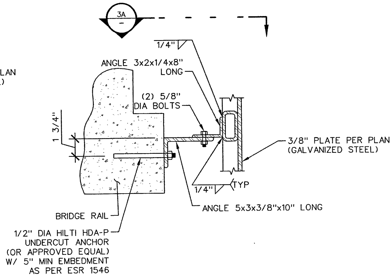
3 TRIANGULAR PANEL CONNECTION @ BRIDGE RAIL
