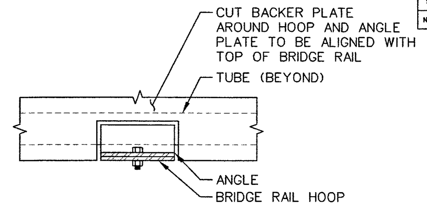
2 BACKER PLATE CUTOUT DETAIL
