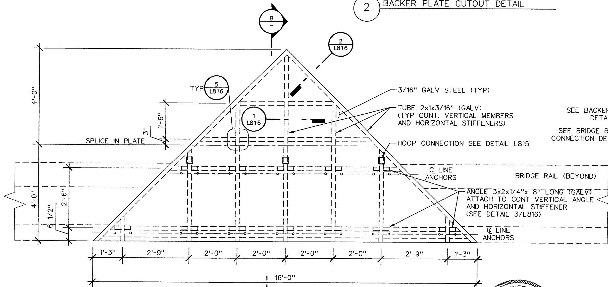
2 BACKER PLATE CUTOUT DETAIL
