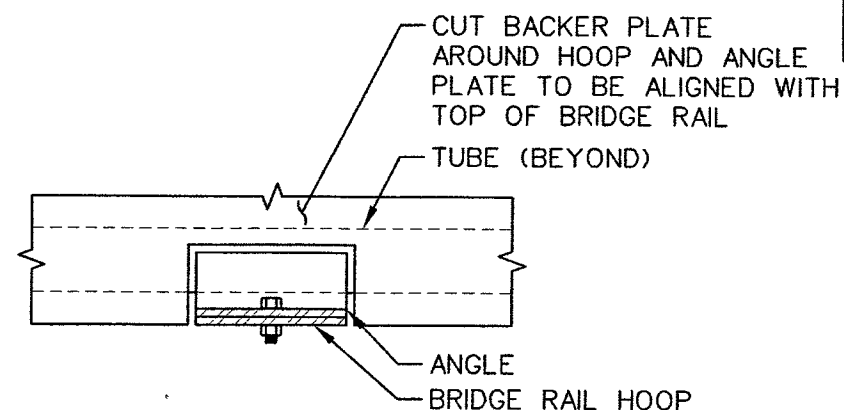
2 BACKER PLATE CUTOUT DETAIL
