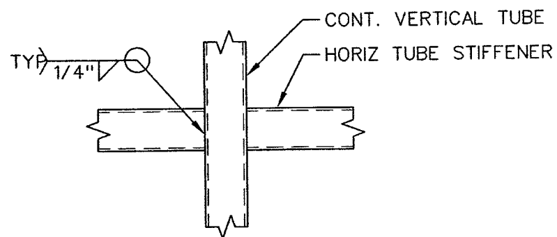
4 TUBE STIFFENER JOINT DETAIL (VIEW FROM INSIDE)
