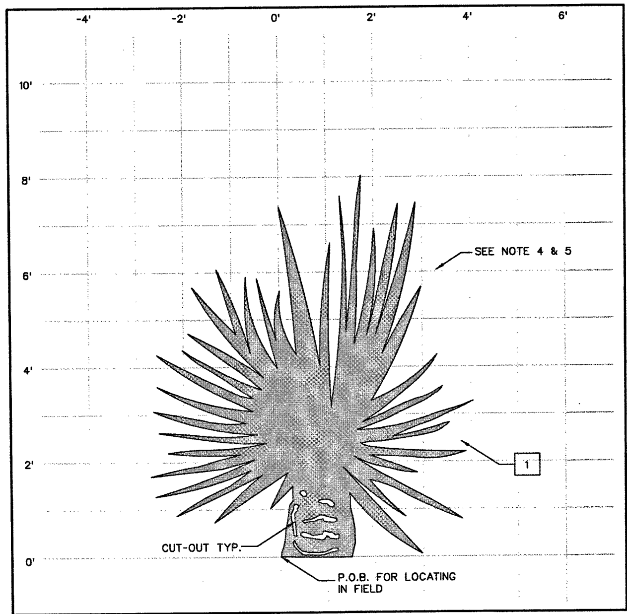
1 GALVANIZED STEEL IMAGE PANEL "A-2"
