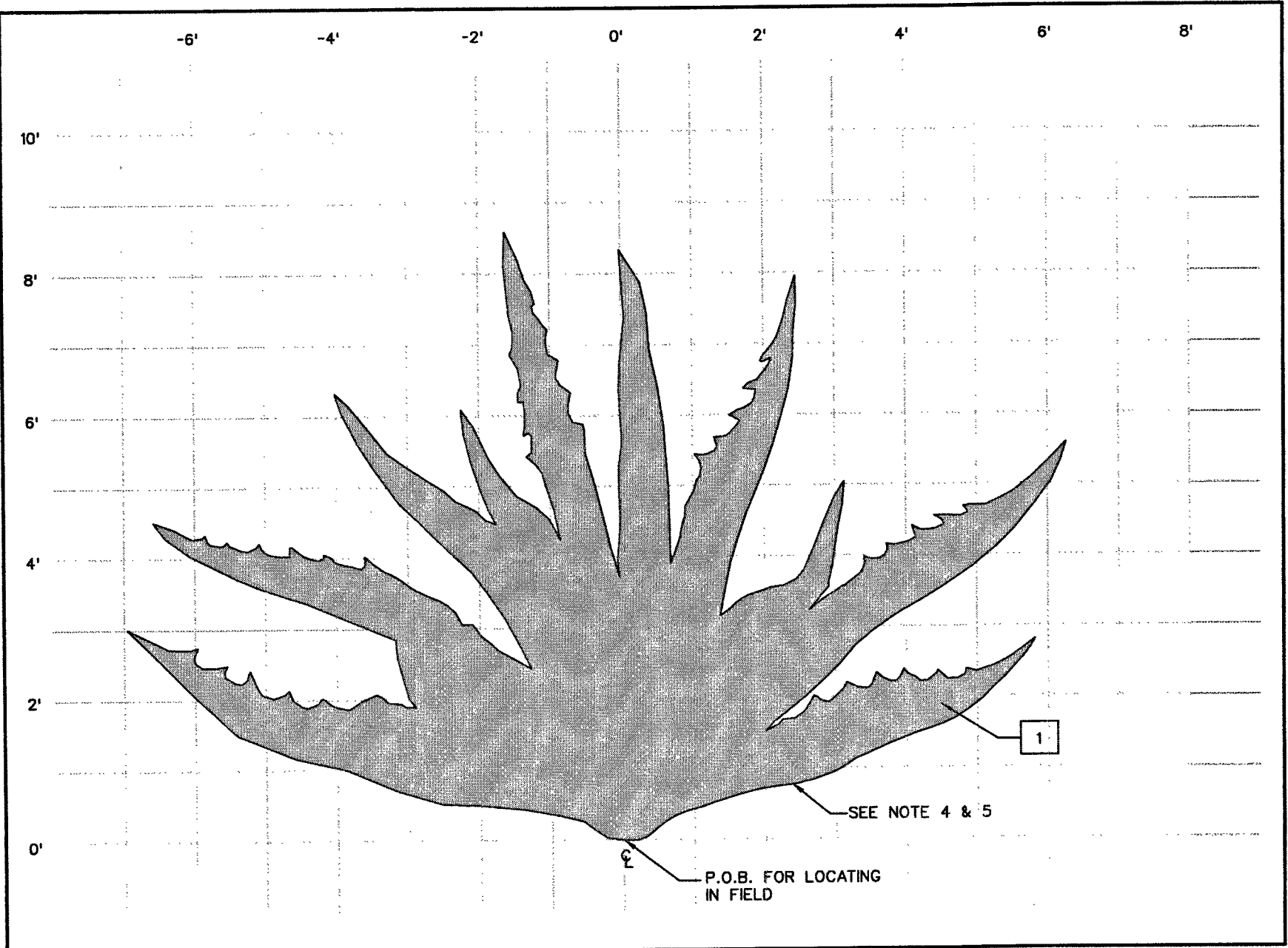
1 GALVANIZED STEEL IMAGE PANEL "D-2"
