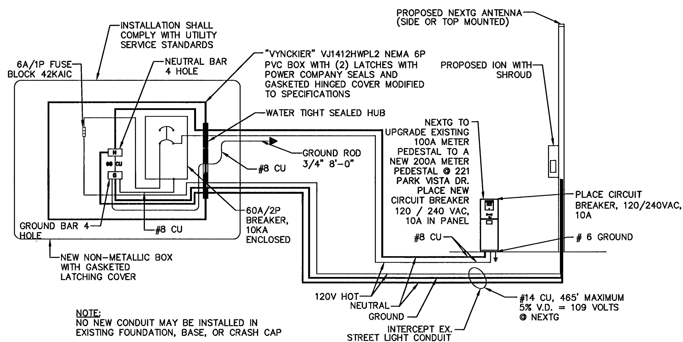
POWER SINGLE LINE DIAGRAM NTS
