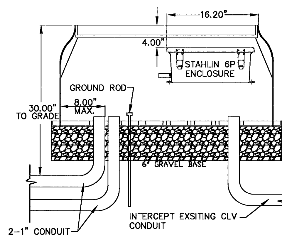
FRONT VIEW
