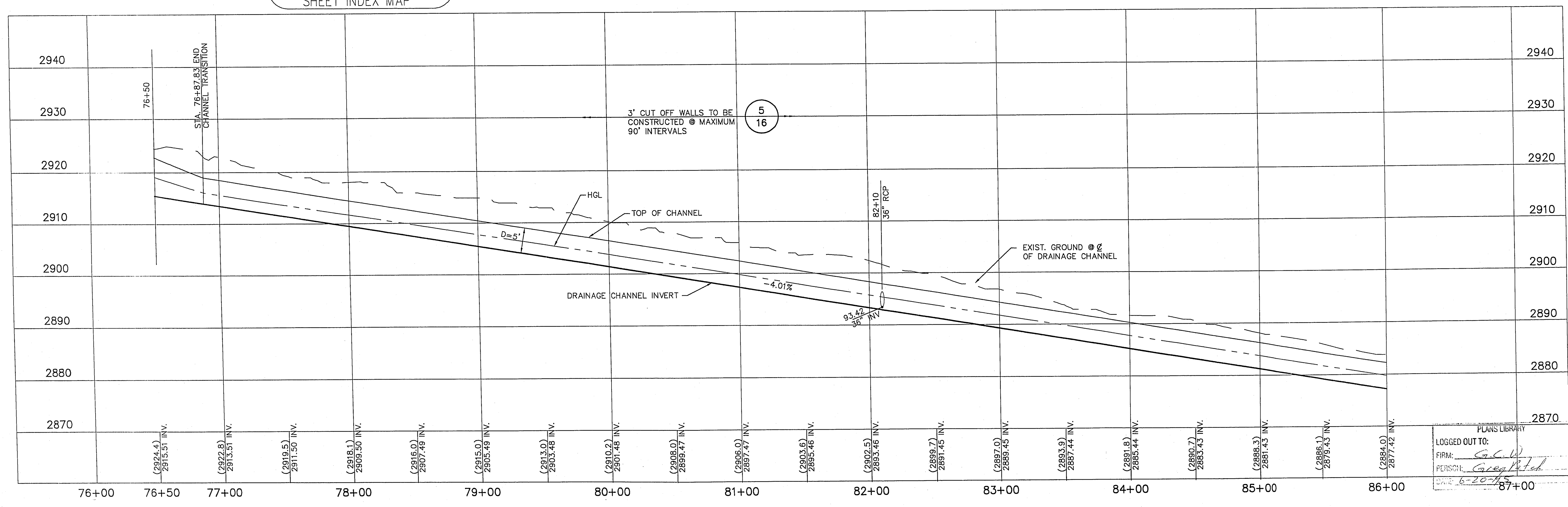
SUMMERLIN PARKWAY DRAINAGE CHANNEL SCALE: 1" = 40' HORIZONTAL 1" = 10' VERTICAL
