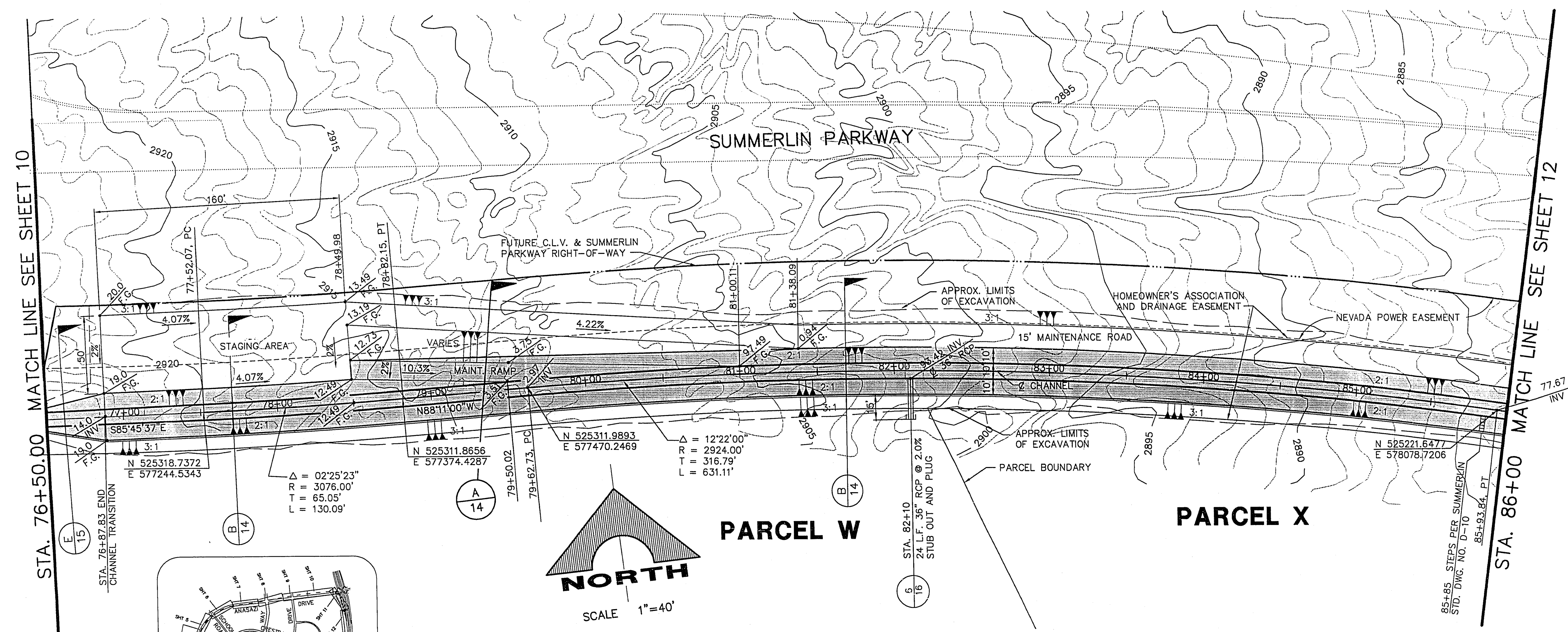
SUMMERLIN PARKWAY DRAINAGE CHANNEL SCALE: 1" = 40' HORIZONTAL 1" = 10' VERTICAL
