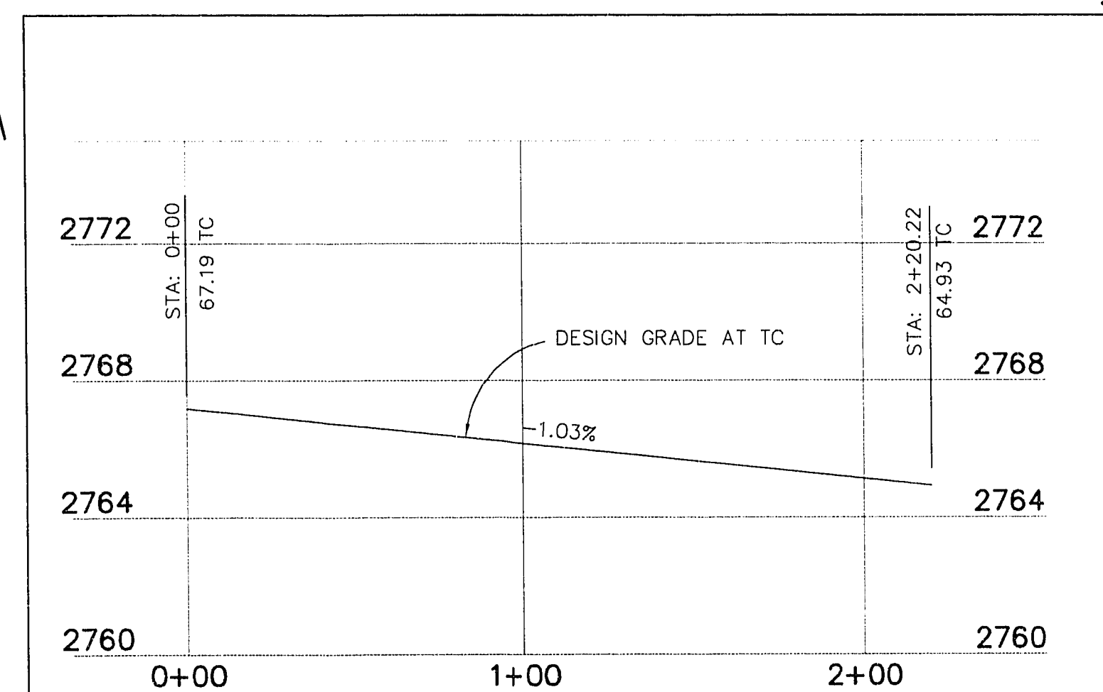
PROFILE "A" SCALE: HORIZ. 1" = 40' VERT. 1" = 4'
