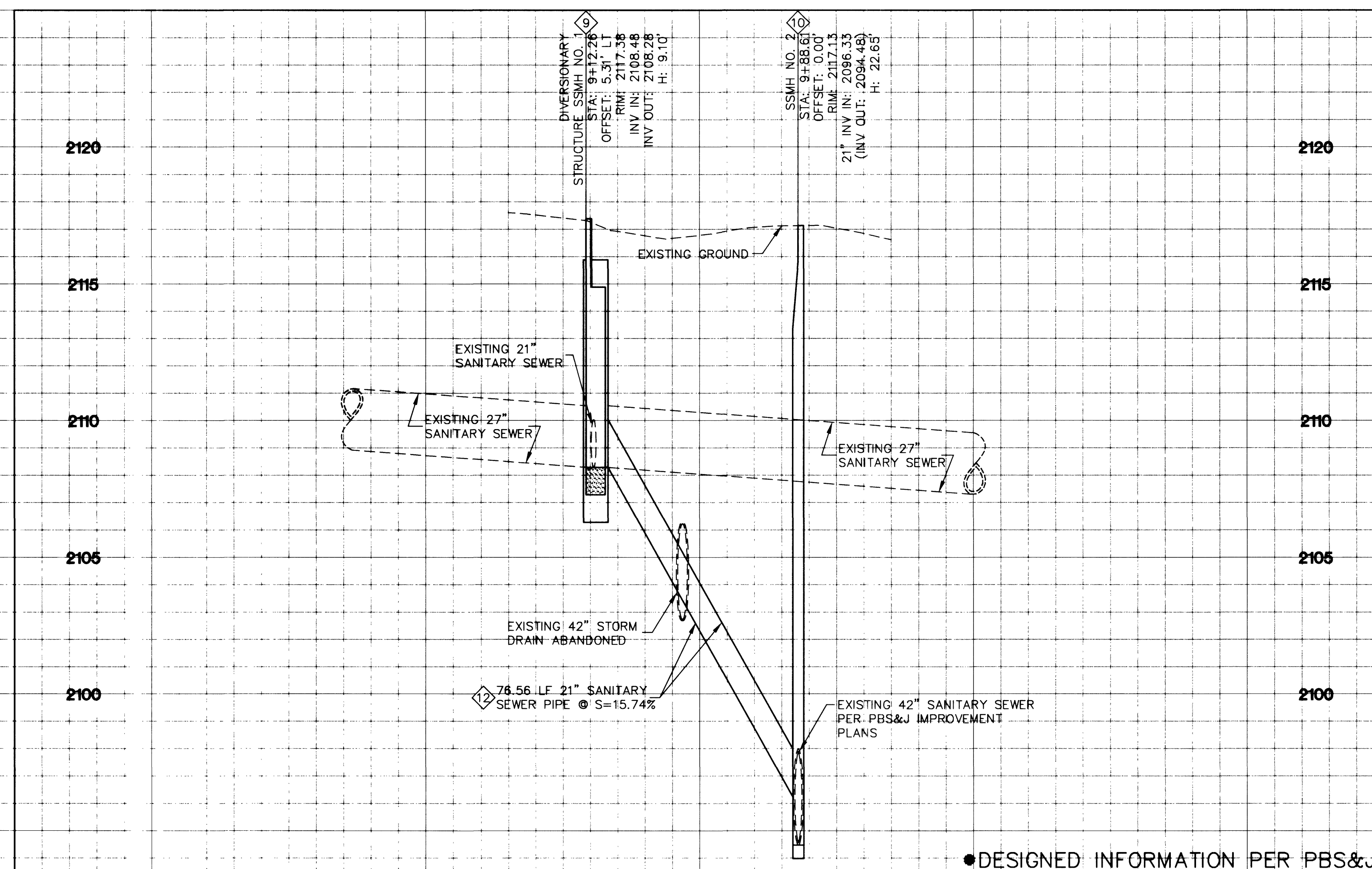
VEGAS DRIVE & RANCHO DRIVE DIVERSIONARY SEWER LINE PROFILE
