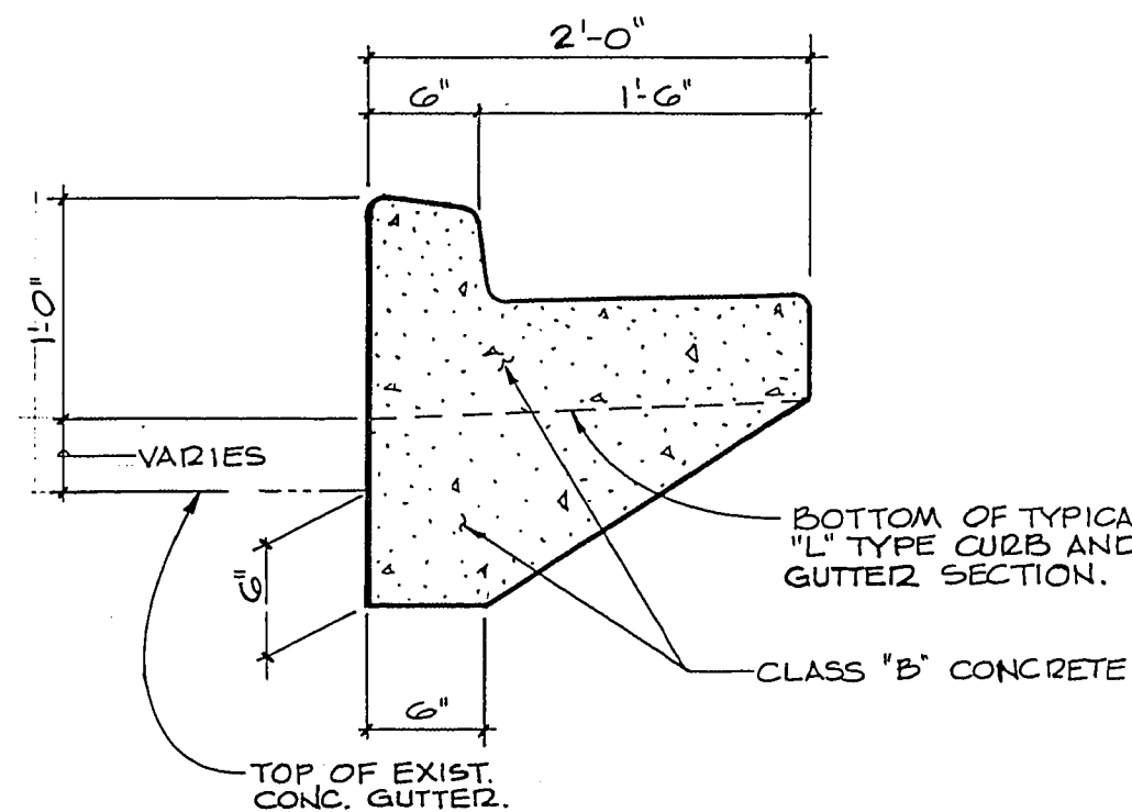
MODIFIED "L" TYPE CURB &amp; GUTTER
