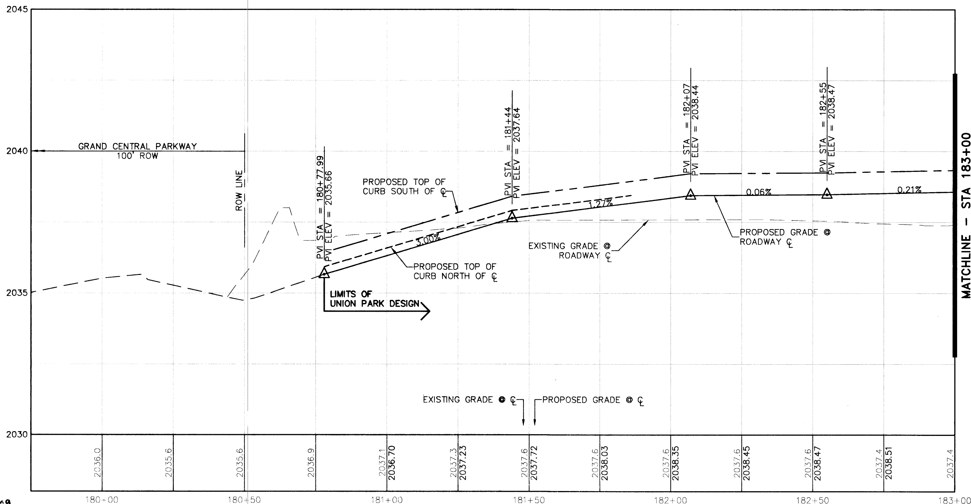
PROFILE VIEW - STREET A1-A2
