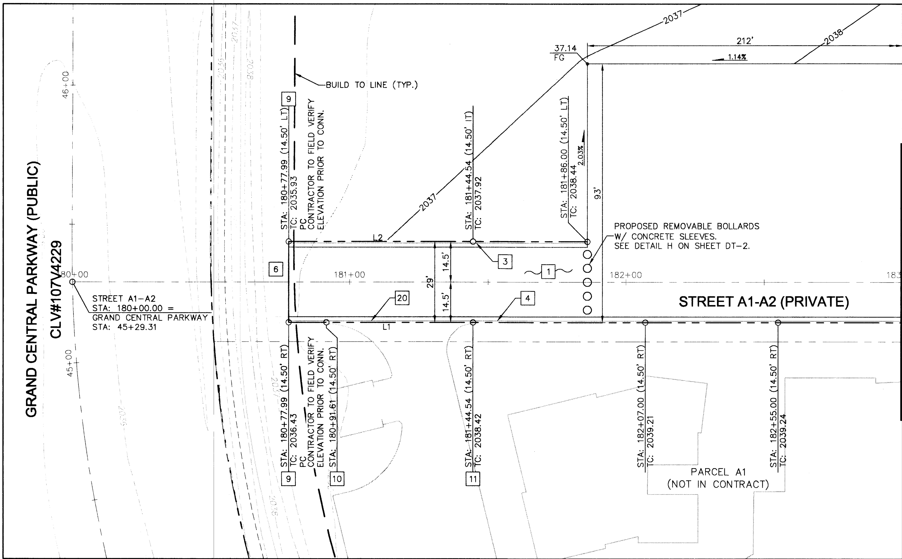
PLAN VIEW - STREET A1-A2
