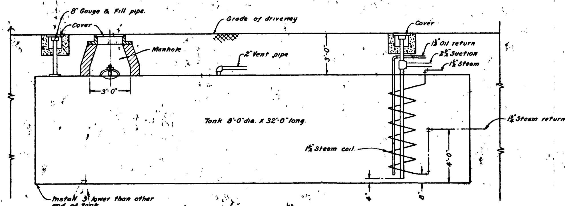
DETAIL OF OIL STORAGE TANK. SCALE 1/2" = 1'-0"
