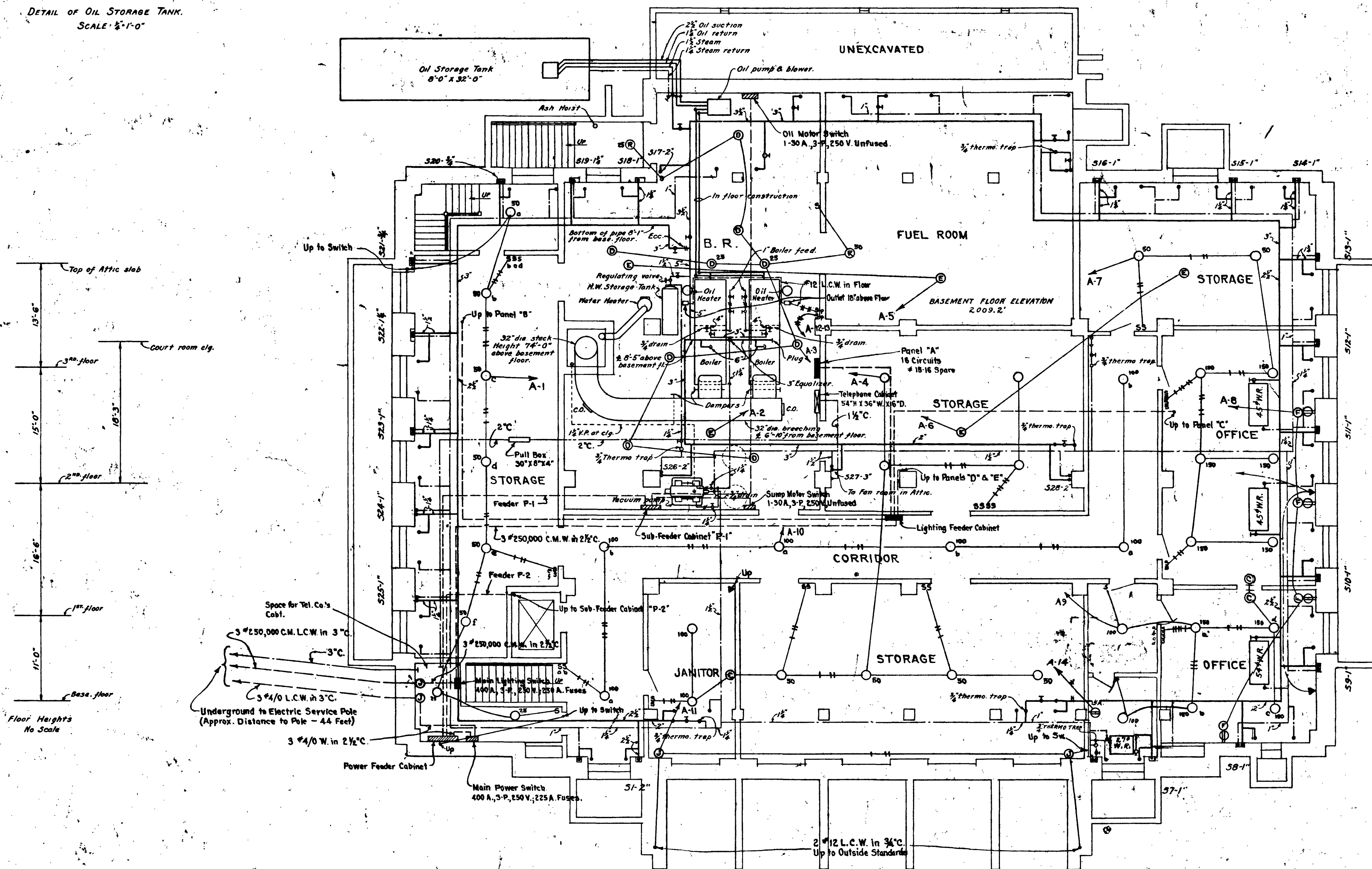
BASEMENT FLOOR PLAN
