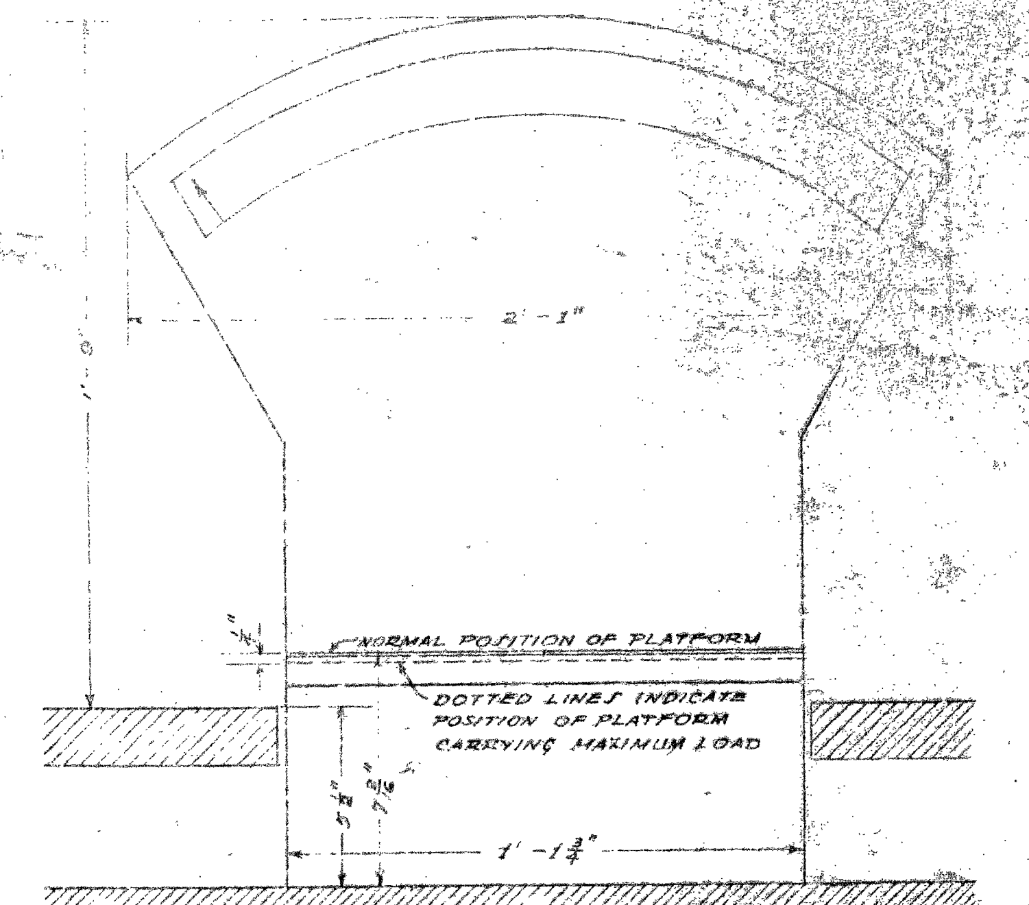
DIAGRAMATIC ELEVATION OF SCALE SCALE 3" = 1'-0"
