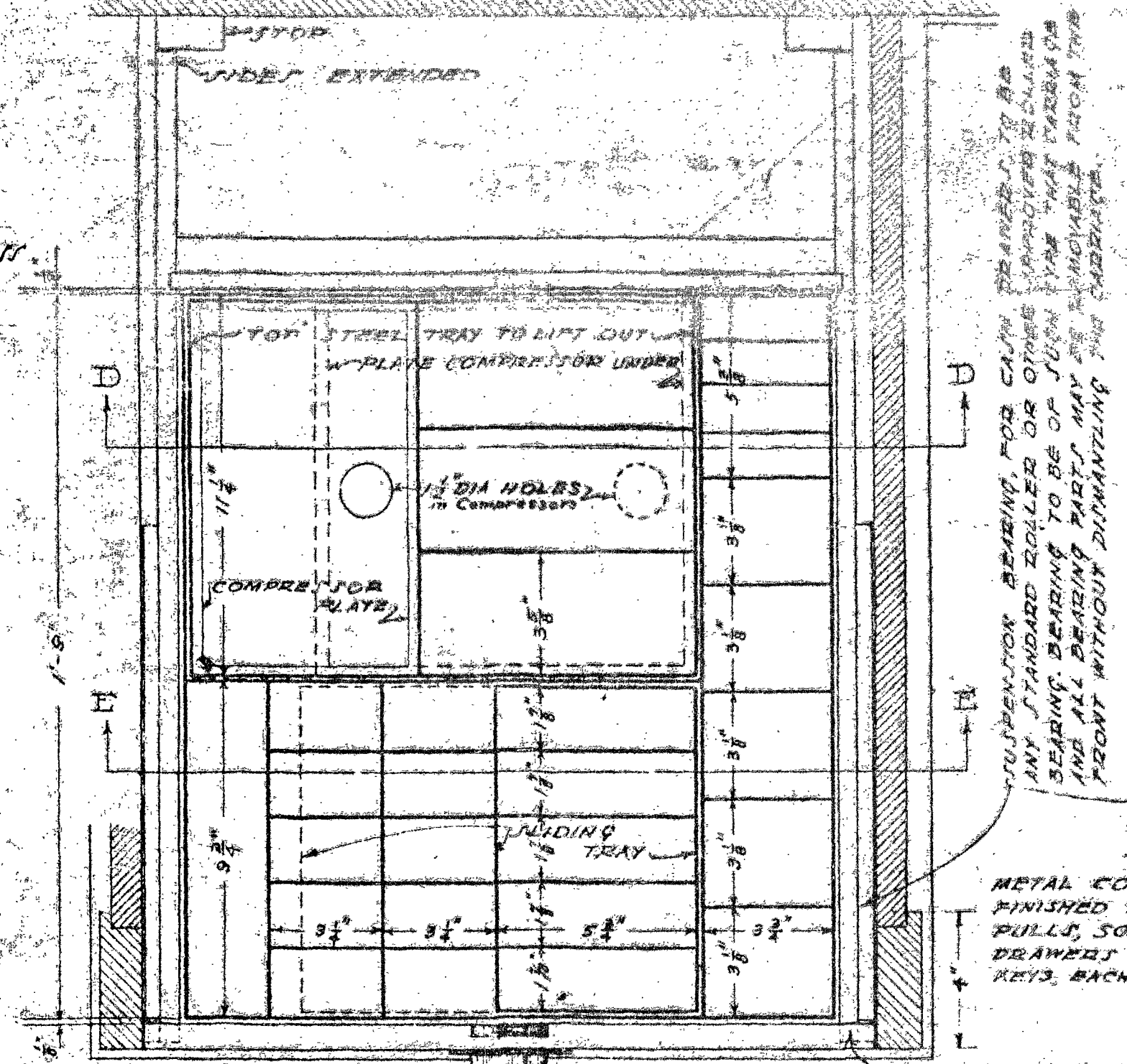
NOTE: THIS TYPE OF DRAWER APPLIES TO PARCEL POST WINDOW ONLY. DETAILS OF CASH AND STAMP DRAWER SCALE 3 INCHES = 1'-0"
