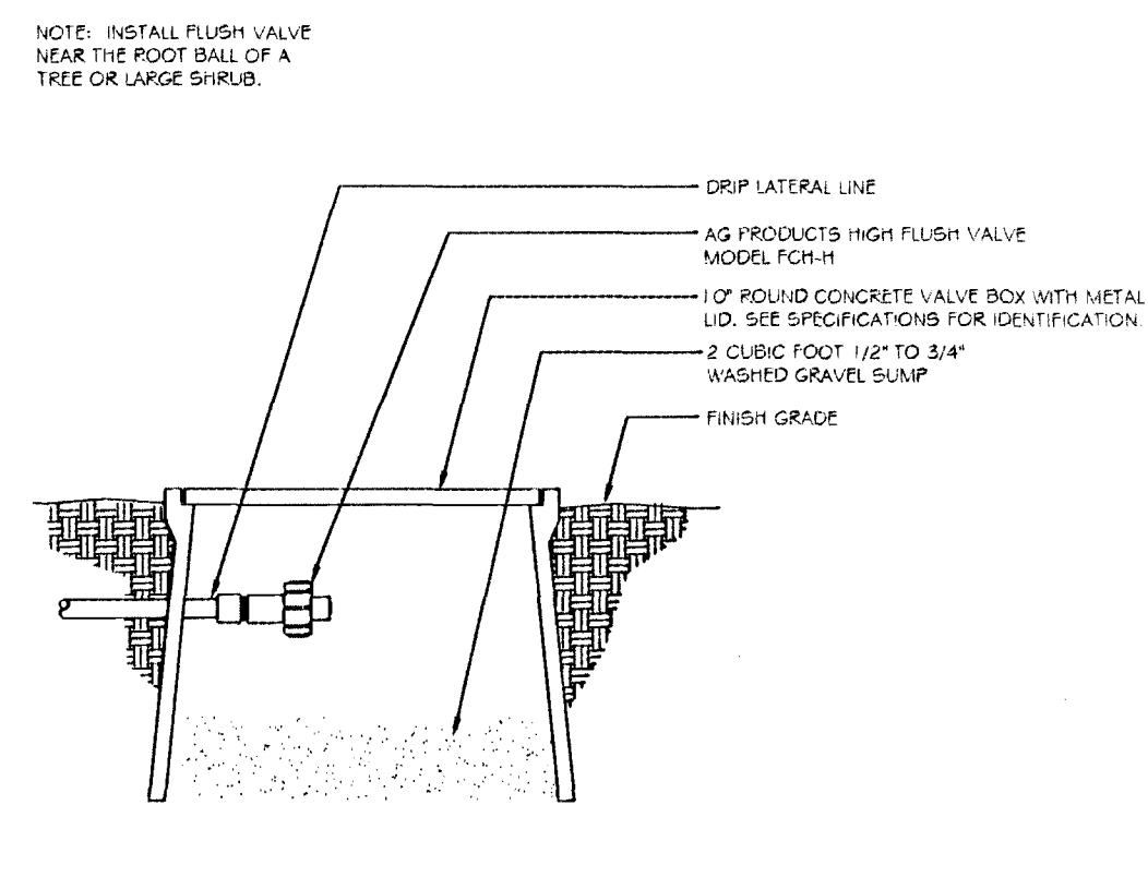
J END FLUSH VALVE
