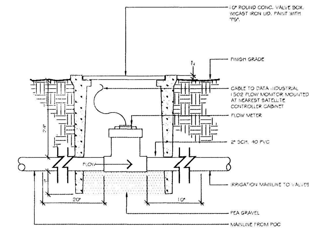
D FLOW METER/SENSOR DETAIL
