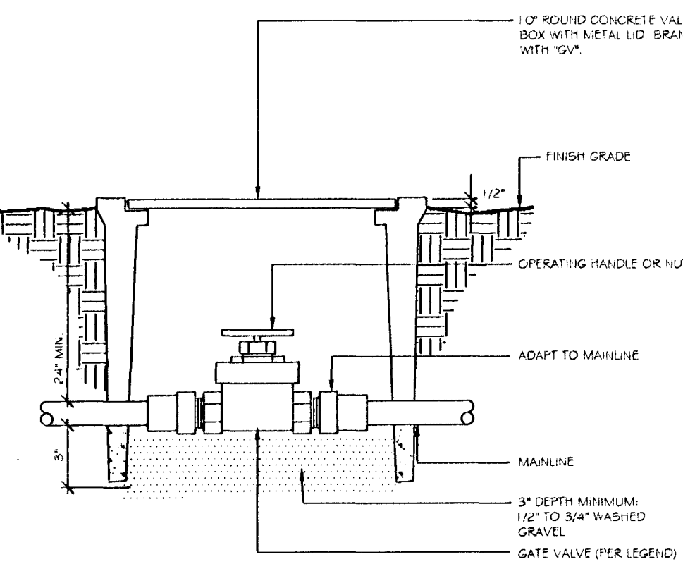
E GATE VALVE
