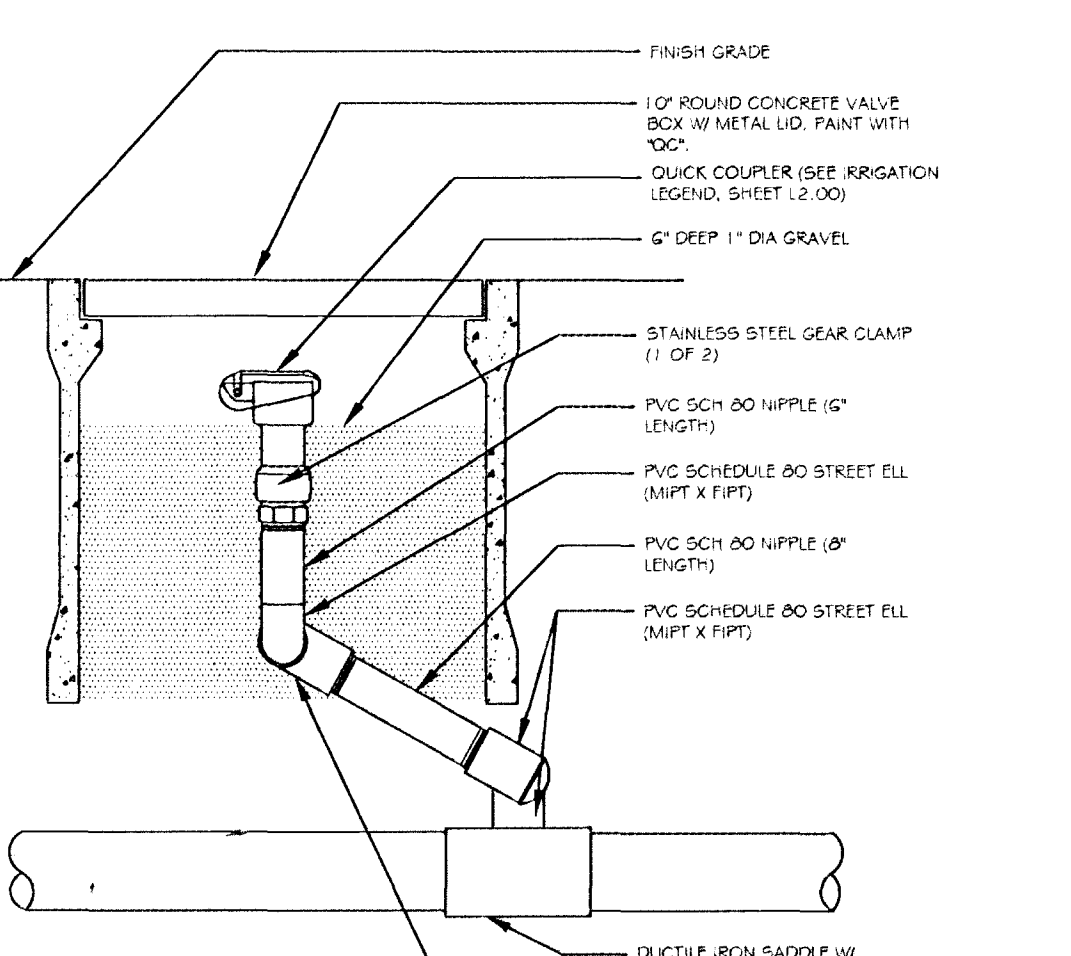
M QUICK COUPLER VALVE
