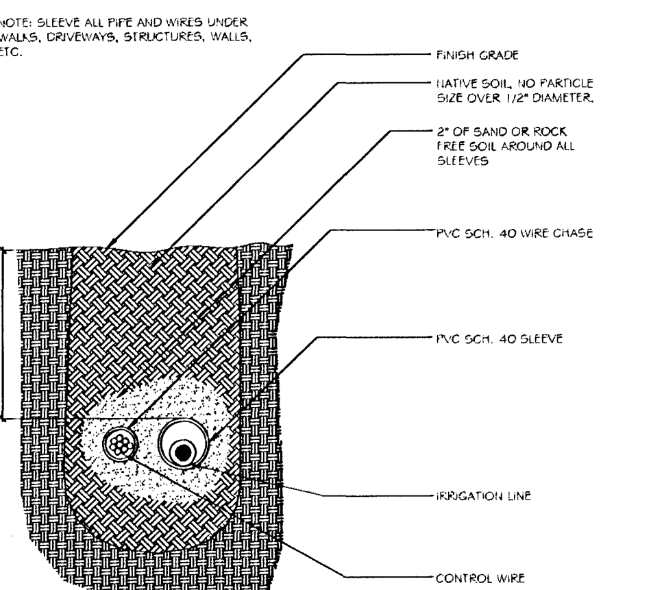
I SLEEVE SECTION
