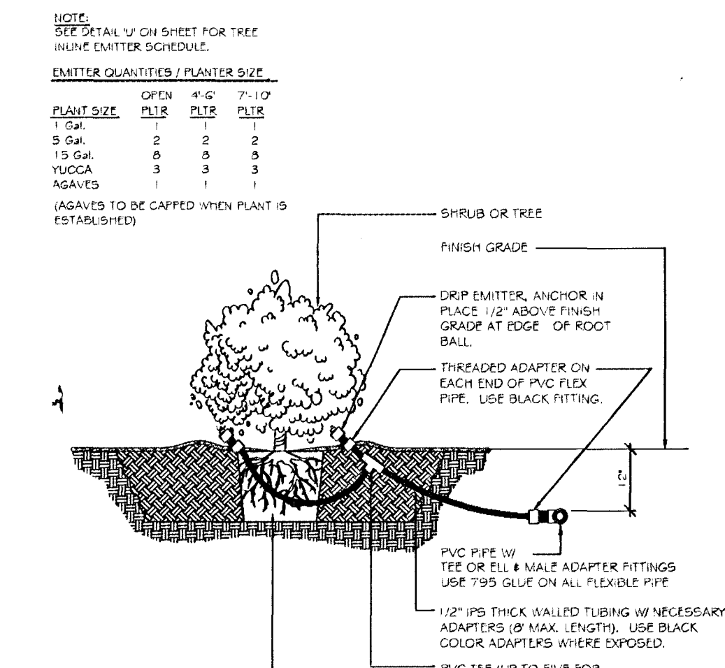
K SHRUB DRIP EMITTER
