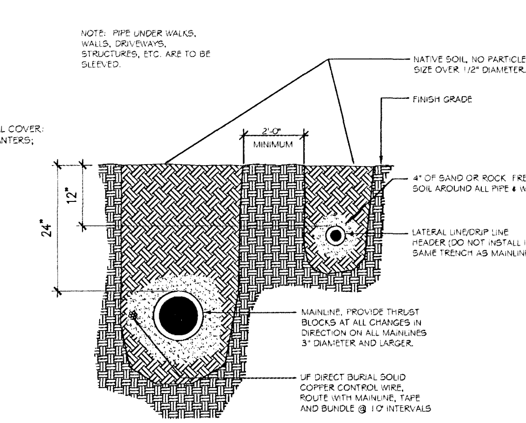
H TRENCH SECTION
