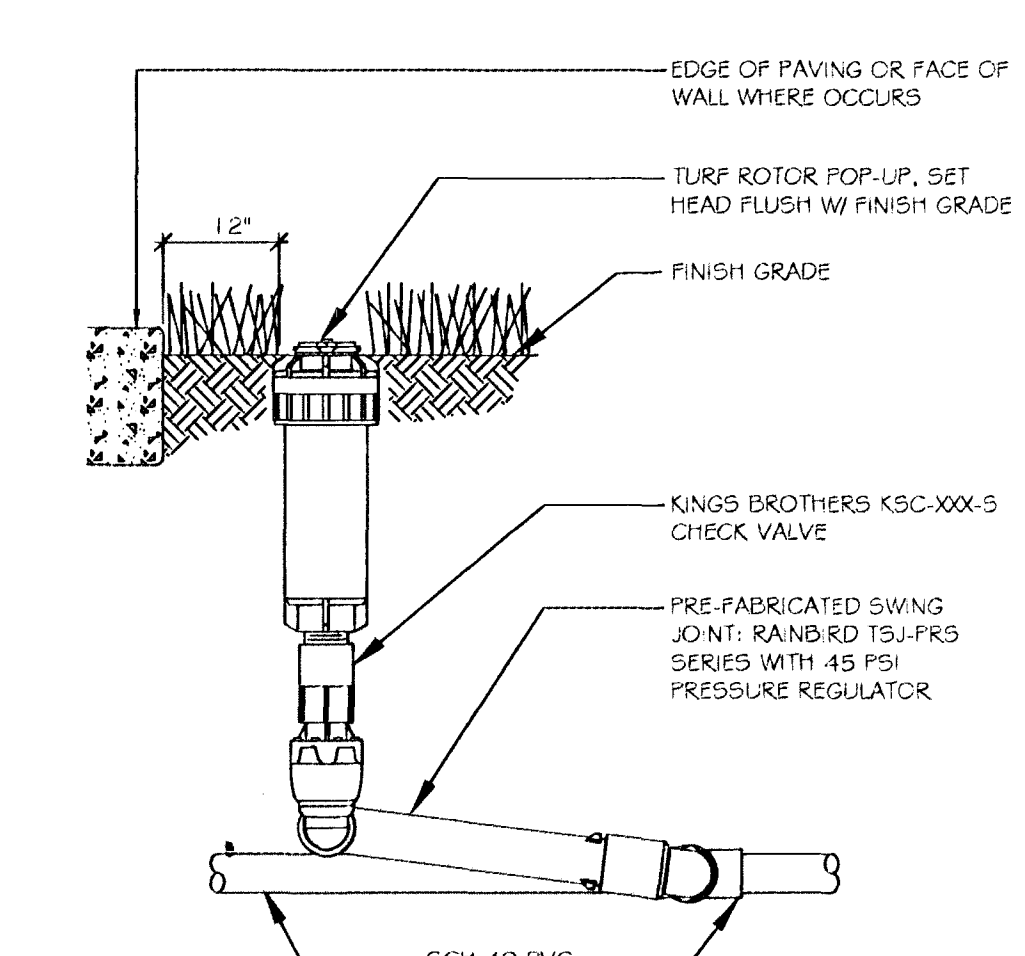
L TURF ROTOR HEAD
