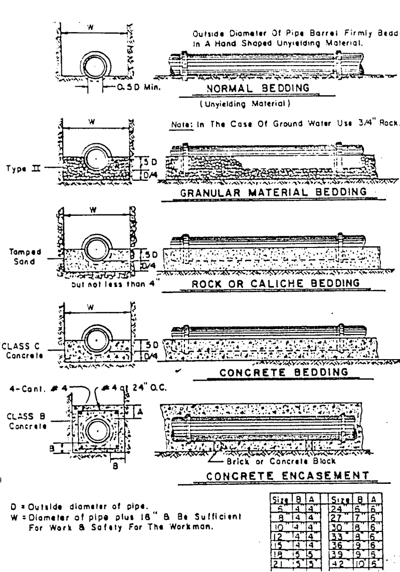
PIPE BEDDING METHODS DWG. NO. 505
