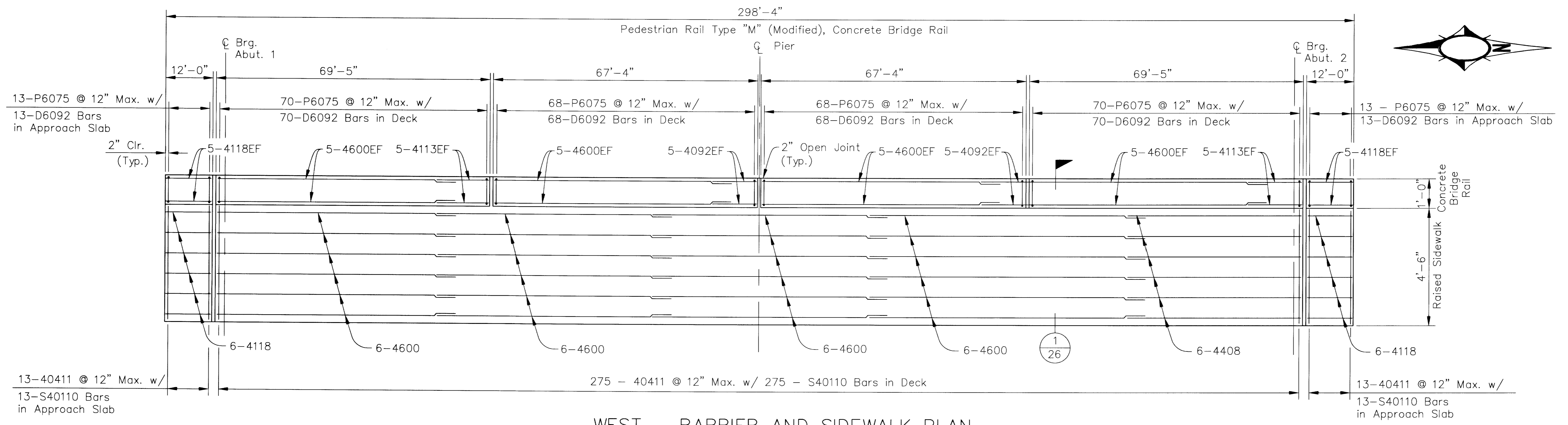
WEST - BARRIER AND SIDEWALK PLAN
