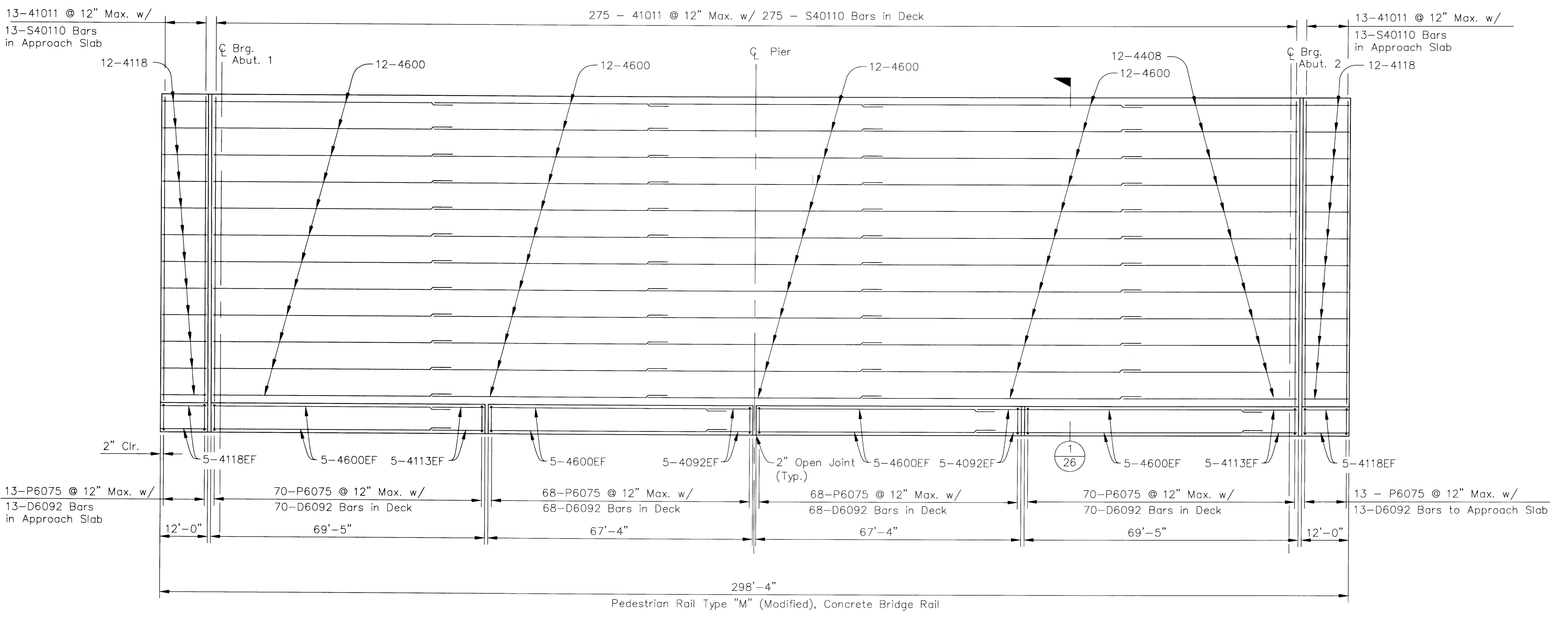
EAST - BARRIER AND SIDEWALK PLAN
