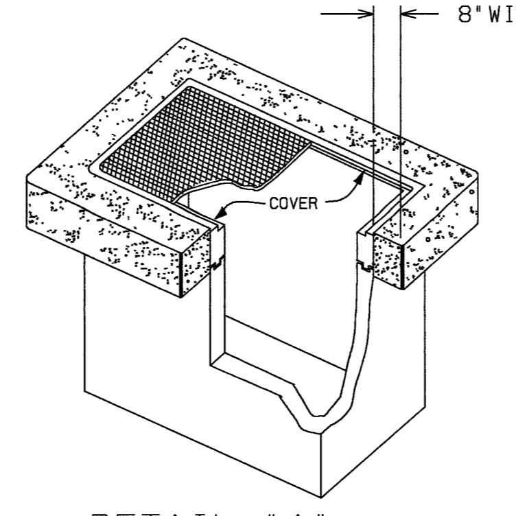
DETAIL "A" FOR COLLAR THICKNESS REFER TO SPRINT SPECIFICATION 8000
