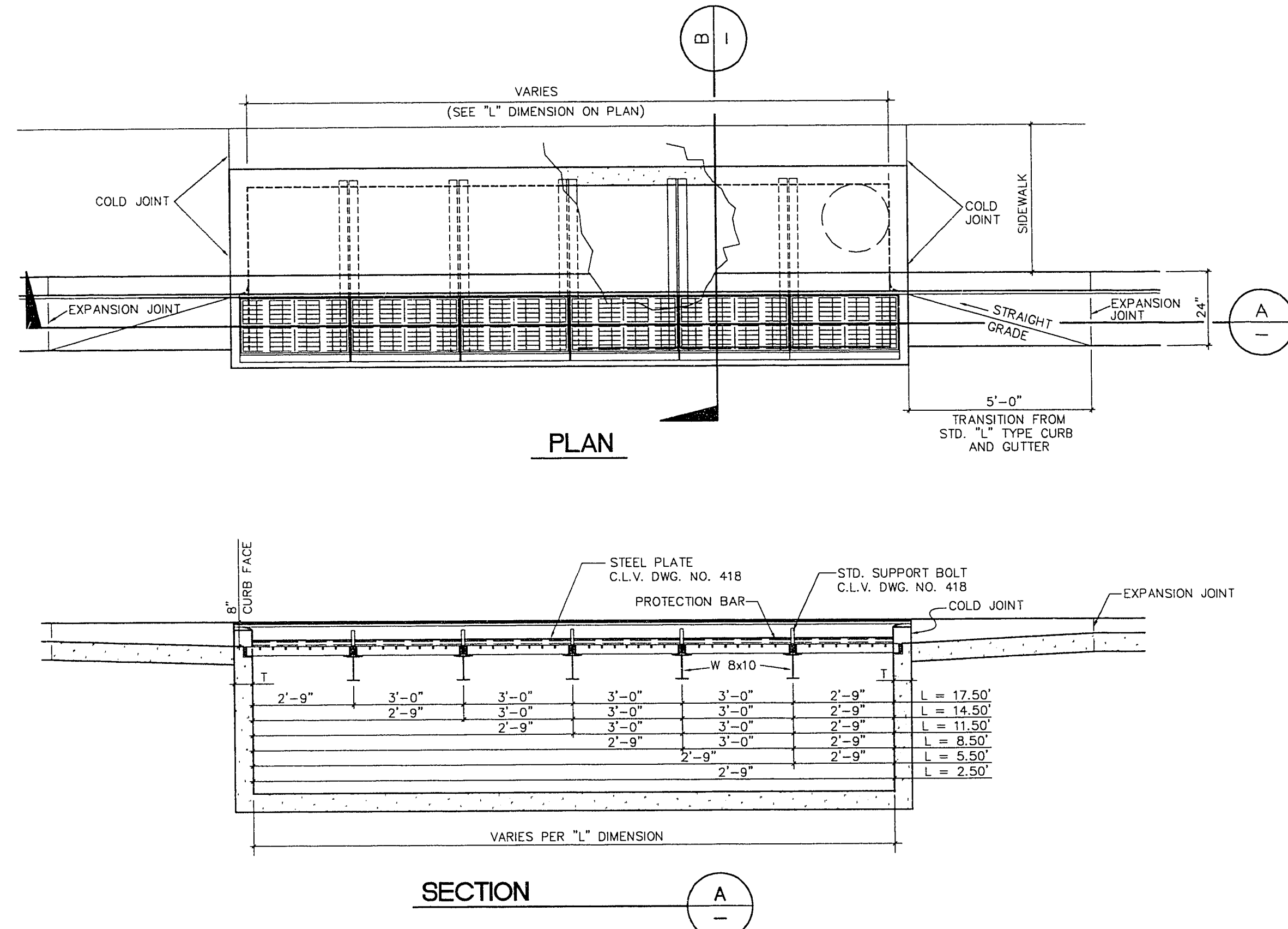
MODIFIED TYPE "C" DROP INLET NOT TO SCALE
