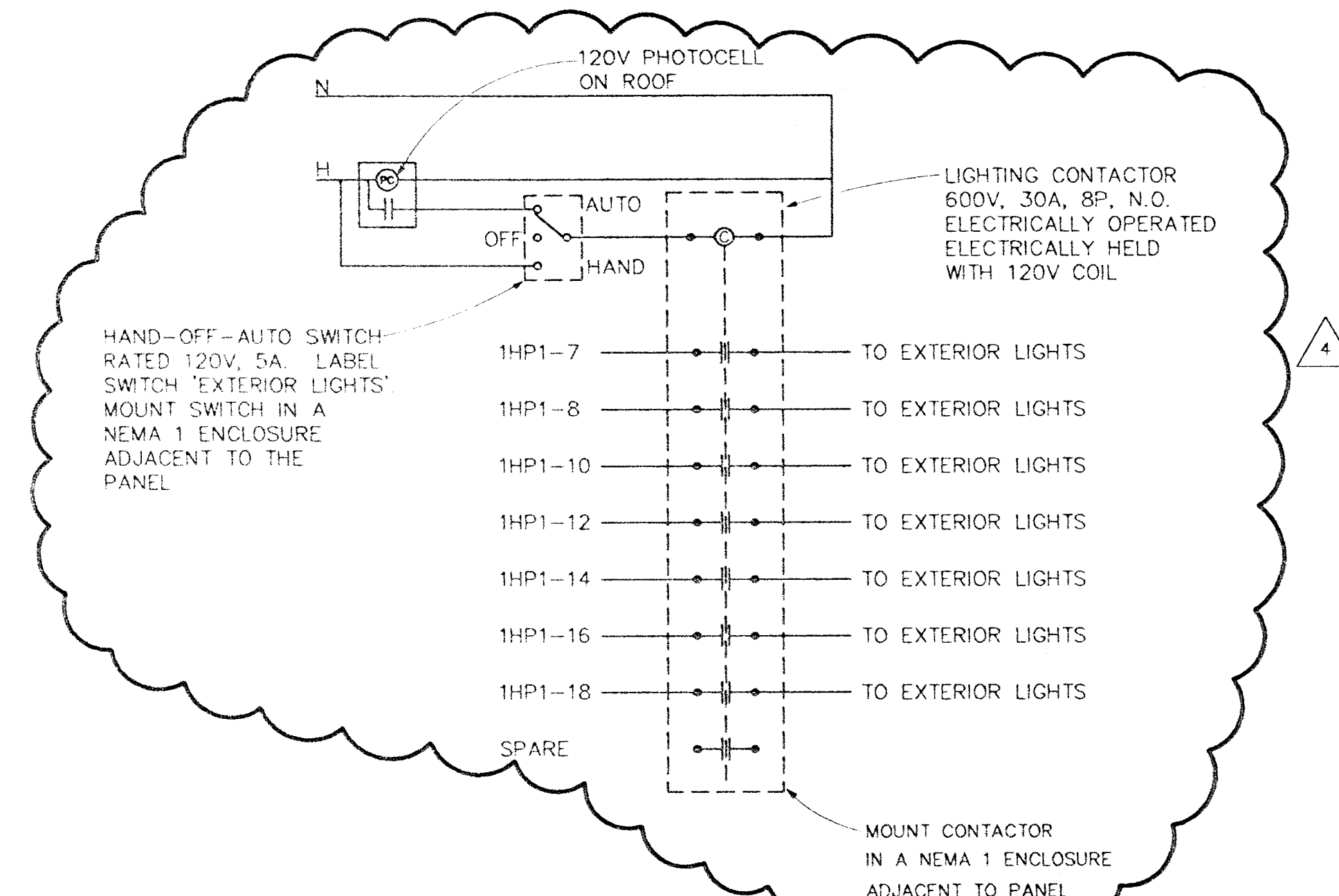
DETAIL - 4 - EXTERIOR LIGHTING CONTACTOR 'a' WIRING SCHEMATIC
