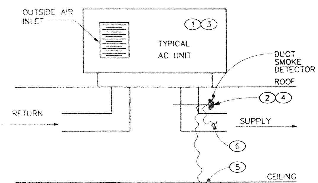
DETAIL # 1 - SMOKE DETECTOR DIAGRAM
