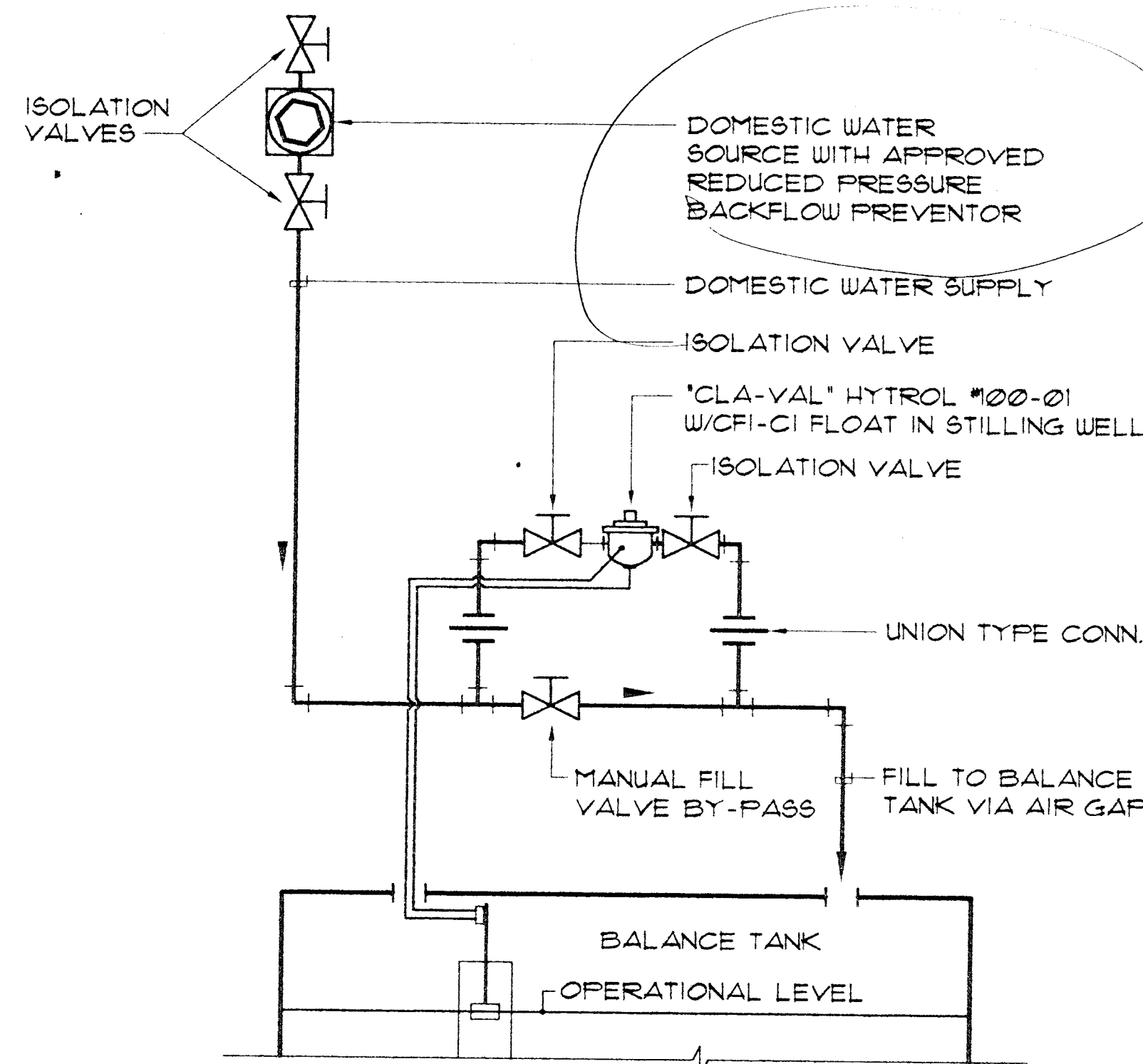
5 AUTOMATIC/MANUAL WATER MAKE-UP SCHEMATIC
