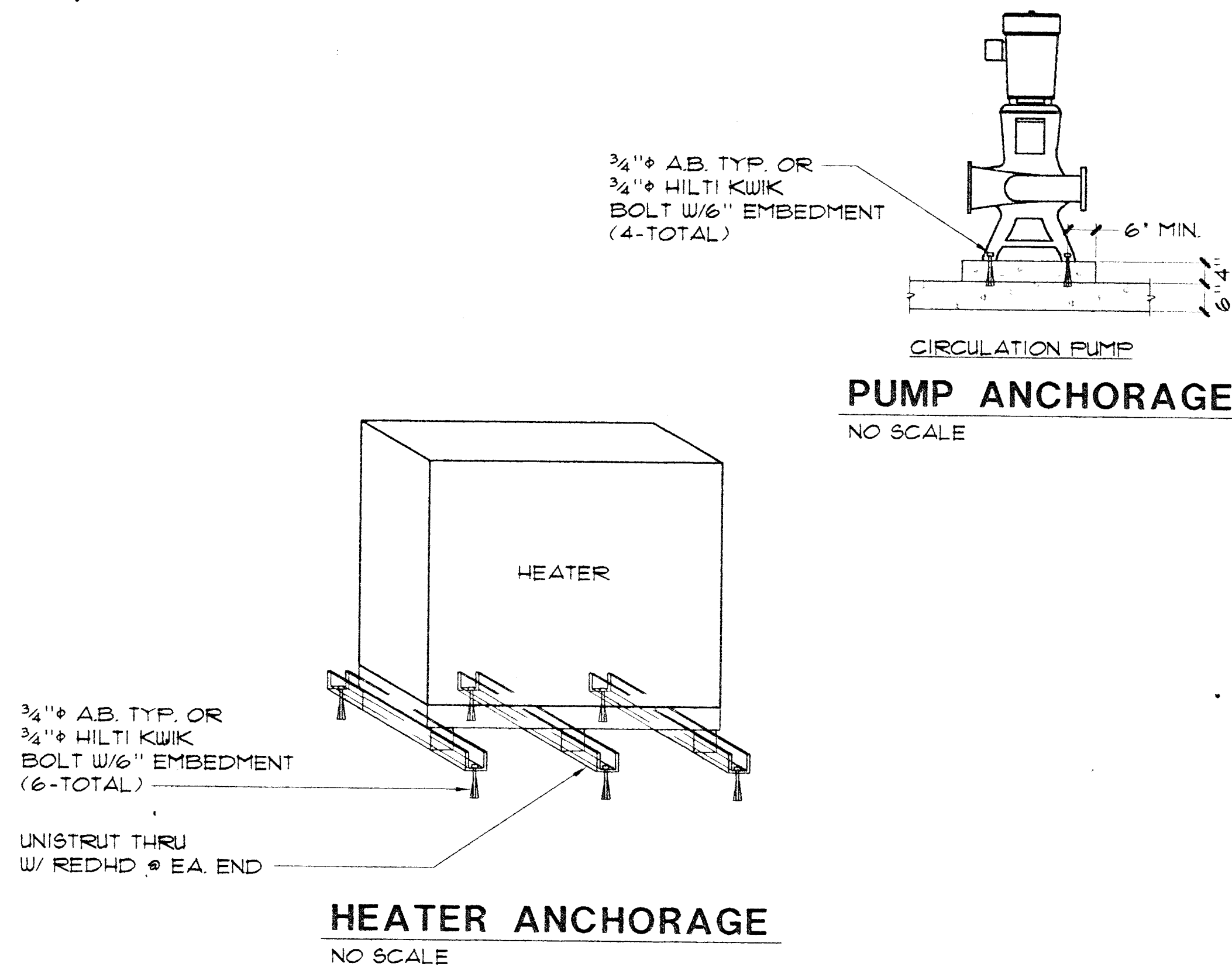
2 HEATER ANCHORAGE
