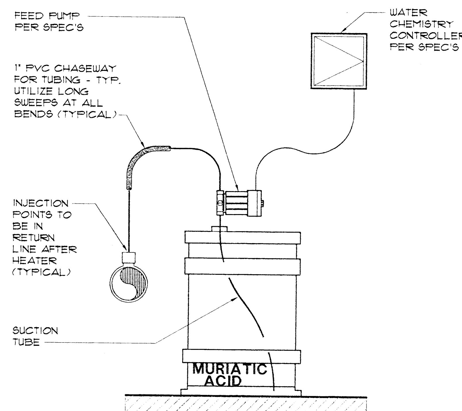
8 MURIATIC ACID FEED SCHEMATIC
