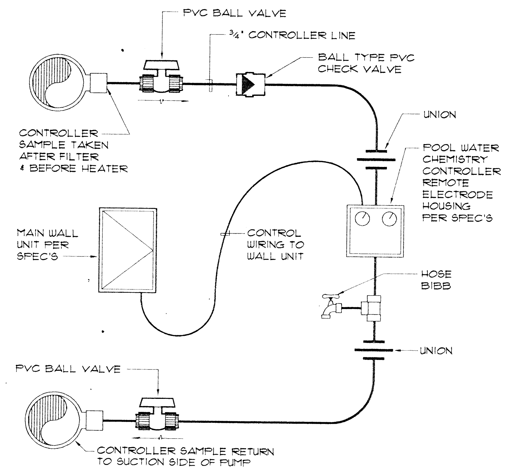
6 POOL WATER CHEMISTRY CONTROLLER
