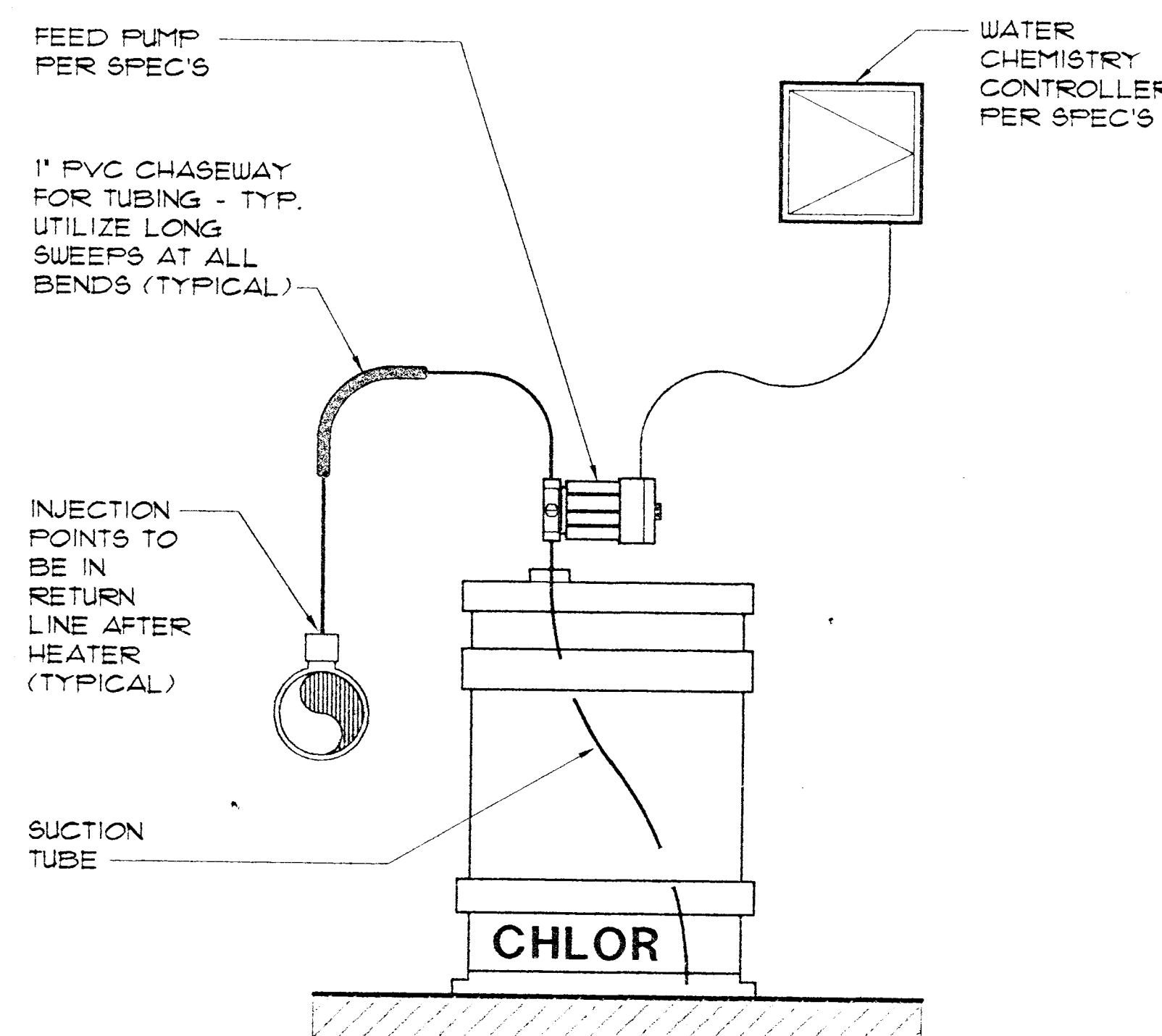
7 SODIUM HYPOCHLORITE FEED SCHEMATIC
