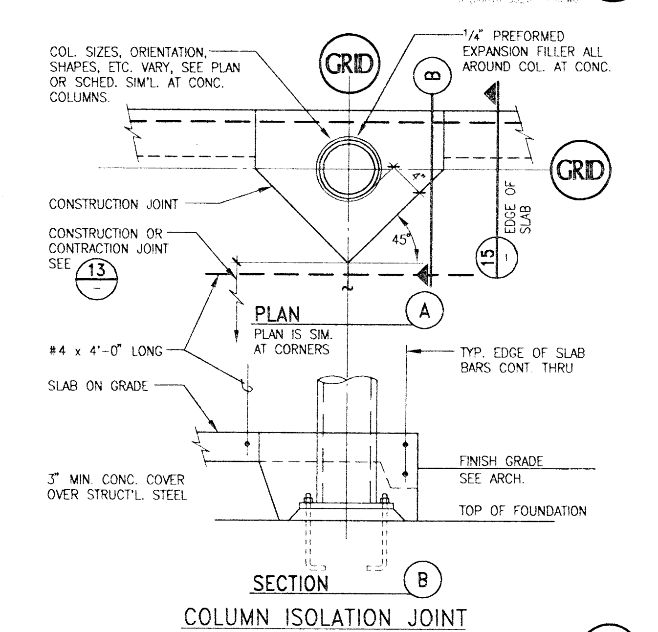
DETAIL 14 COLUMN ISOLATION JOINT
