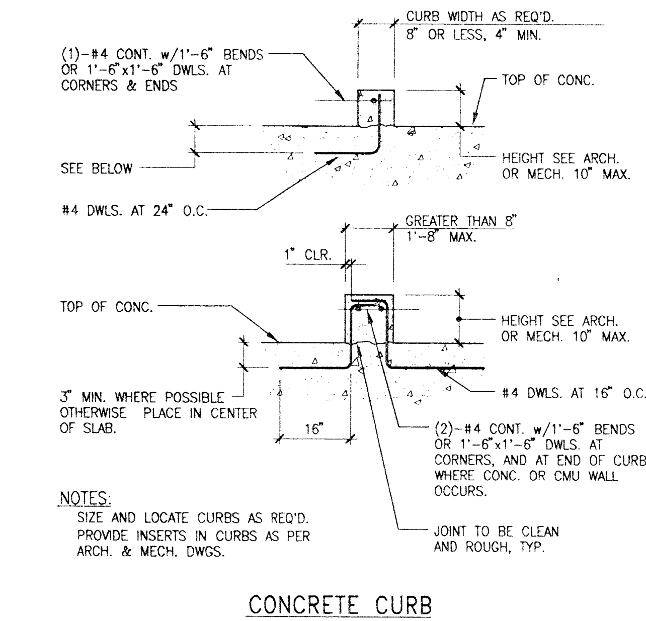
DETAIL 17 CONCRETE CURB
