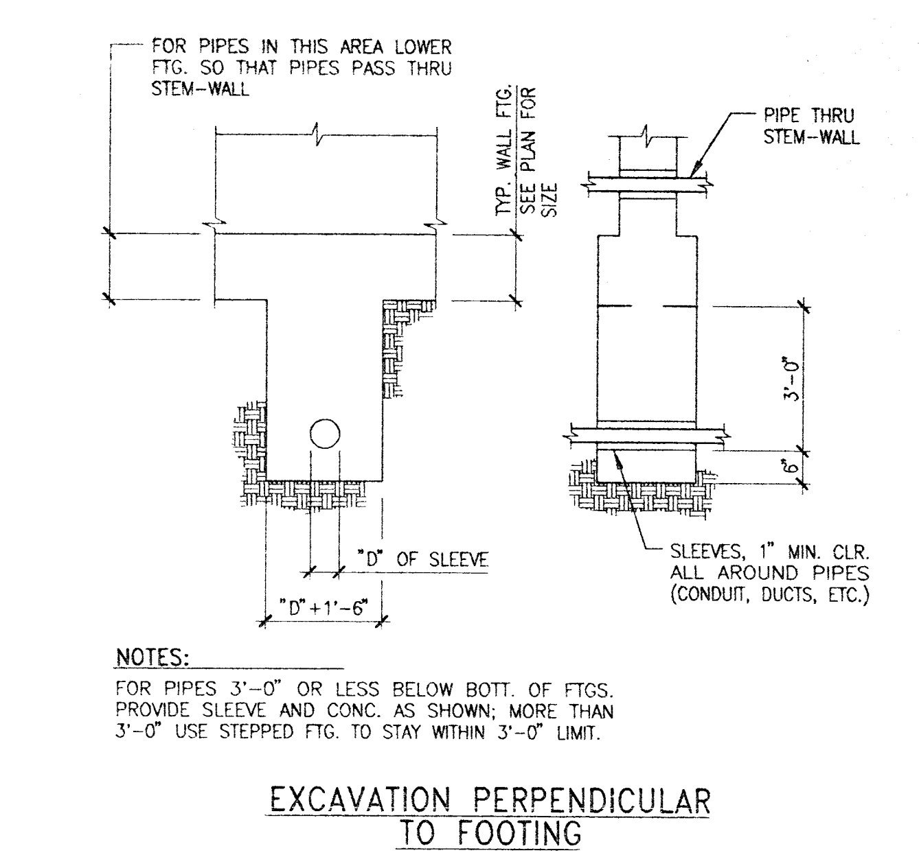
DETAIL 1 EXCAVATION PERPENDICULAR TO FOOTING
