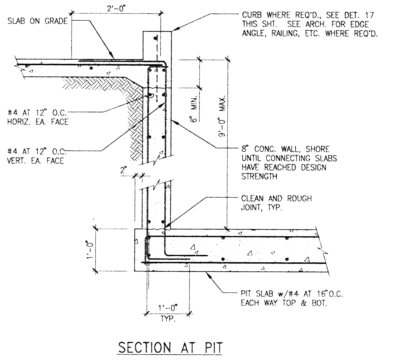
DETAIL 9 SECTION AT PIT
