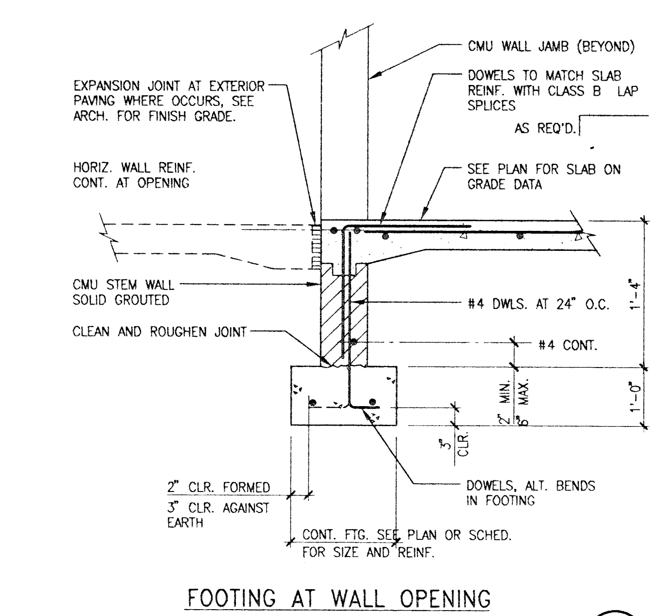
DETAIL 8 FOOTING AT WALL OPENING
