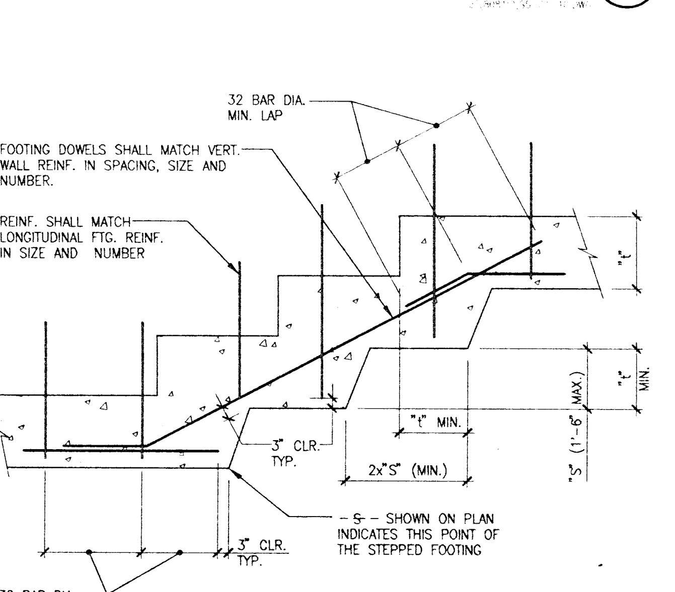
DETAIL 11 STEPPED FOOTING
