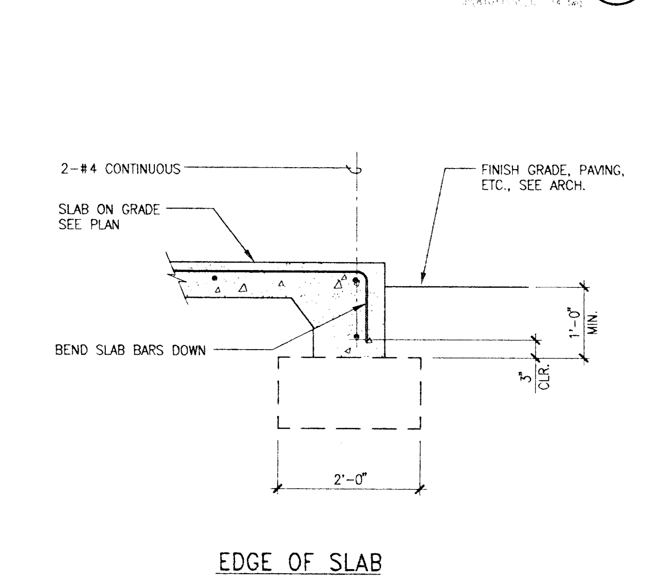
DETAIL 15 EDGE OF SLAB
