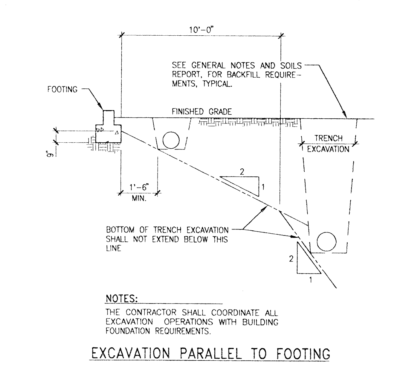
DETAIL 2 EXCAVATION PARALLEL TO FOOTING
