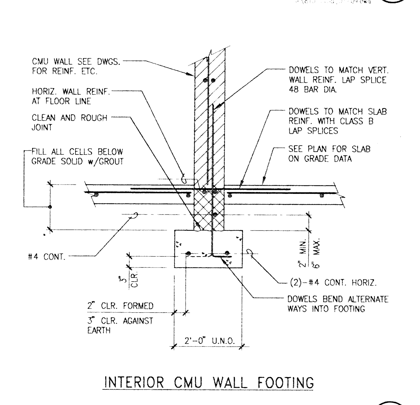
DETAIL 10 INTERIOR CMU WALL FOOTING
