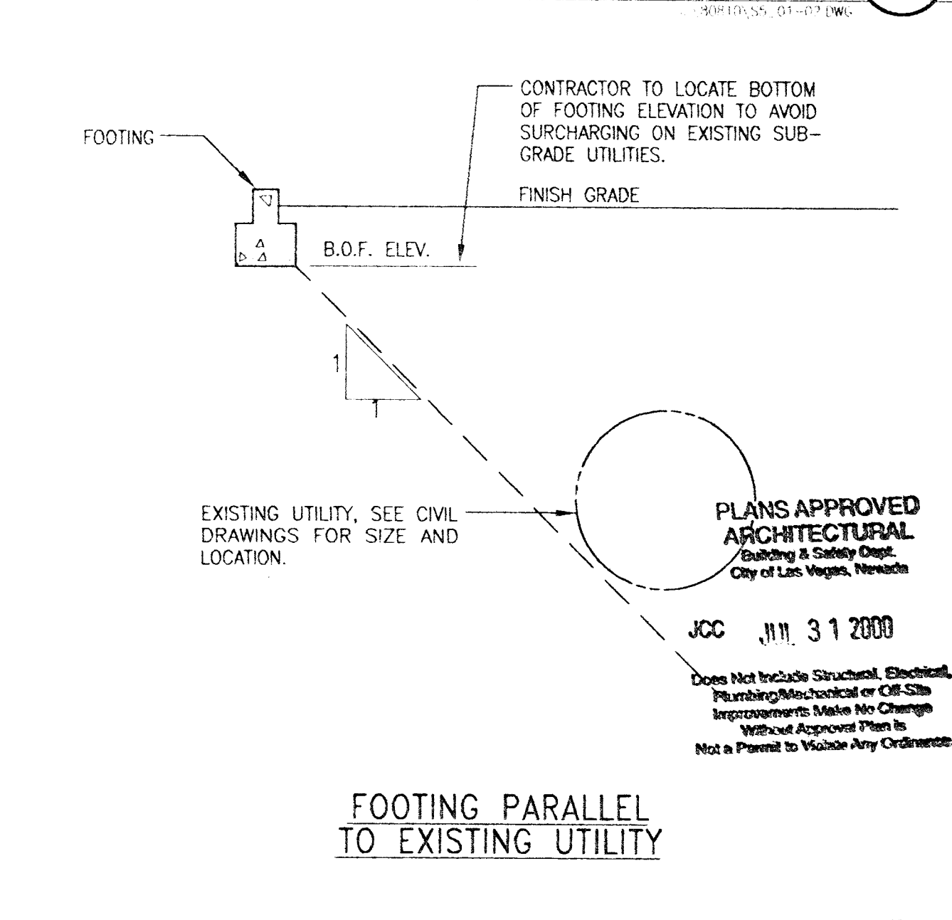
DETAIL 3 FOOTING PARALLEL TO EXISTING UTILITY
