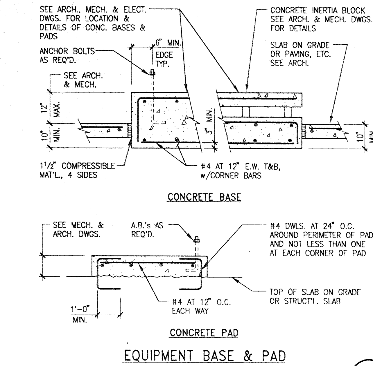
DETAIL 16 CONCRETE BASE & PAD
