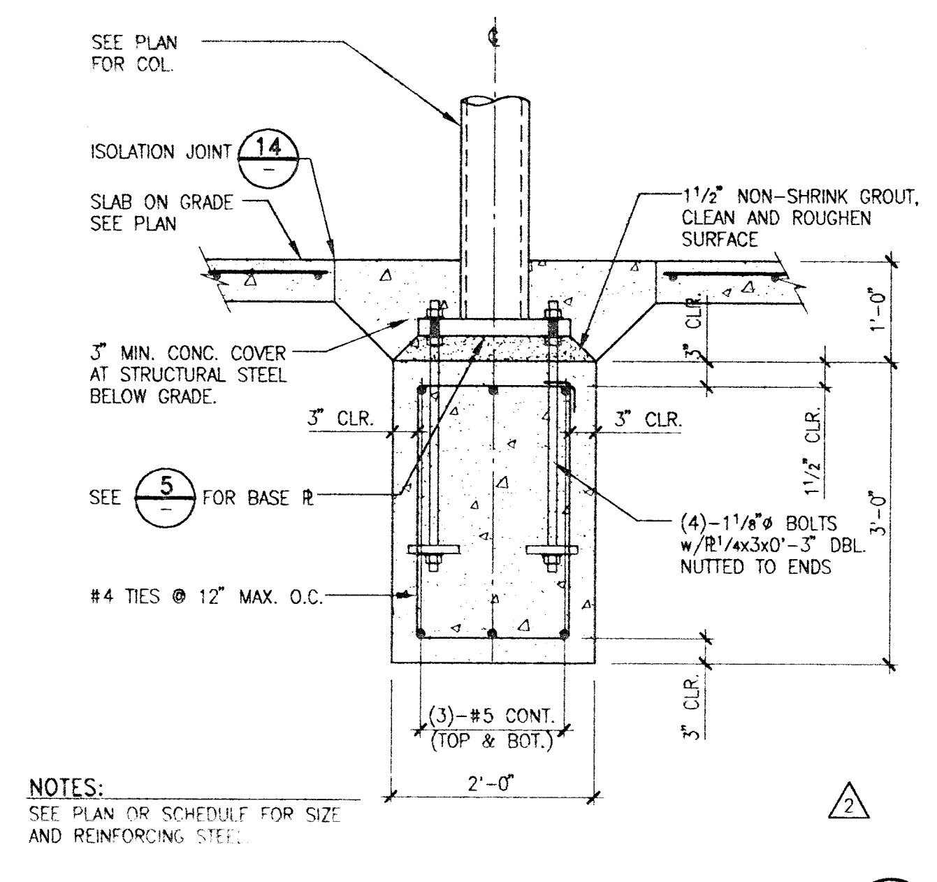
DETAIL 4 BASE PLATE DETAIL
