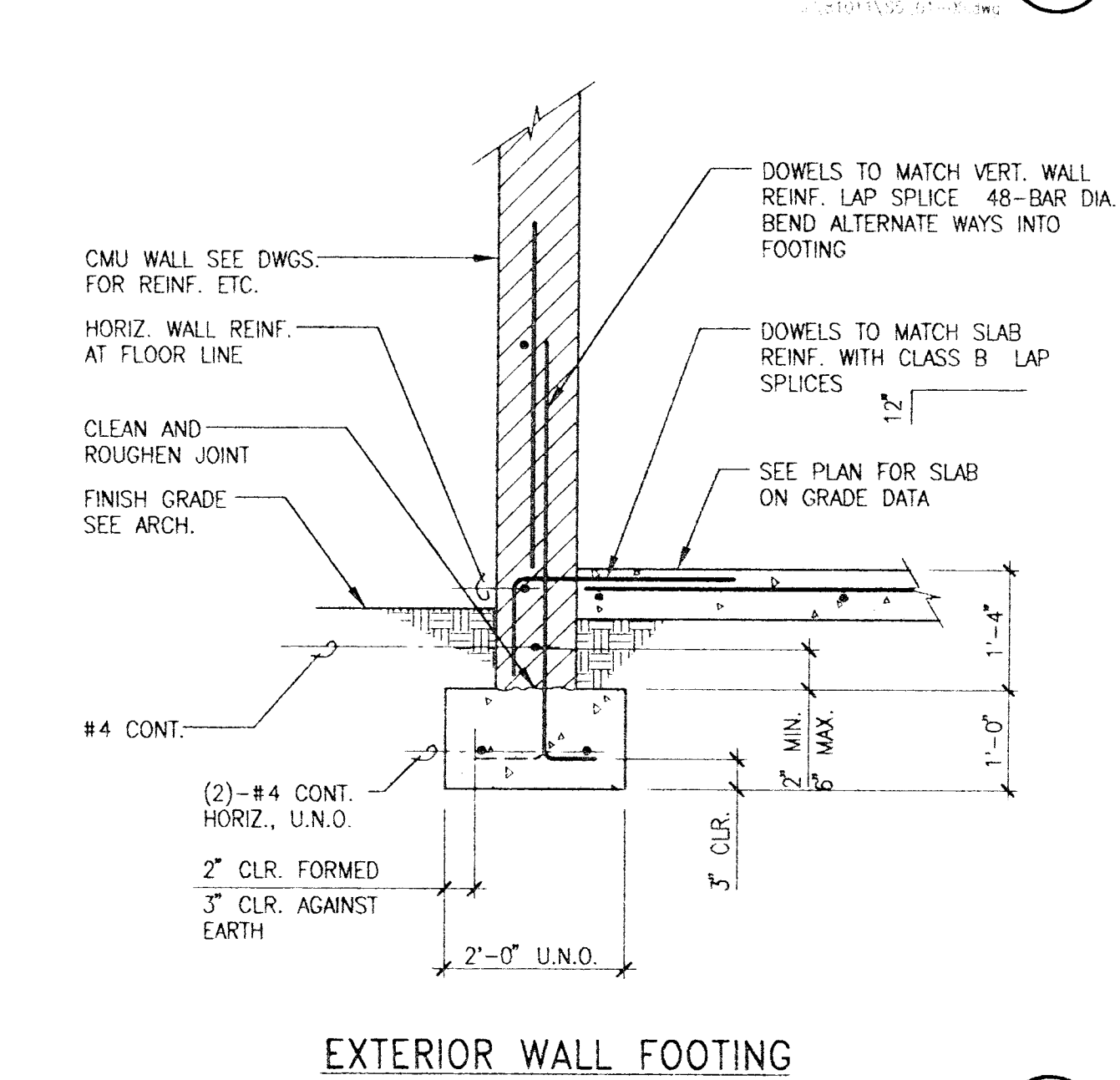
DETAIL 6 EXTERIOR WALL FOOTING
