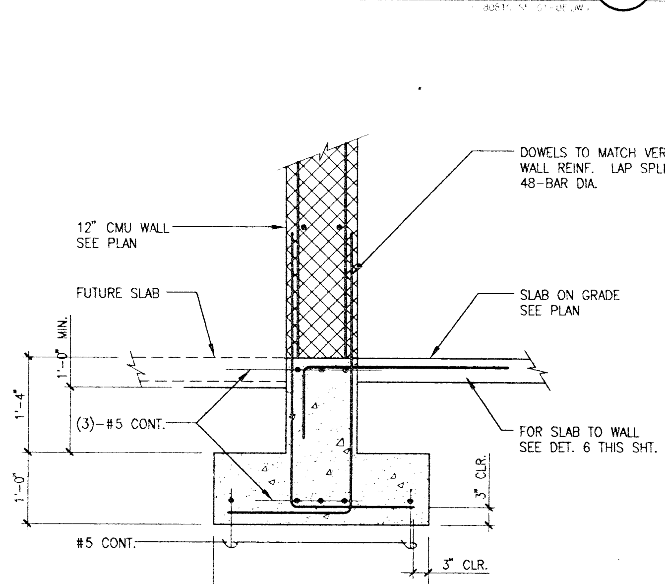
DETAIL 7 EXTERIOR WALL FOOTING
