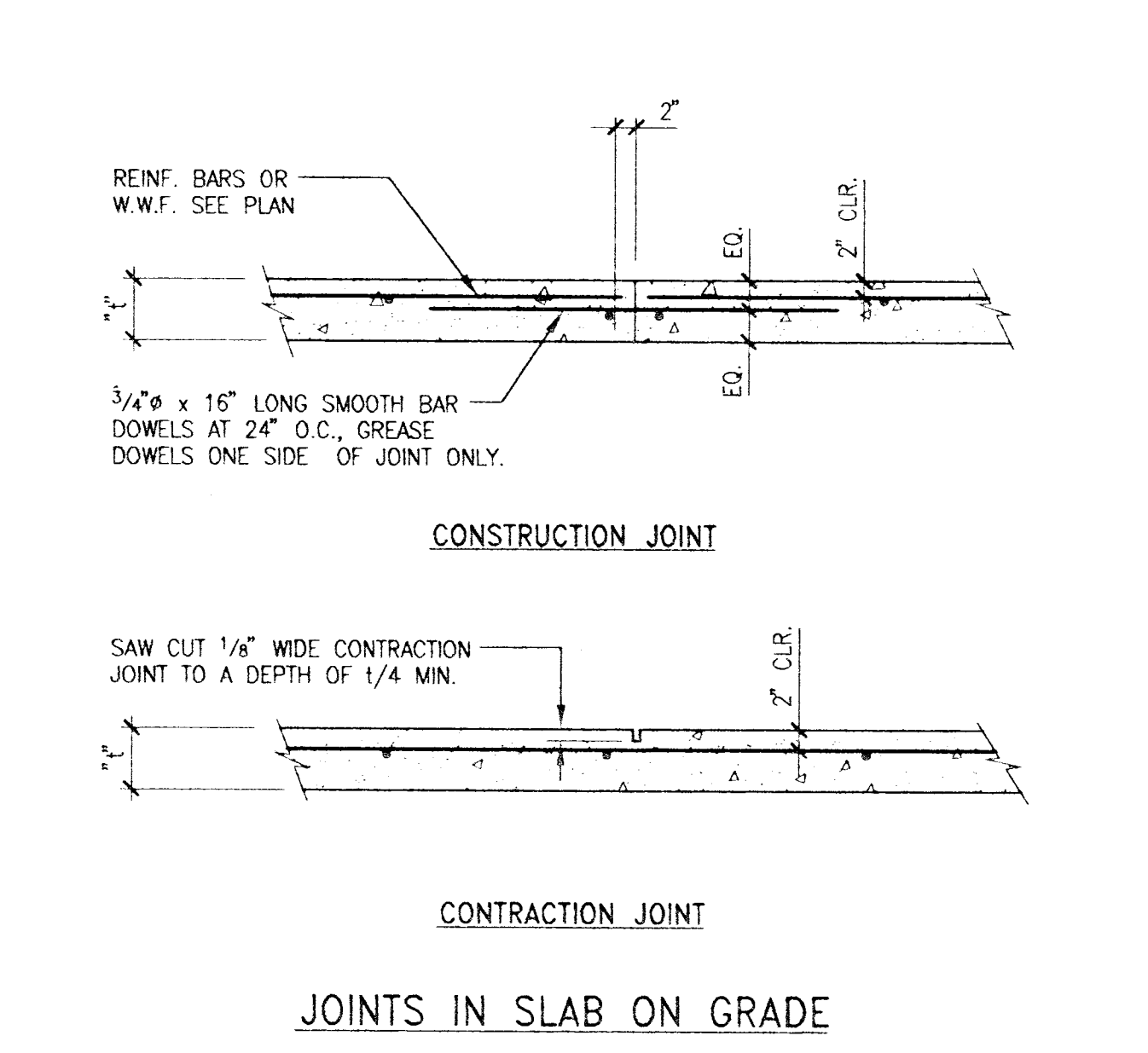
DETAIL 13 JOINTS IN SLAB ON GRADE
