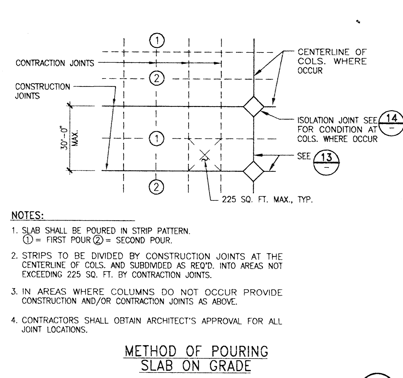
DETAIL 12 METHOD OF POURING SLAB ON GRADE
