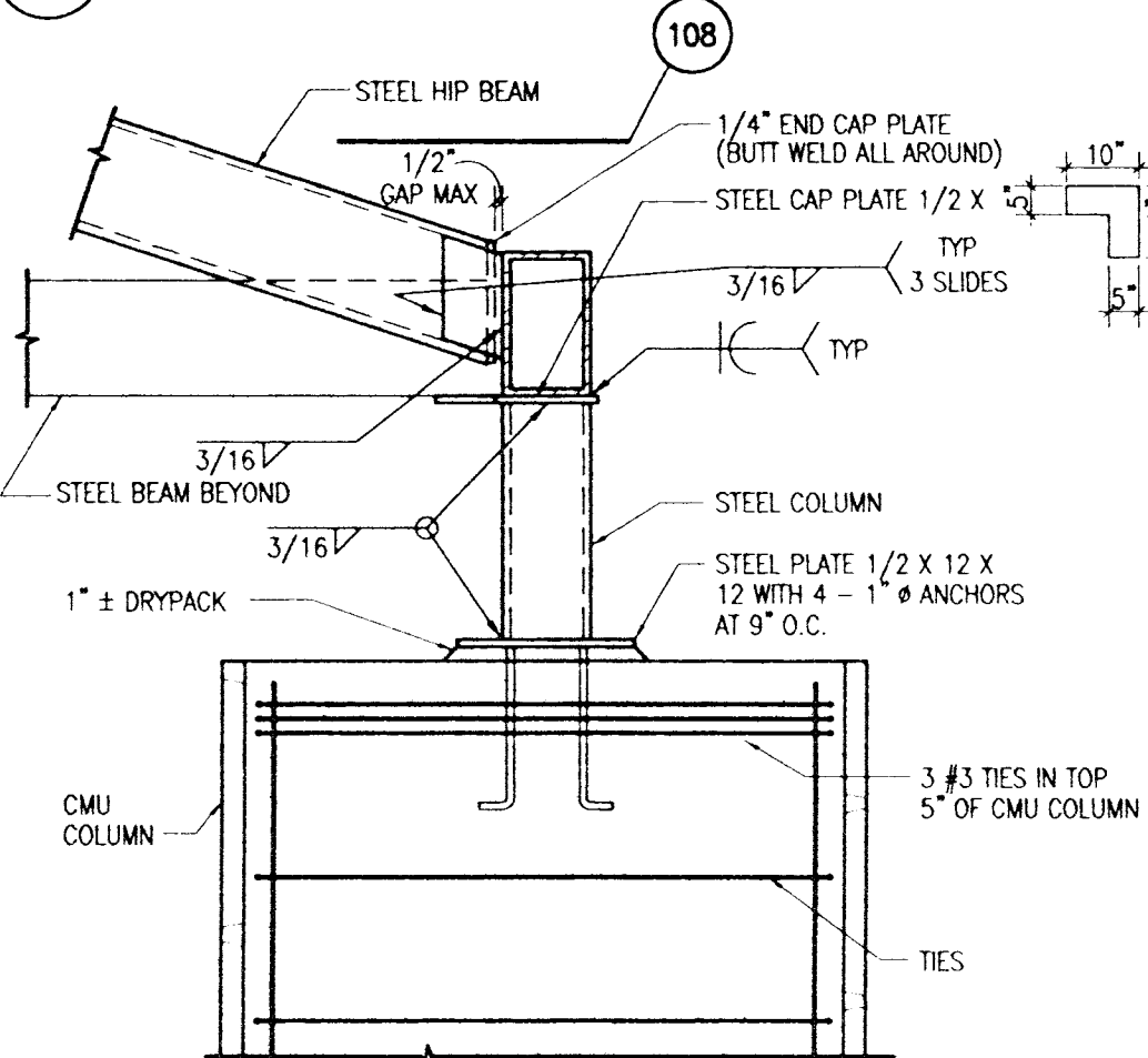
107 MULTIPLE STEEL BEAMS AT CMU COLUMN
