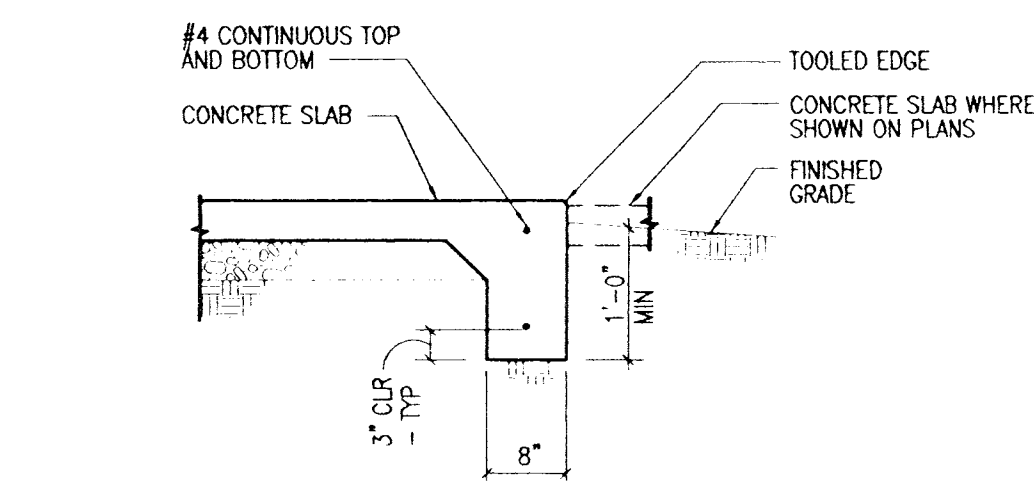
103 TYPICAL CONCRETE SLAB TOEDOWN 203.01A
