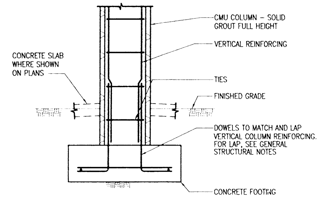
102 EXTERIOR CMU COLUMN FOOTING 271.01
