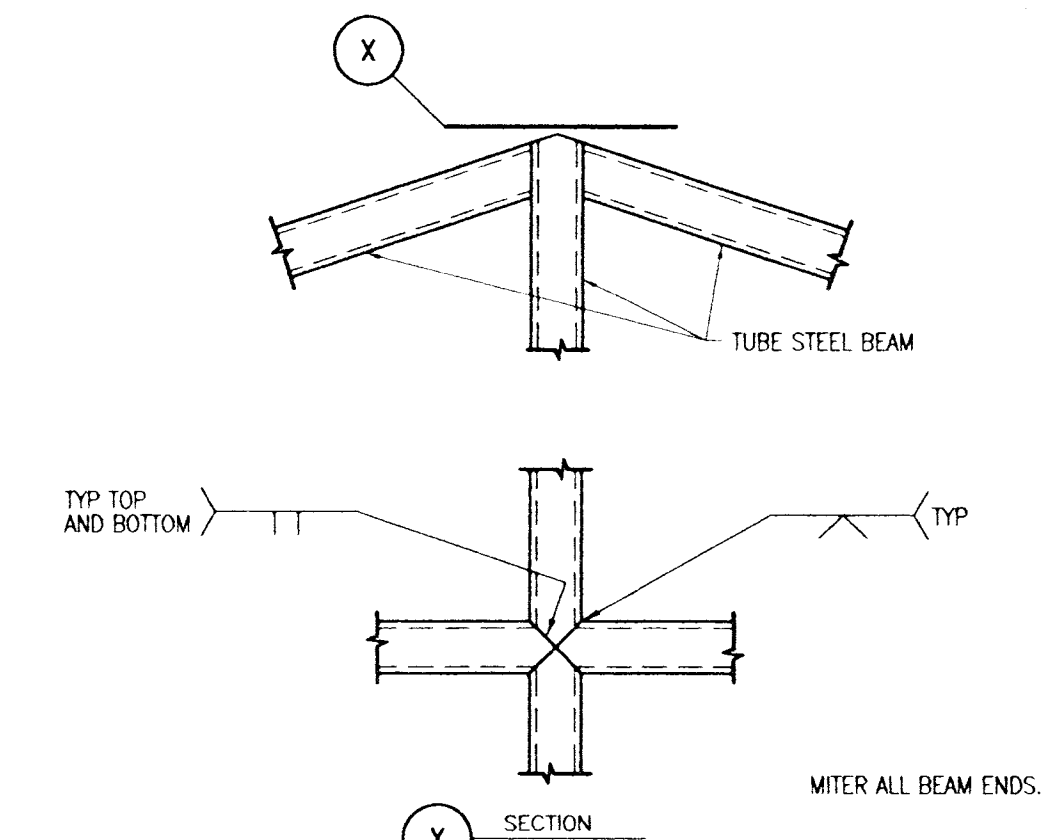
105 CONNECTION OF ROOF MITERED BEAMS
