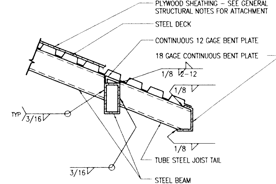
104 STEEL BEAM TO STEEL BEAM CONNECTION
