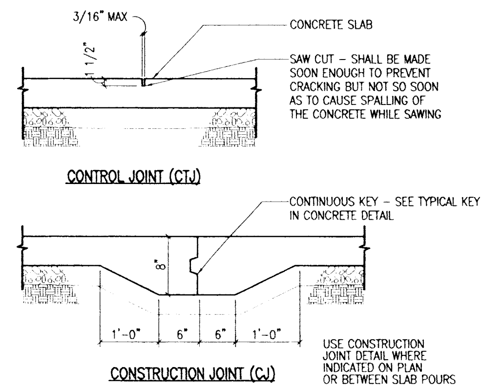
101 TYPICAL CONCRETE SLAB JOINTS 202.01
