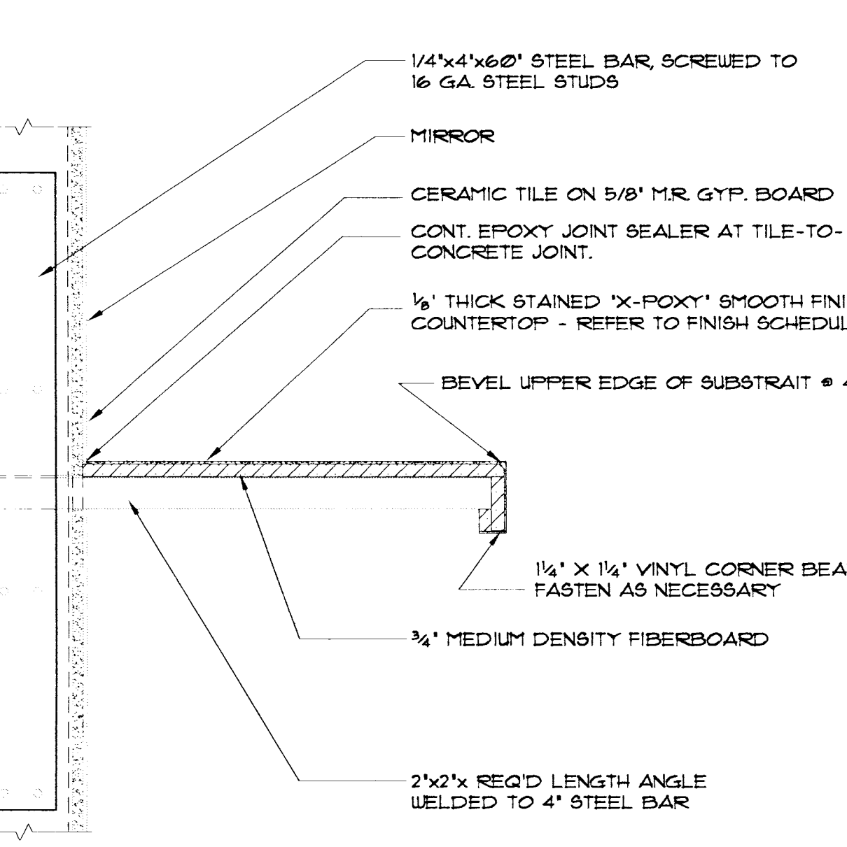
LAVATORY/COUNTER TOP SCALE: 1/2" = 1'-0"
