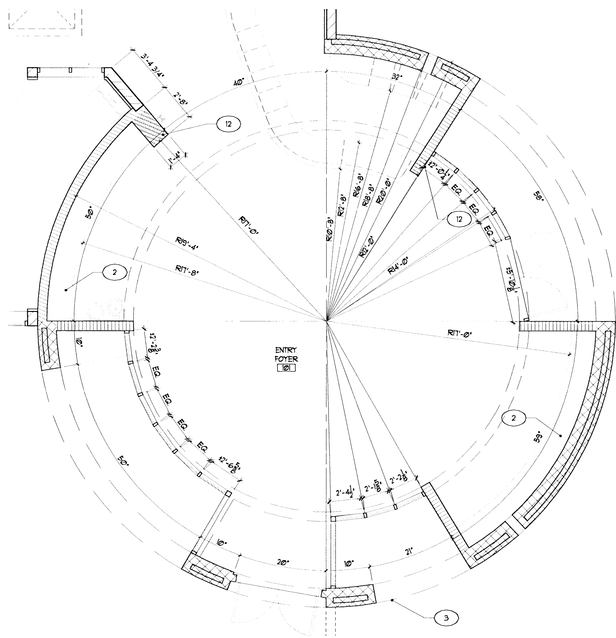
ENTRY FOYER PLAN SCALE: 1/4" = 1'-0"
