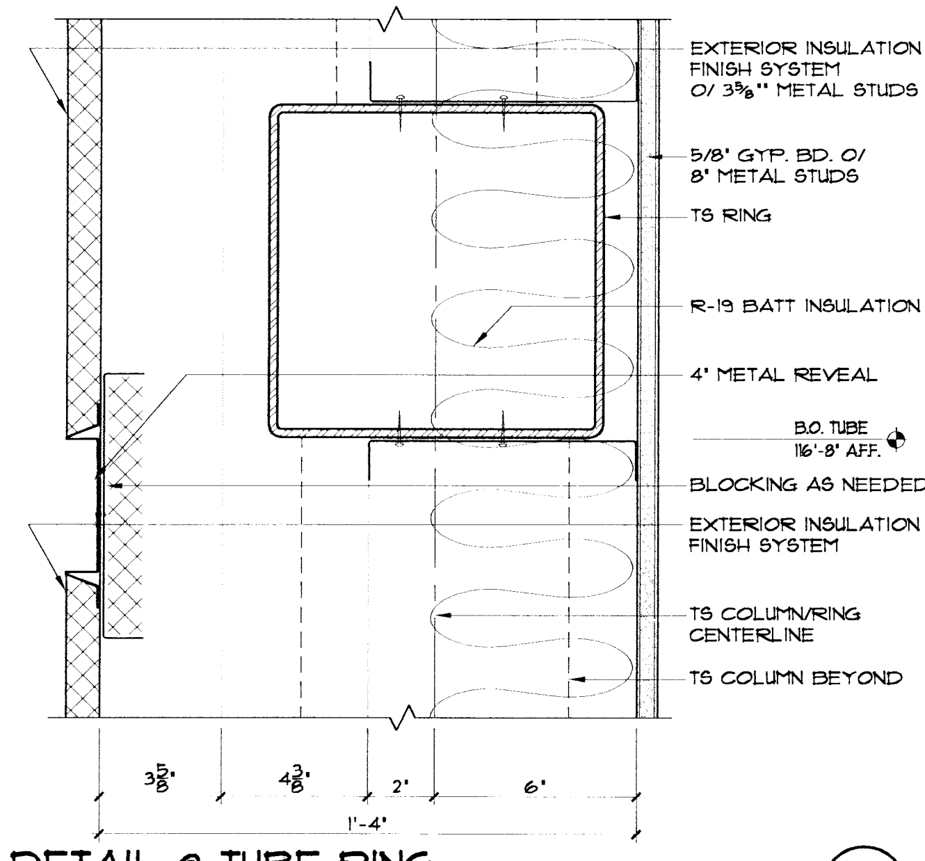
DETAIL @ TUBE RING SCALE: 3" = 1'-0"
