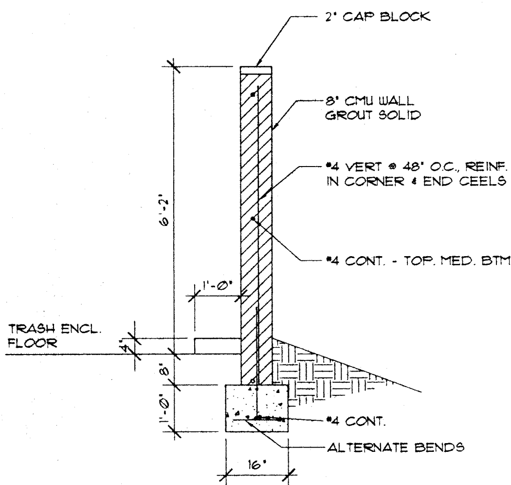
DUMPSTER ENCLOSURE SECTION
