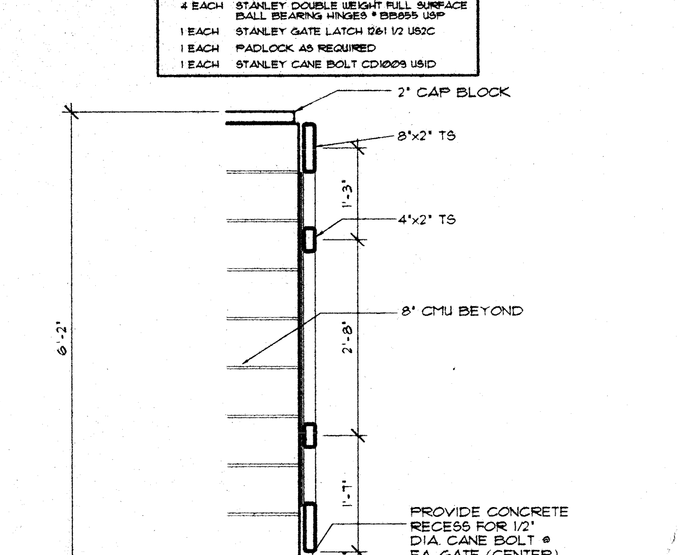
DUMPSTER SECTION
