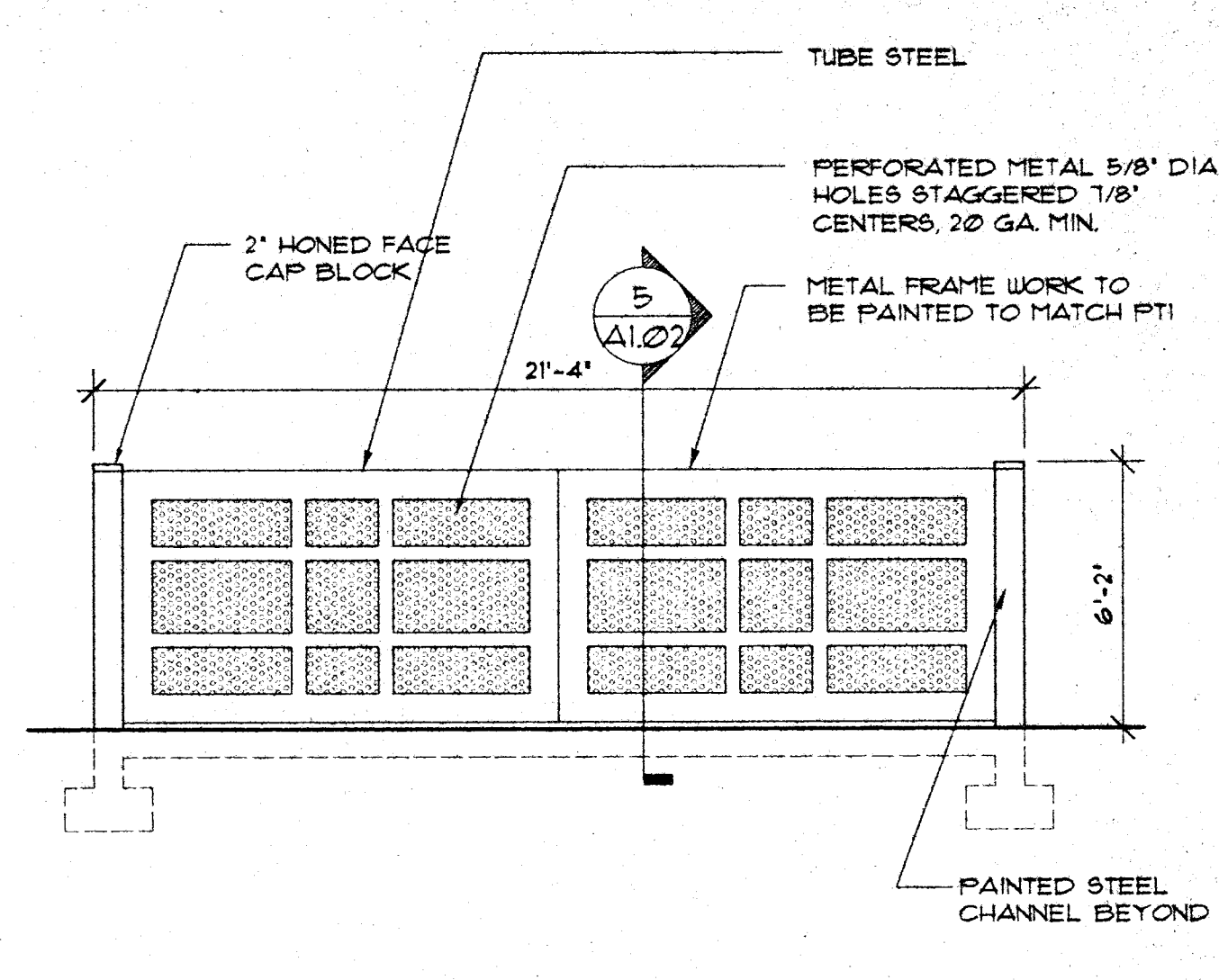
DUMPSTER ELEVATION
