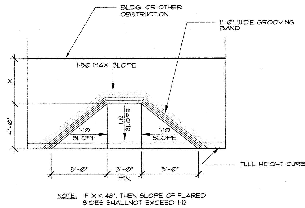
WHEEL CHAIR RAMP PLAN
