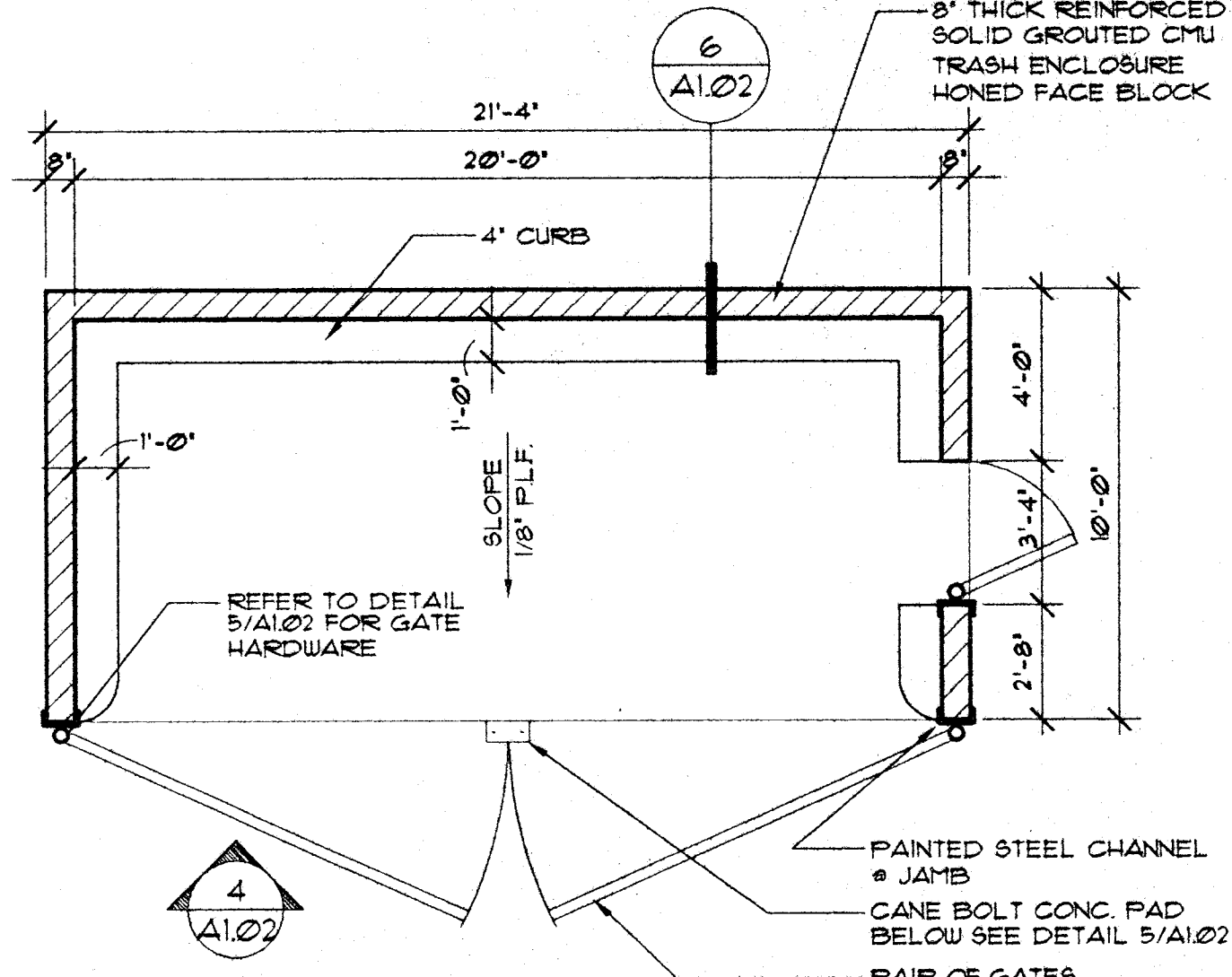
DUMPSTER ENCLOSURE
