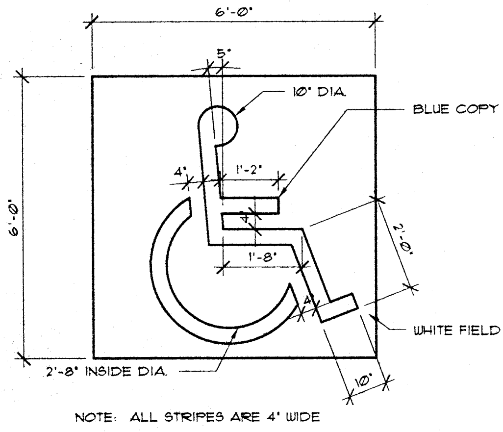
SYMBOL OF ACCESSIBILITY
