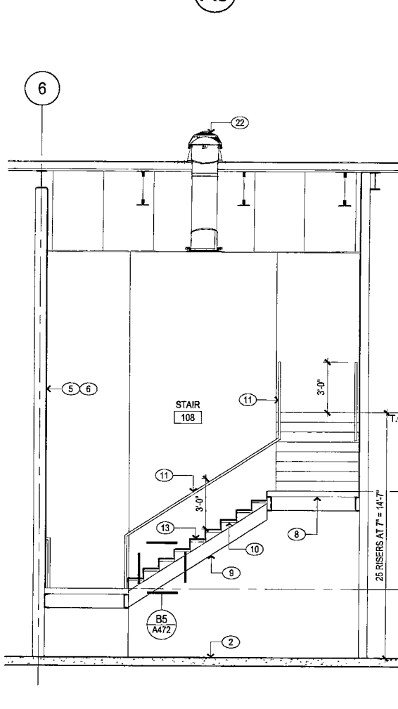
C2 STAIR SECTION
