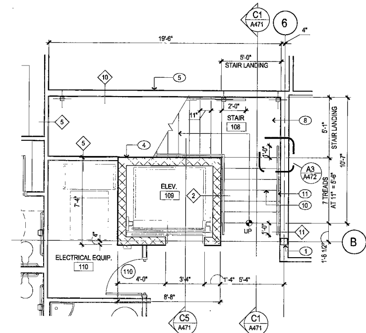
A1 STAIR AND ELEVATOR PLAN
