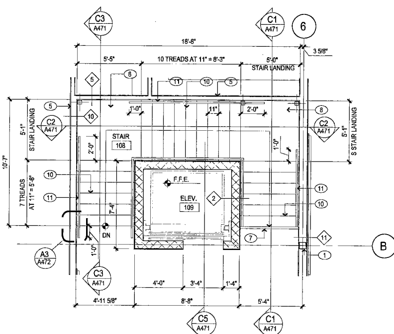
A3 STAIR AND ELEVATOR PLAN
