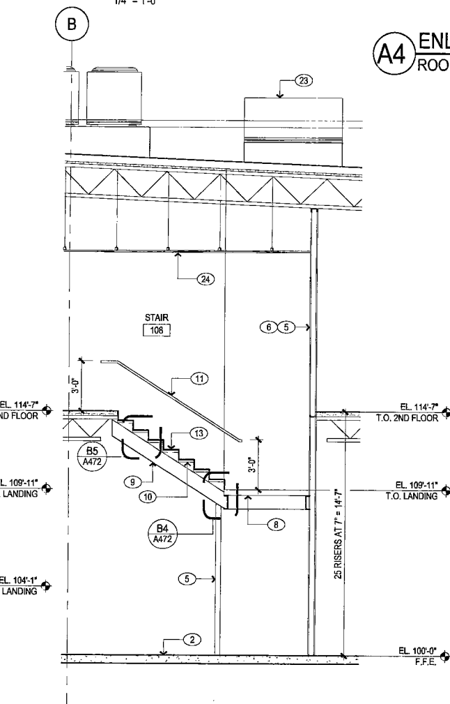
C3 STAIR SECTION
