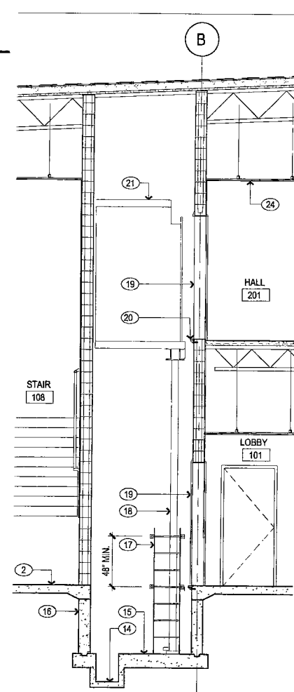
C5 ELEVATOR SECTION
