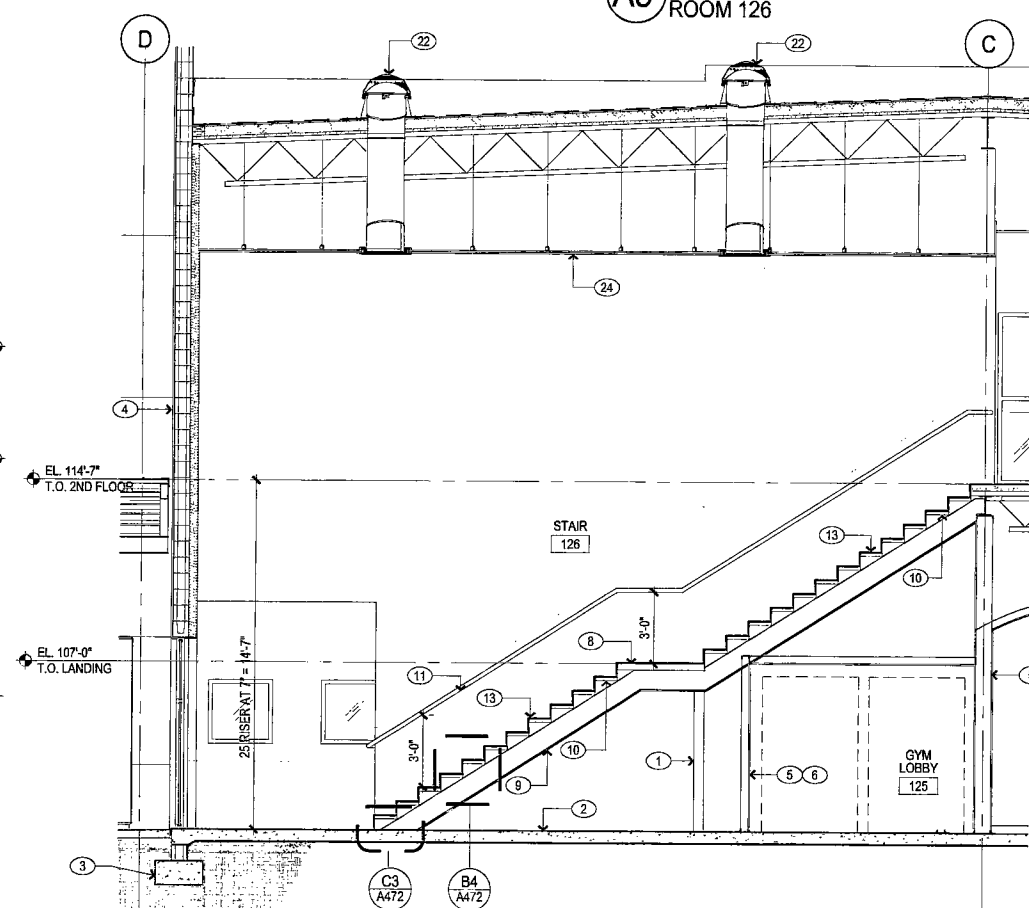
C4 STAIR SECTION
