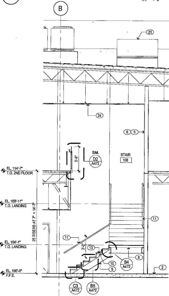
C1 STAIR SECTION
