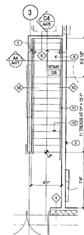
A4 ENLARGED STAIR PLAN ROOM 126
