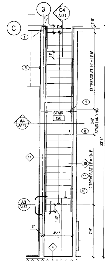
A5 ENLARGED STAIR PLAN ROOM 126
