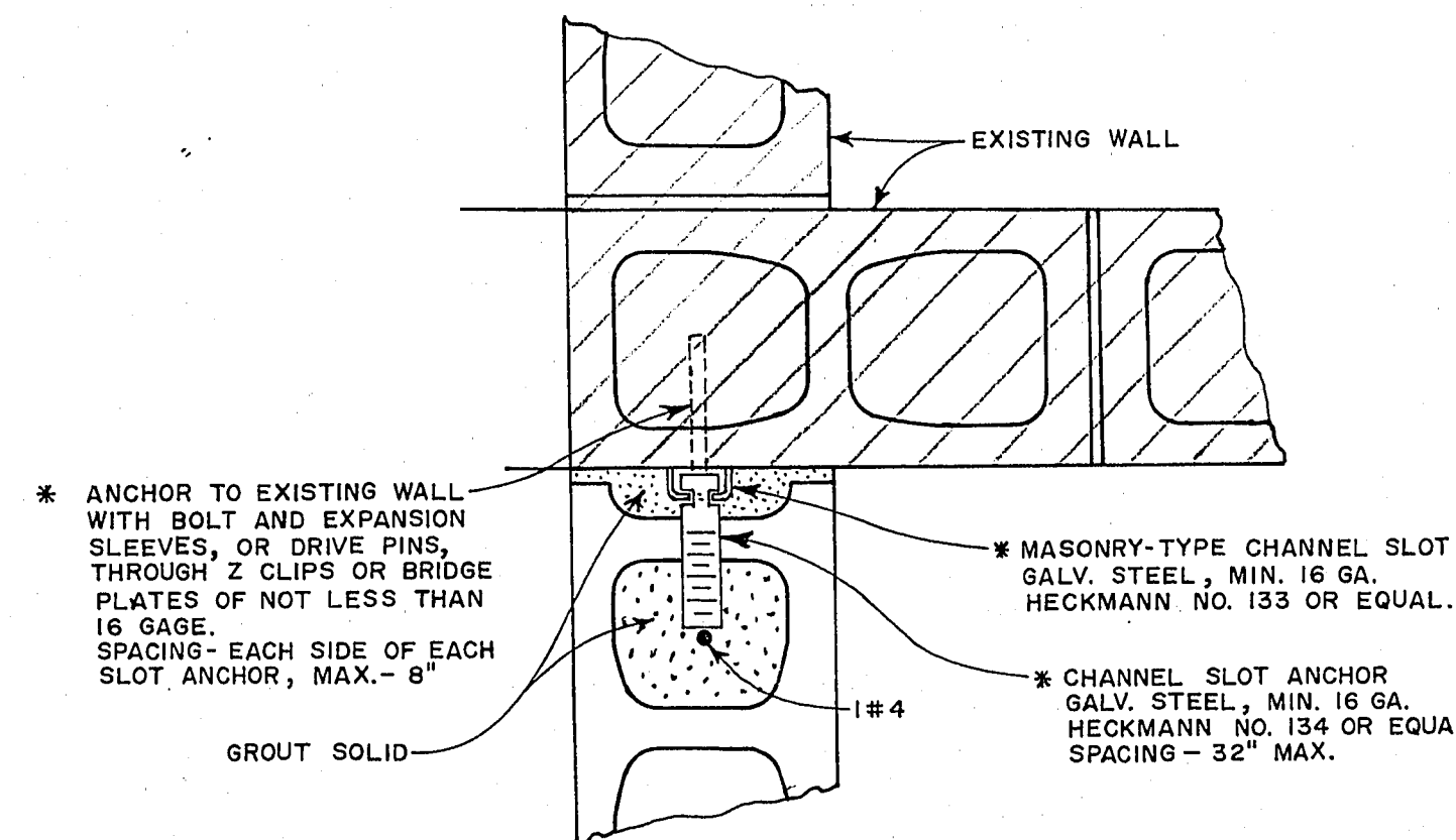
WALL TIE-IN DETAIL SCALE: 2" = 1'-0"
