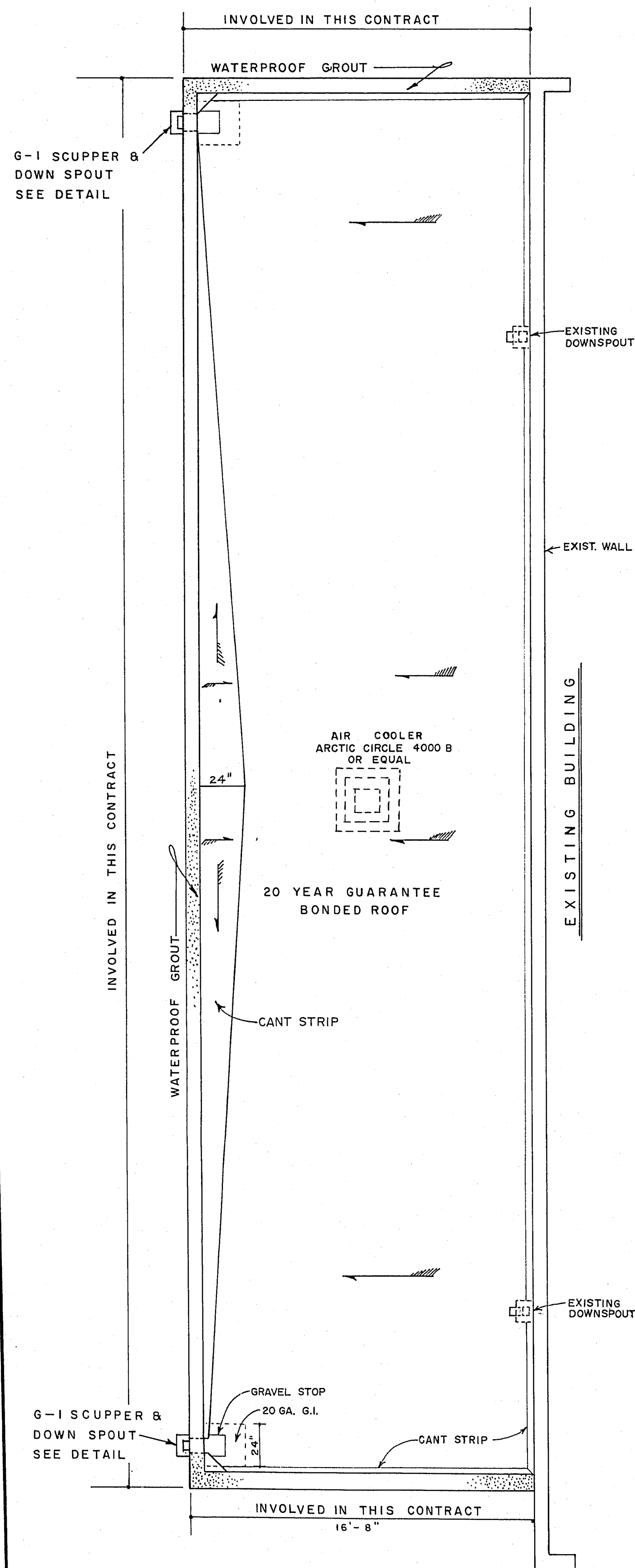
ROOF PLAN SCALE: 1/4" = 1'-0"
