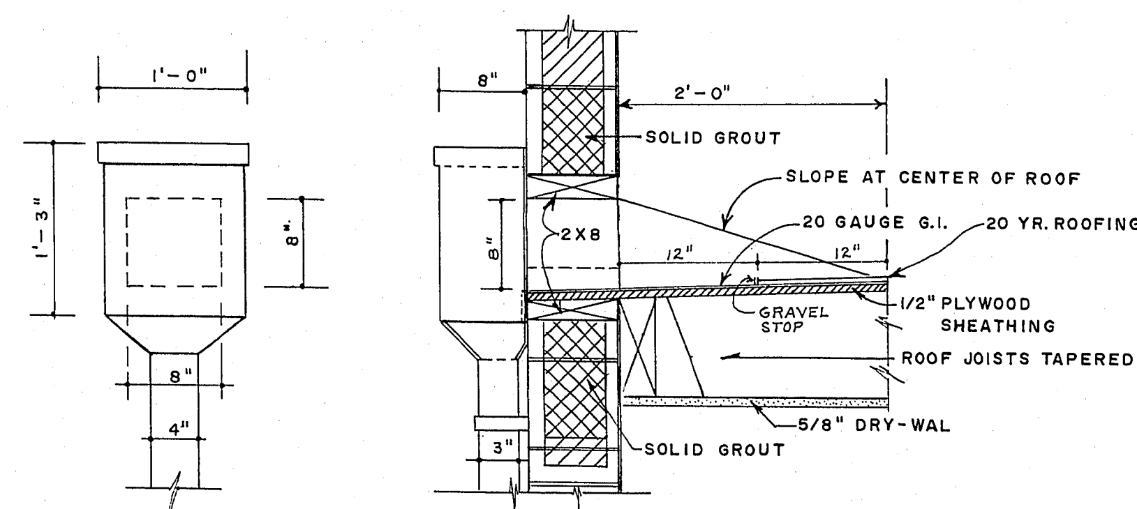
SCUPPER & DOWNSPOUT DETAIL SCALE: 1" = 1'-0"
