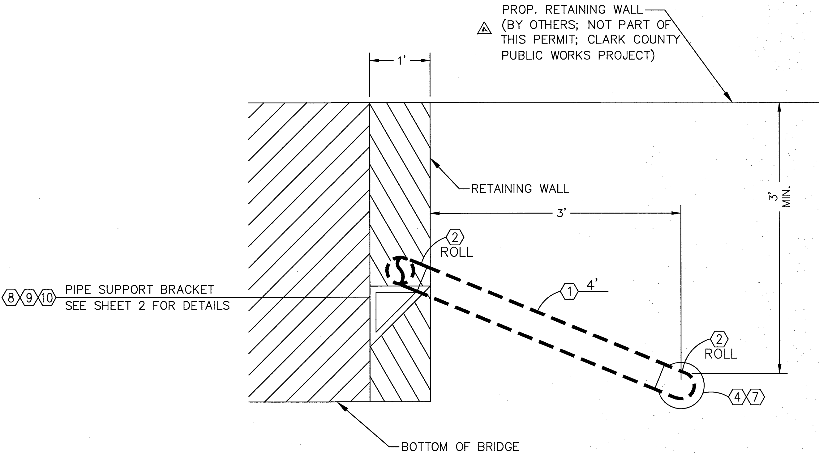
C CROSS SECTION - LOOKING WEST N.T.S.
