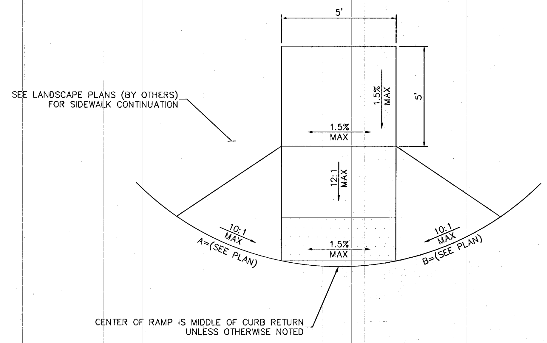
SIDEWALK RAMP DETAIL NOT TO SCALE
