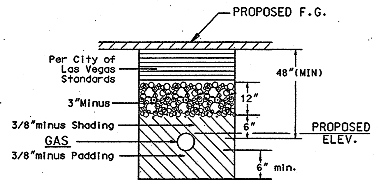
TRENCH DETAIL FOR UNIMPROVED AREAS ONLY CLV
