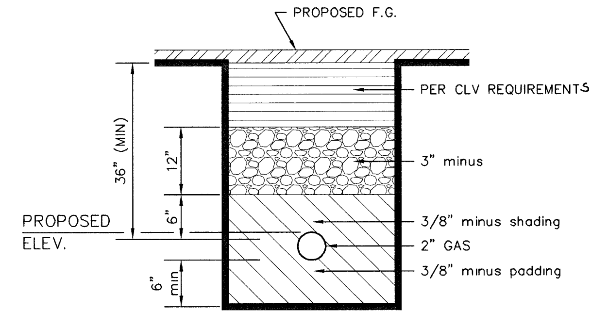
TRENCH DETAIL
