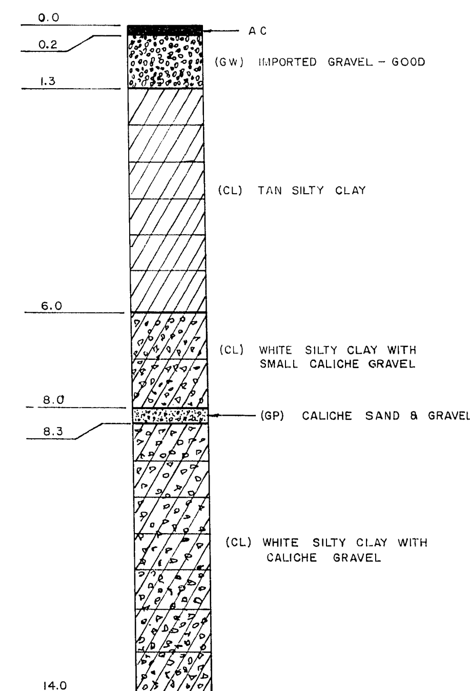
TEST HOLE NO.6 (Sandhill Rd.) STA. 90+78.82 (STA. C 65+00) HOLE ON SEC. LINE
