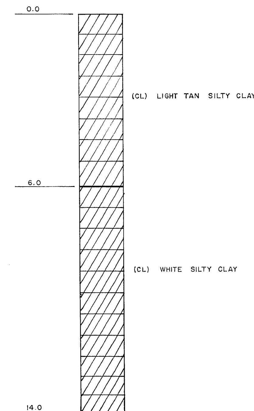
TEST HOLE NO.9 (Charleston Blvd.) STA. C97+00 HOLE 35' SOUTH OF SEC. LINE
