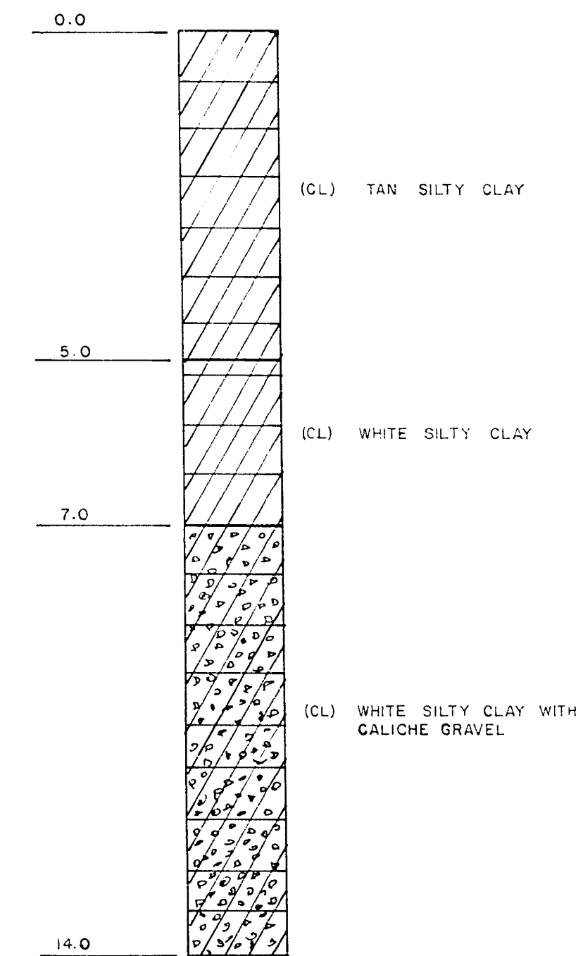
TEST HOLE NO.5 (Sandhill Rd.) STA. 78+78.82 (STA. C53+00) HOLE ON SEC. LINE
