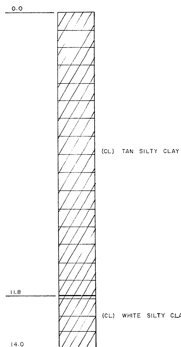
TEST HOLE NO.2 (Sandhill Rd.) STA. 41+78.82 (STA. C16+00) HOLE ON SEC. LINE
