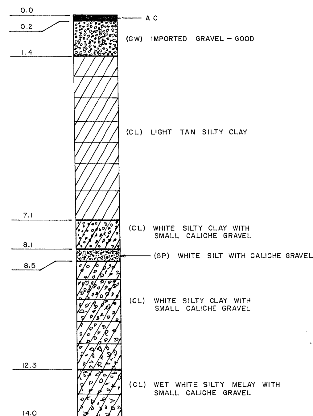
TEST HOLE NO.7 (Del Amo Dr.) STA. C 77+00 HOLE 19' WEST OF CENTER LINE
