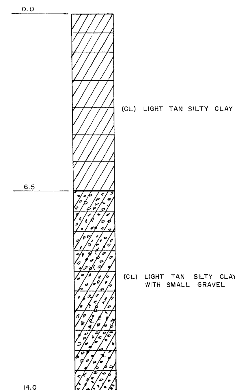
TEST HOLE NO.8 (Charleston Blvd.) STA. C85+00 HOLE 35' SOUTH OF SEC. LINE
