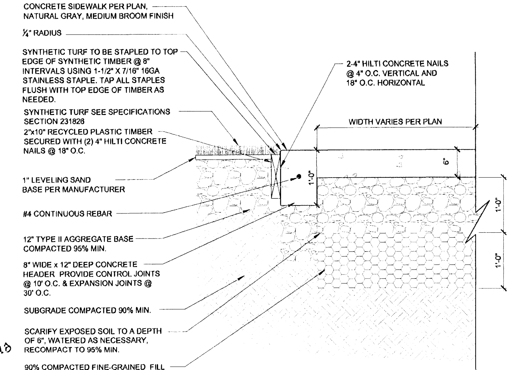
4 SYNTHETIC TURF (@ CONC. WALKWAY) SCALE: 1" = 1'-0"
