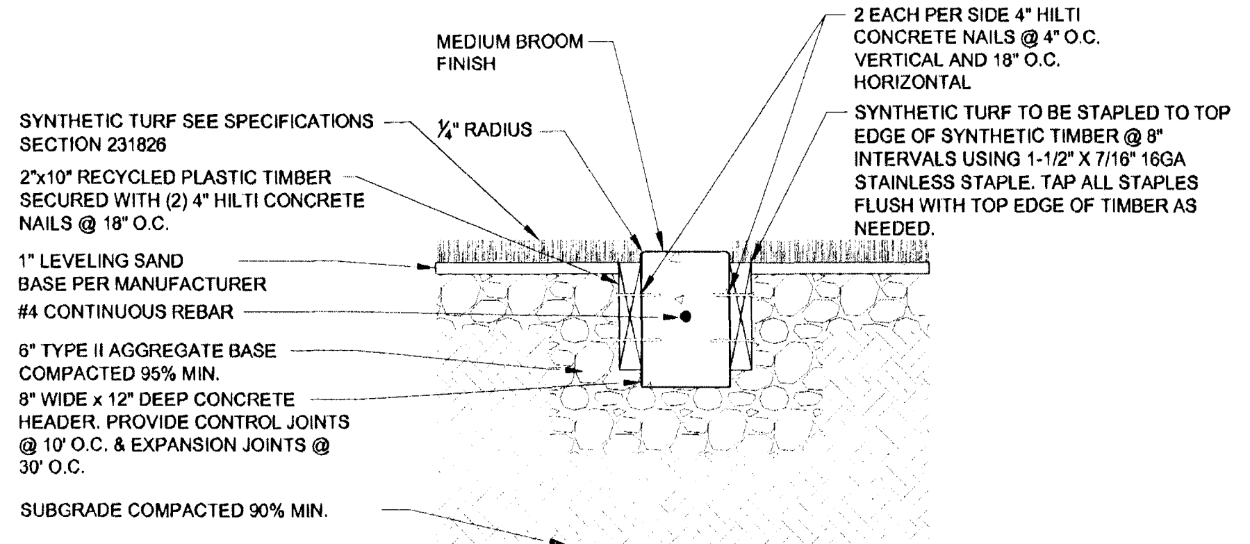
2 SYNTHETIC TURF (BOTH SIDES OF CONC. HEADER) SCALE: 1/4" = 1'-0"
