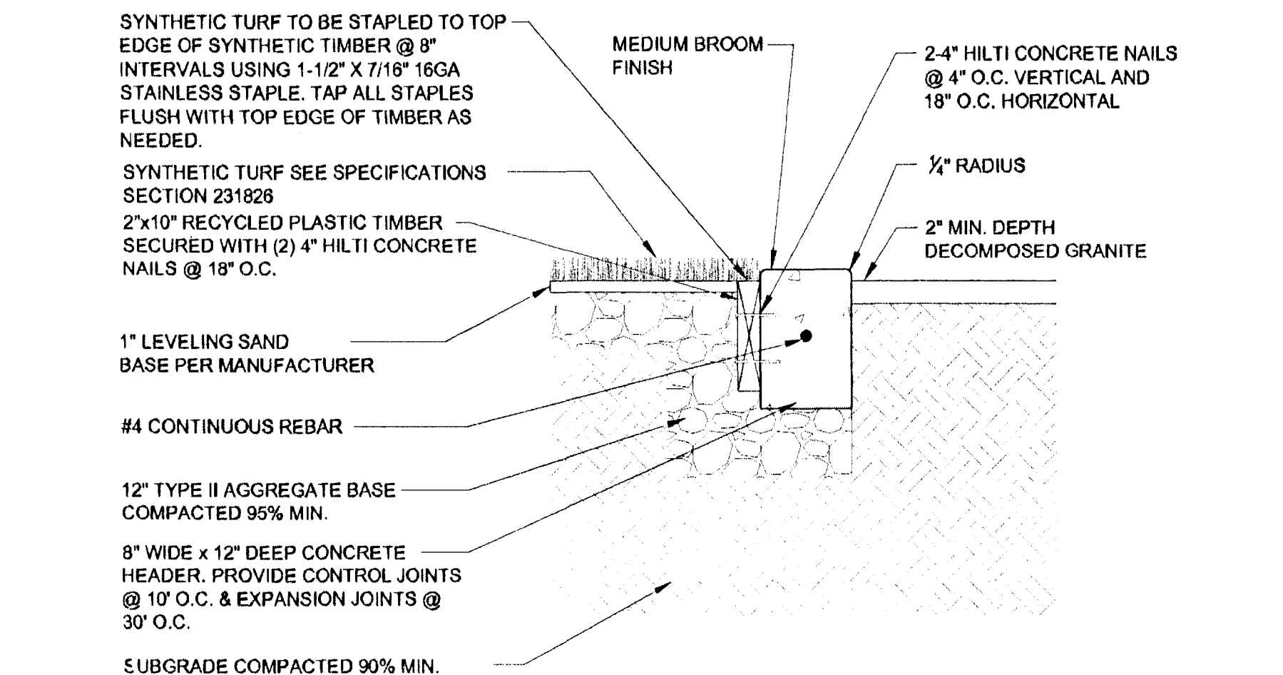
3 SYNTHETIC TURF (ONE SIDE OF CONC. HEADER) SCALE: 1/4" = 1'-0"
