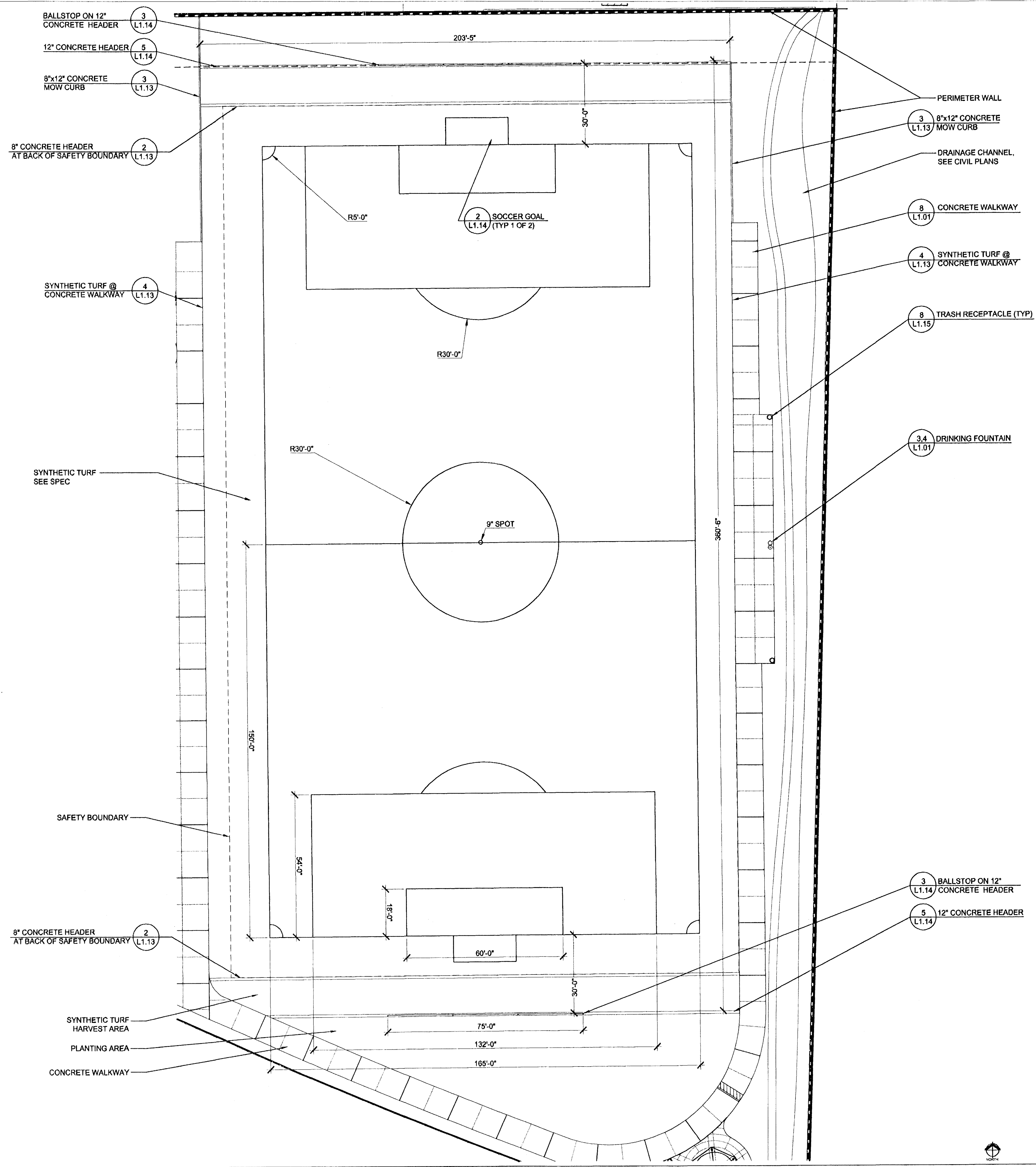
1 SOCCER FIELD LAYOUT SCALE: 1" = 20'-0"
