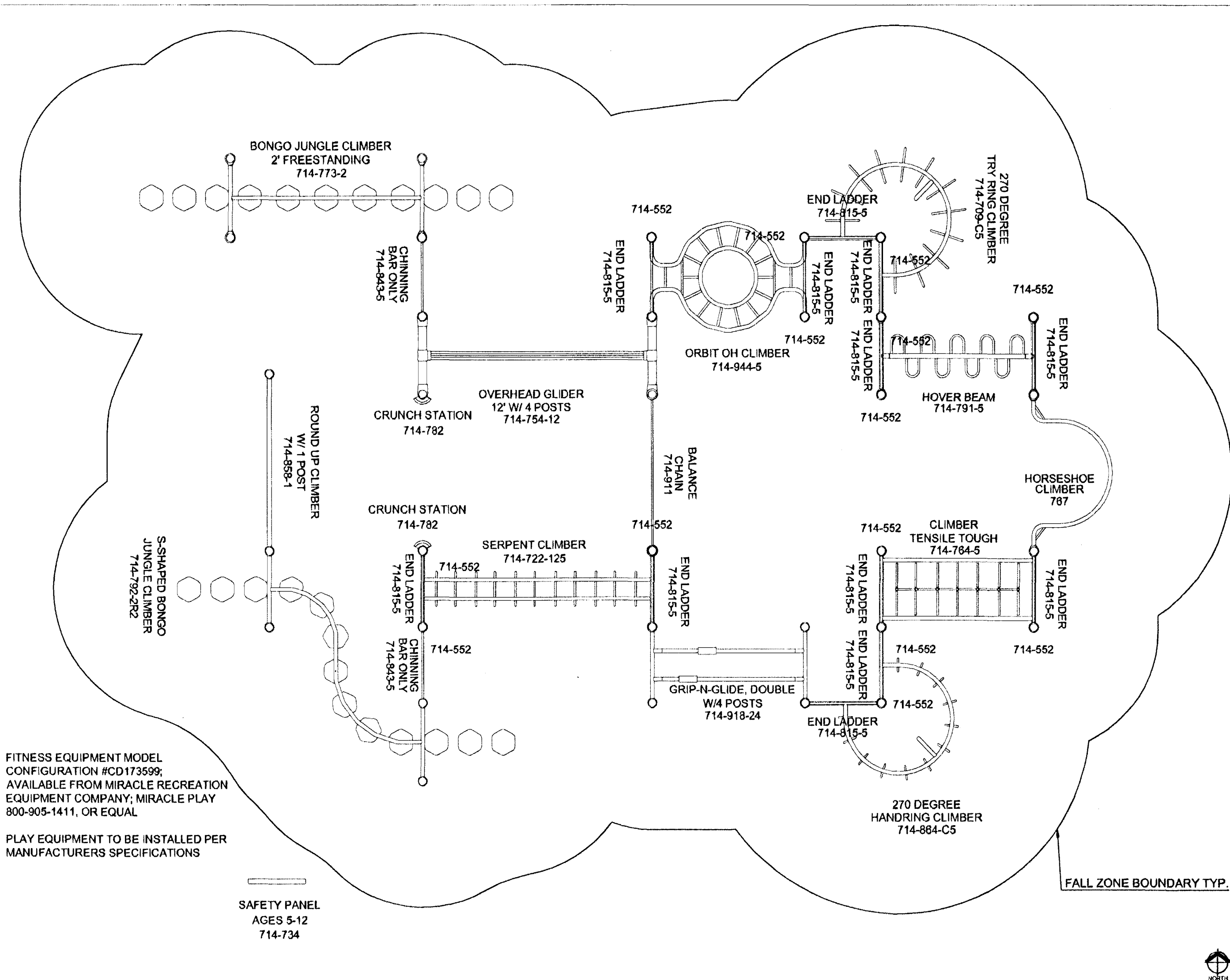
3 FITNESS EQUIPMENT COMPONENT LAYOUT PLAN
