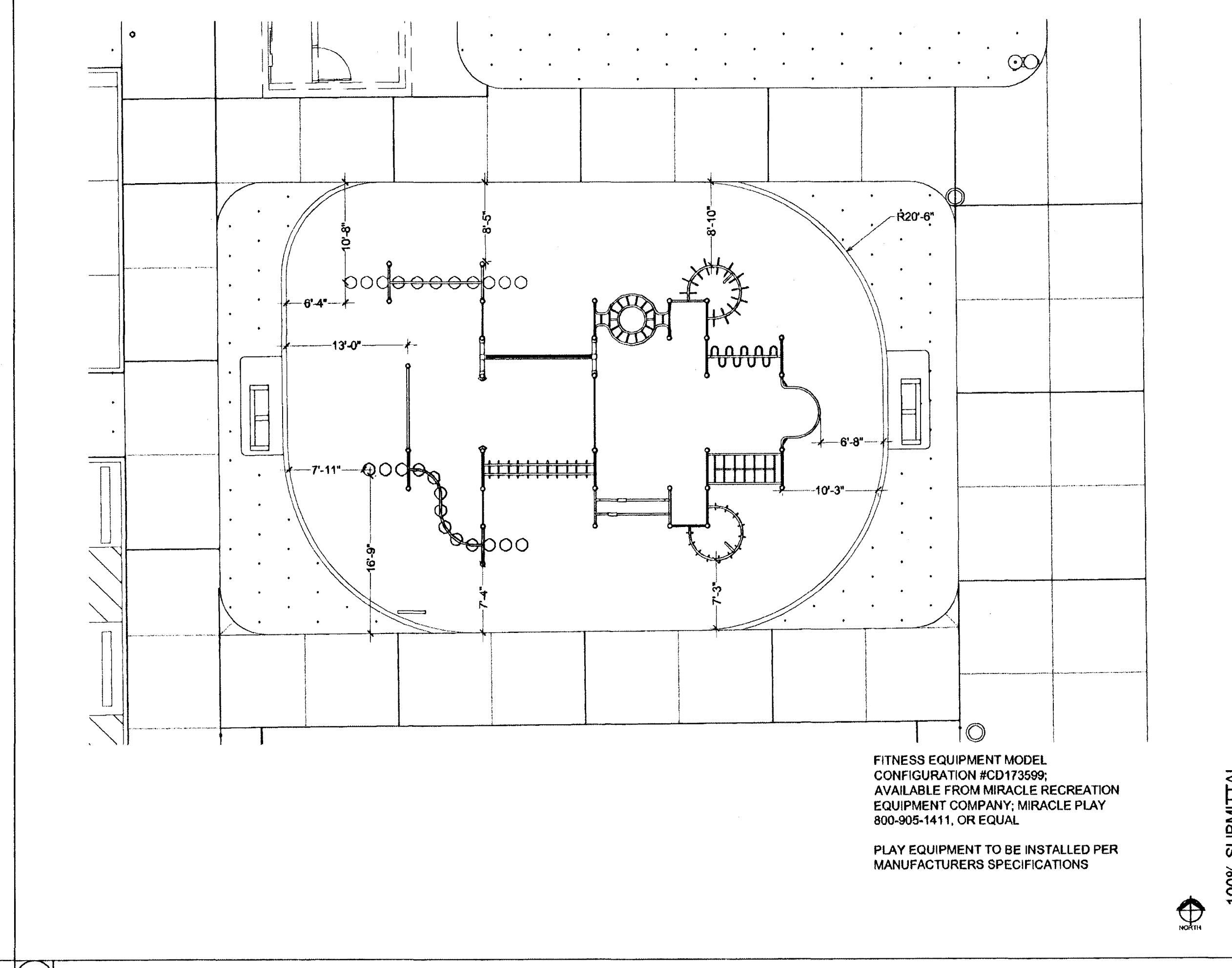
2 FITNESS EQUIPMENT LAYOUT DIMENSION PLAN
