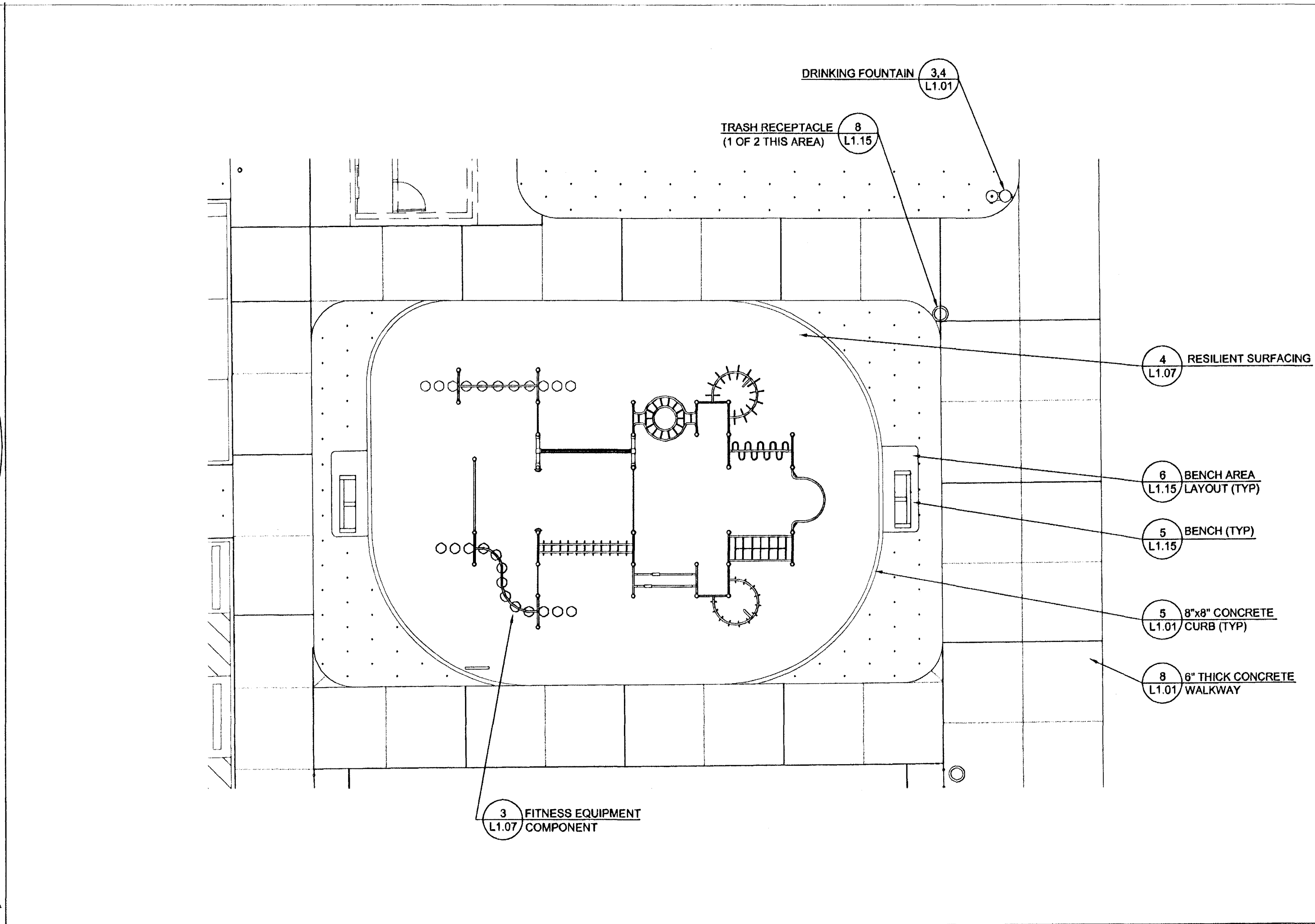
1 FITNESS AREA LAYOUT
