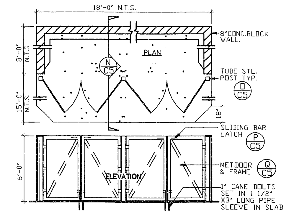
J DOUBLE TRASH ENCLOSURE NO SCALE
