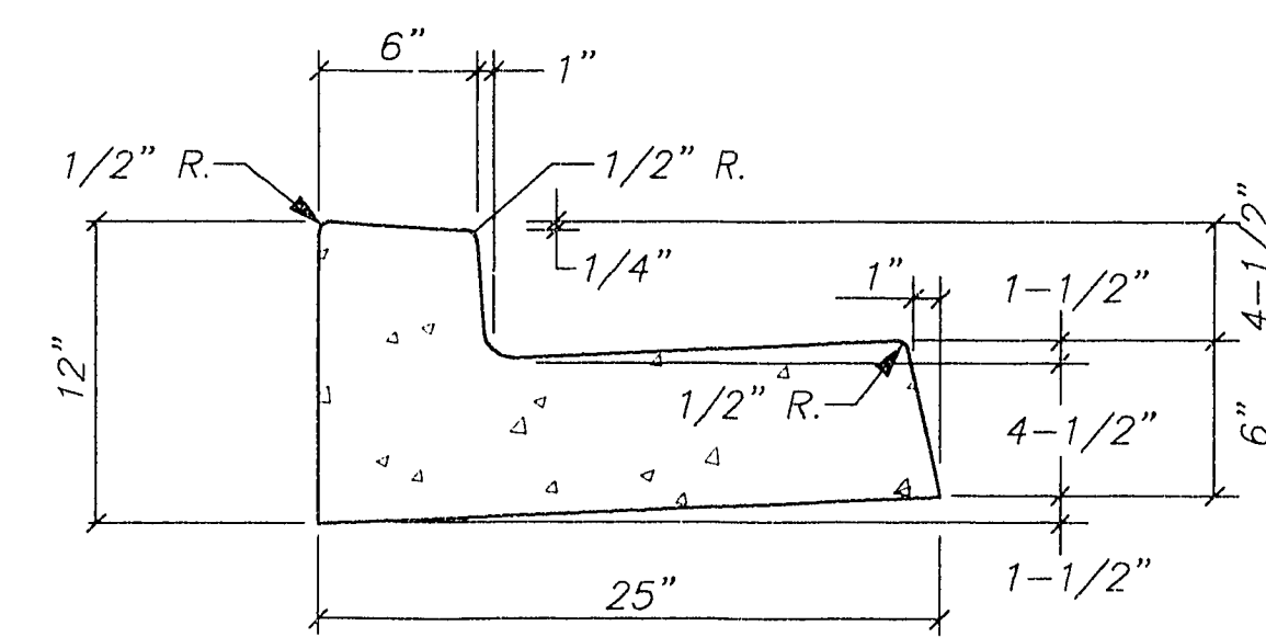
A 'L' TYPE CURB AND GUTTER NO SCALE
