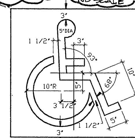
F DISABLED SYMBOL NO SCALE
