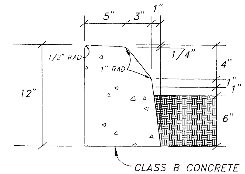
G "A" TYPE CURBING NO SCALE
