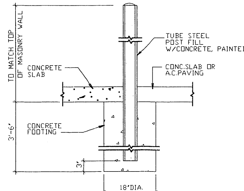
M TRASH ENCLOSURE DOOR POST NO SCALE
