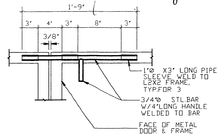
N SLIDING BAR LATCH NO SCALE
