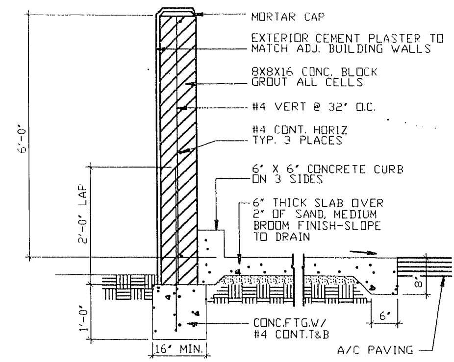
L TRASH ENCLOSURE WALL NO SCALE
