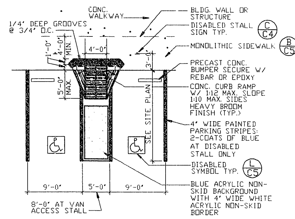
I 90° DISABLED STALL DOUBLE NO SCALE
