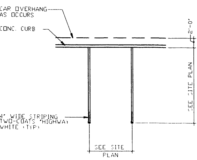
H 90° STALL @ CURB NO SCALE
