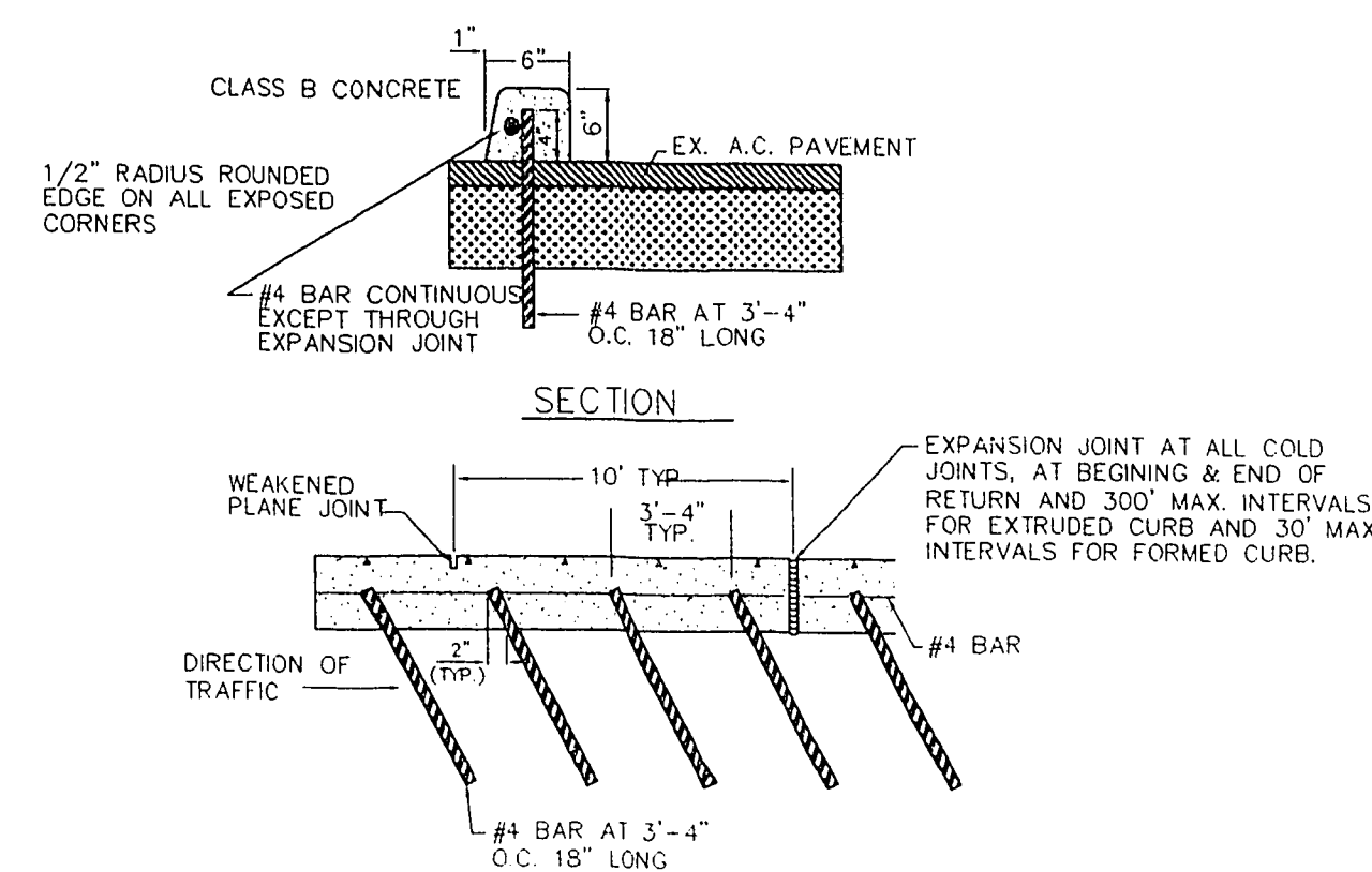
D TACK ON CURB NO SCALE
