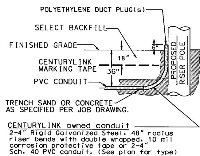
RISER DETAIL (TYPICAL)
