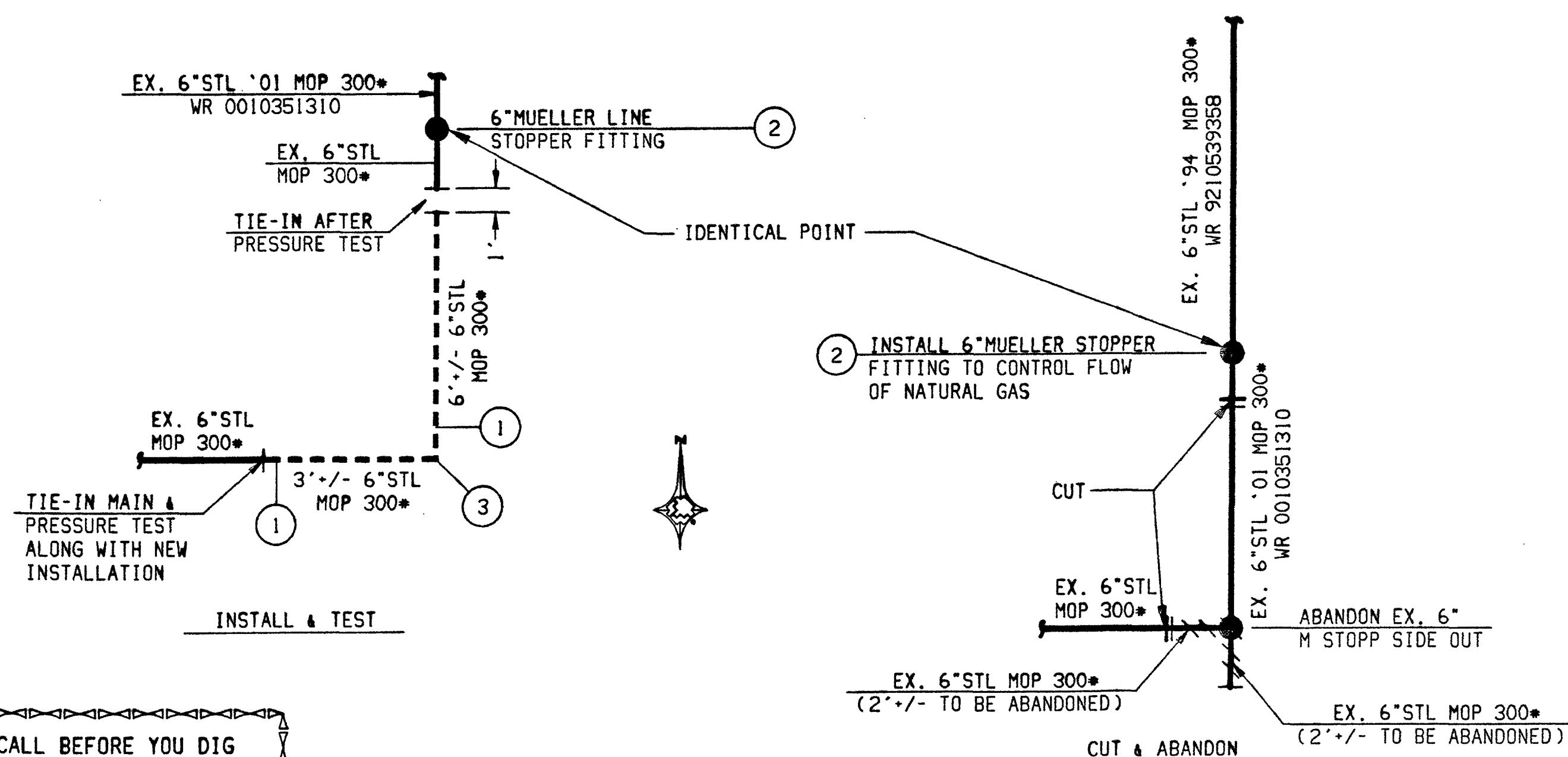
DETAIL "A" NORTH END OF DROP SECTION NTS
