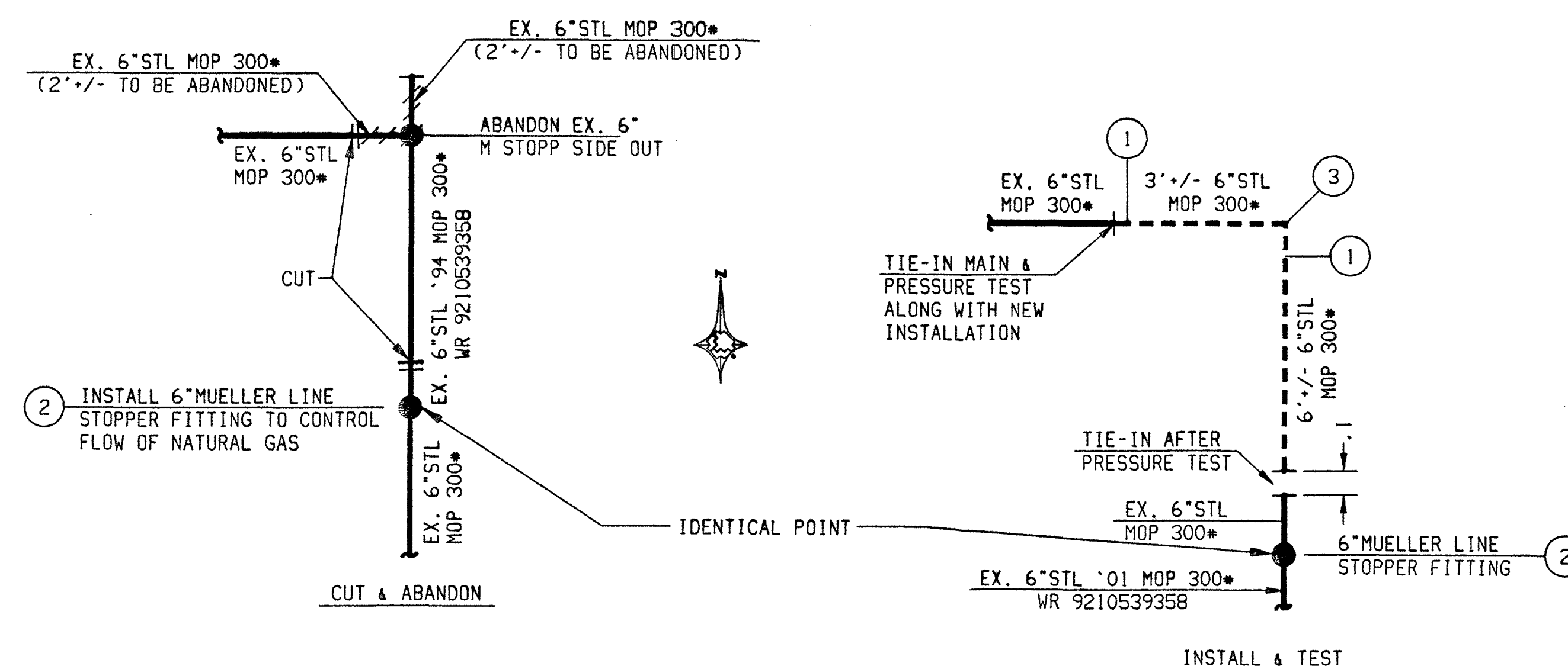
DETAIL "B" SOUTH END OF DROP SECTION NTS
