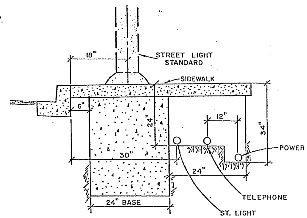
TYPICAL TRENCH DETAIL CITY OF LAS VEGAS
