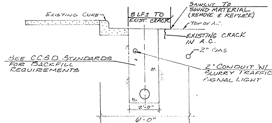
SECTION A-A SCALE 1" = 3'-0"
