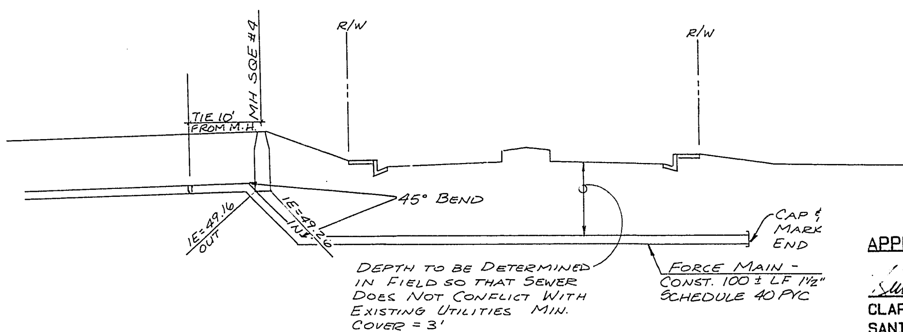
SEWER CROSSING @ ENTRANCE TO QUAIL ESTATES WEST (N.T.D.)
