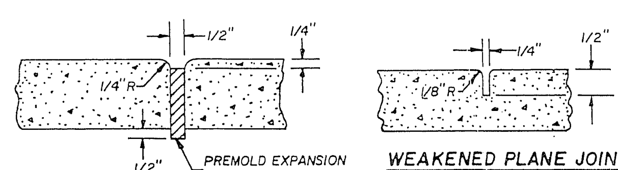
EXPANSION JOINT
