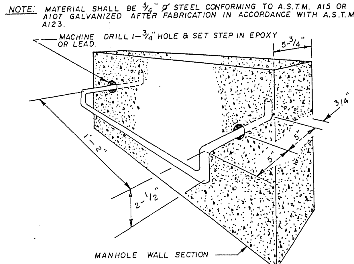
STEP INSTALLATION FOR MANHOLES IN PLACE
