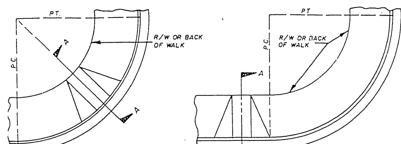
RAMP IN CURB RETURN
