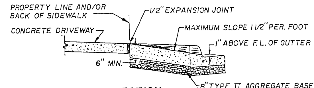
SECTION
