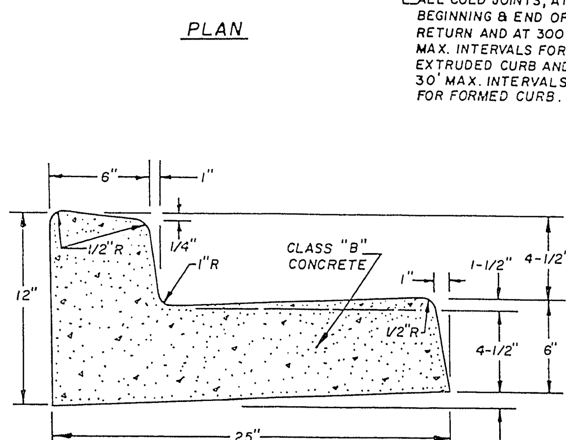
TYPICAL SECTION
