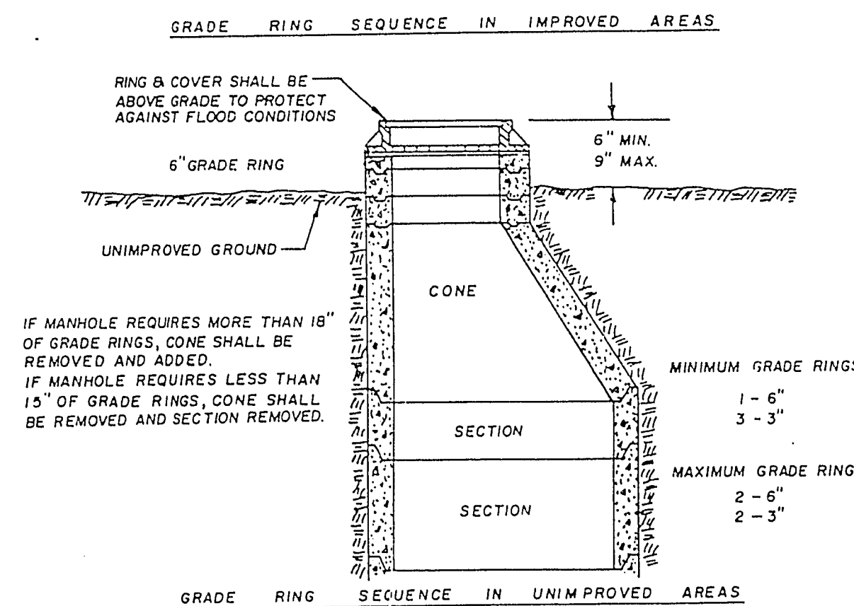
GRADE RING SEQUENCE
