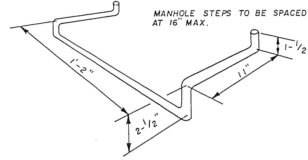
FOR PRE-CAST MANHOLES MADE WITH STEPS
