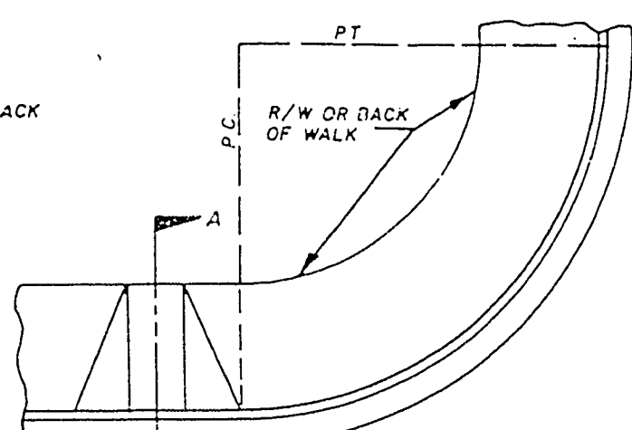
RAMP OUTSIDE CURB RETURN
