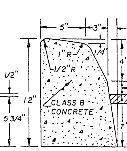
"A" CURB SECTION
