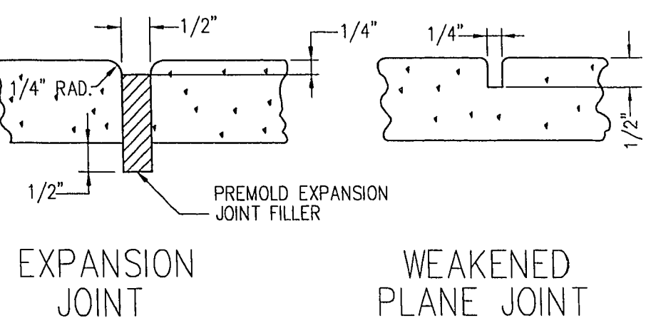
H EXPANSION / CONSTRUCTION JOINT DETAIL N.T.S. UNIFORM STANDARD DWG. No. 234
