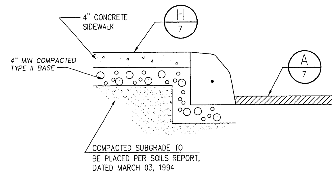
B CONCRETE SIDEWALK DETAIL (ON-SITE ONLY) N.T.S.
