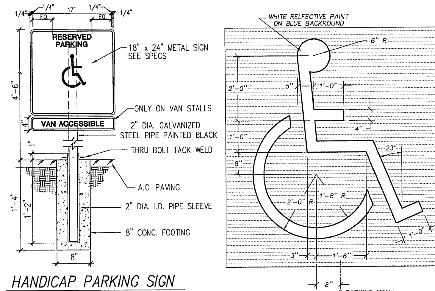
J INTERNATIONAL HANDICAP SYMBOL (ON-SITE ONLY) N.T.S.
