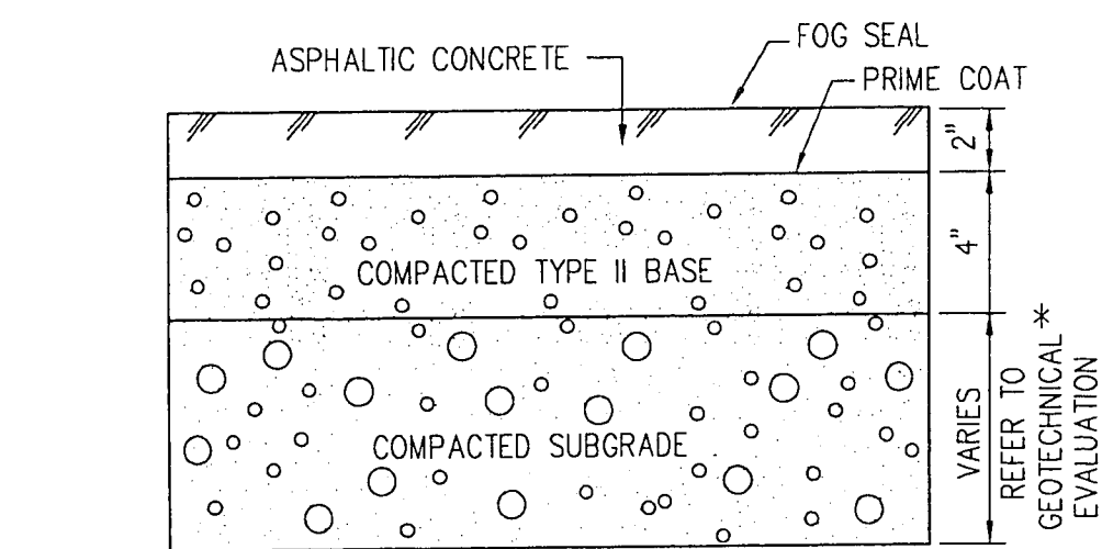
STANDARD DUTY PAVING
