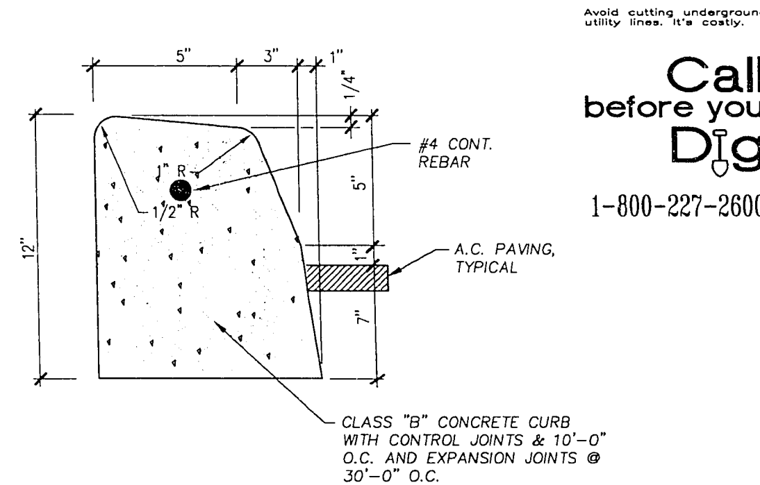
D BUILDING PAD SECTION N.T.S. DEVIATION FROM STANDARD DWG. NO. 219 - HEIGHT CHANGED FROM 5" TO 6"
