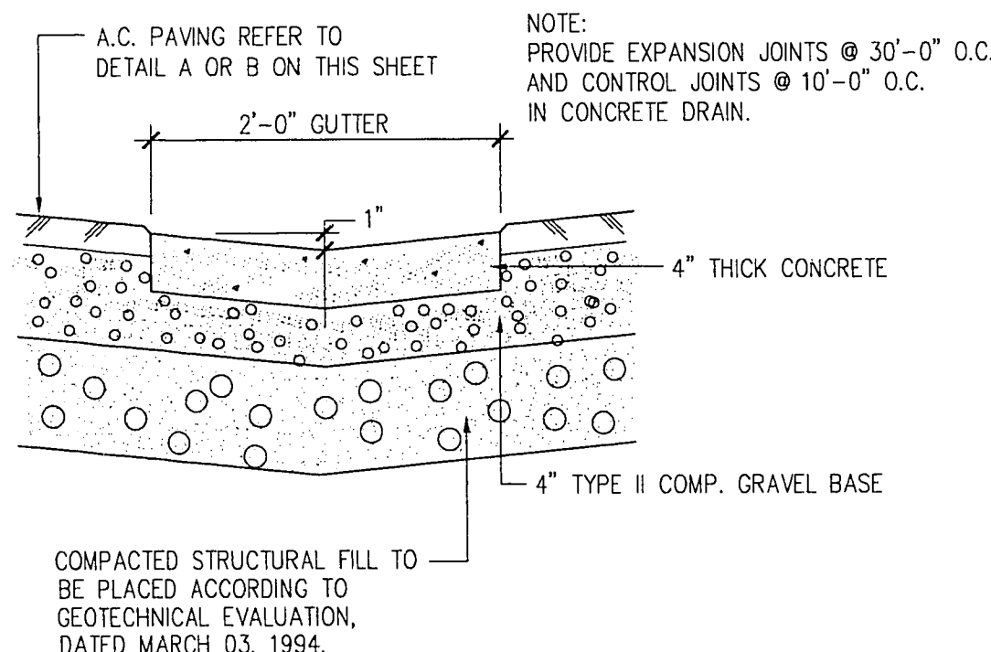
E CONCRETE VALLEY GUTTER (ON-SITE ONLY) N.T.S. NOTE: BASE MATERIAL AND CONCRETE THICKNESS'S TO BE CONFIRMED BY SOILS ENGINEER.
