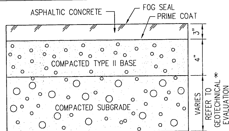
HEAVY DUTY PAVING
