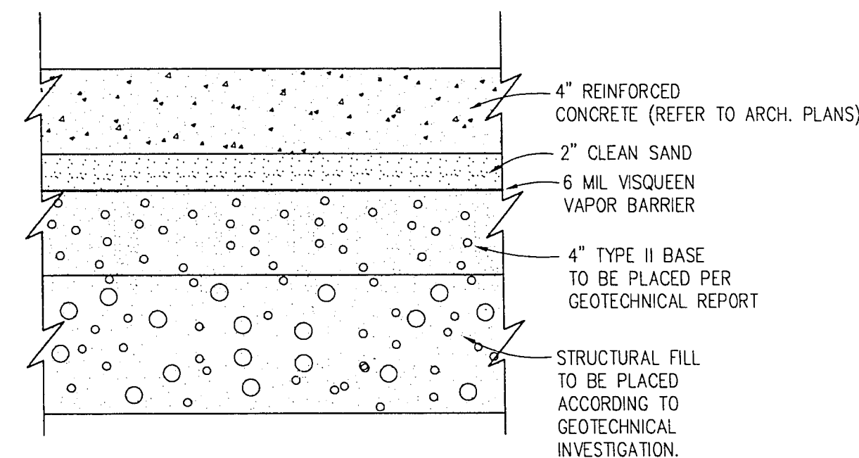
C BUILDING PAD SECTION* N.T.S. * OBTAINED FROM GEOTECHNICAL EVALUATION BY WESTERN TECHNOLOGIES, INC., DATED MARCH 03, 1994.
