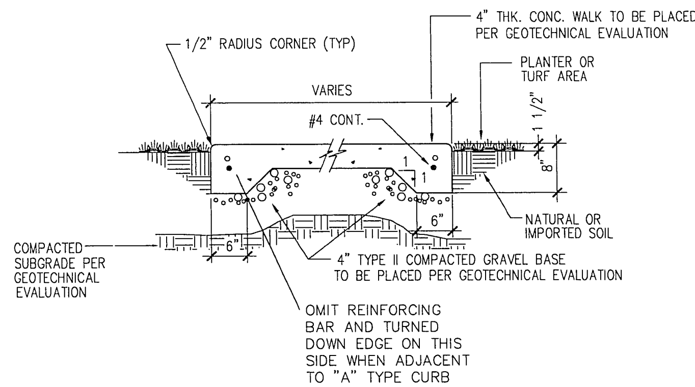
F CONCRETE WALK (ON-SITE ONLY) N.T.S. NOTE: BASE MATERIAL AND CONCRETE THICKNESS'S TO BE CONFIRMED BY SOILS ENGINEER.
