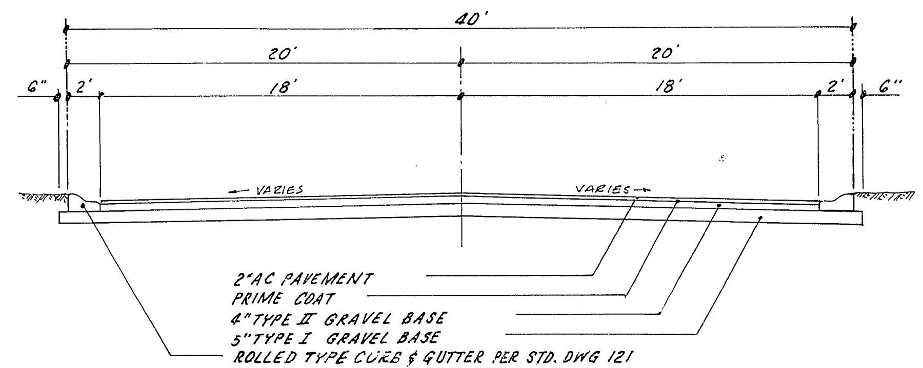
STREET SECTION - PRIVATE DRIVE
