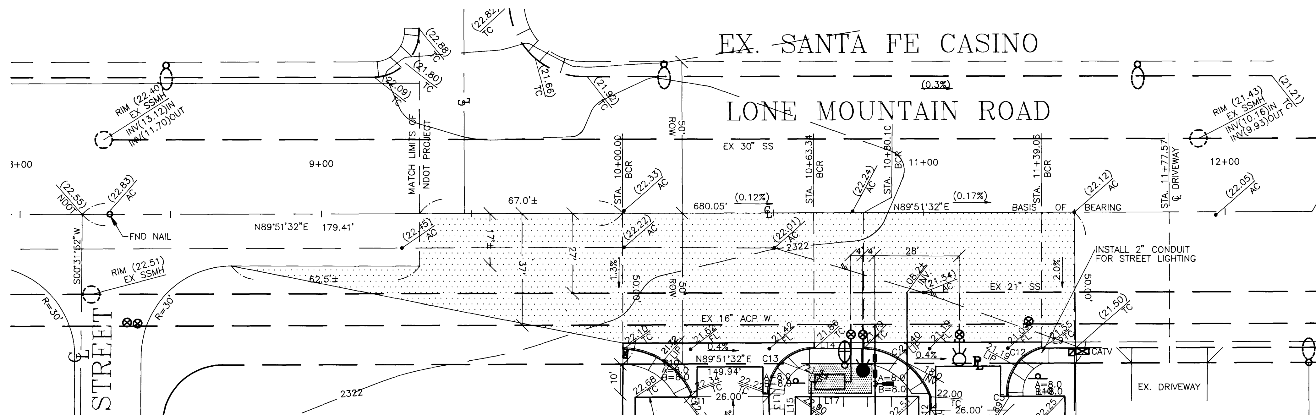
PLAN: LONE MOUNTAIN ROAD SCALE: (HORIZ.) 1"=20'
