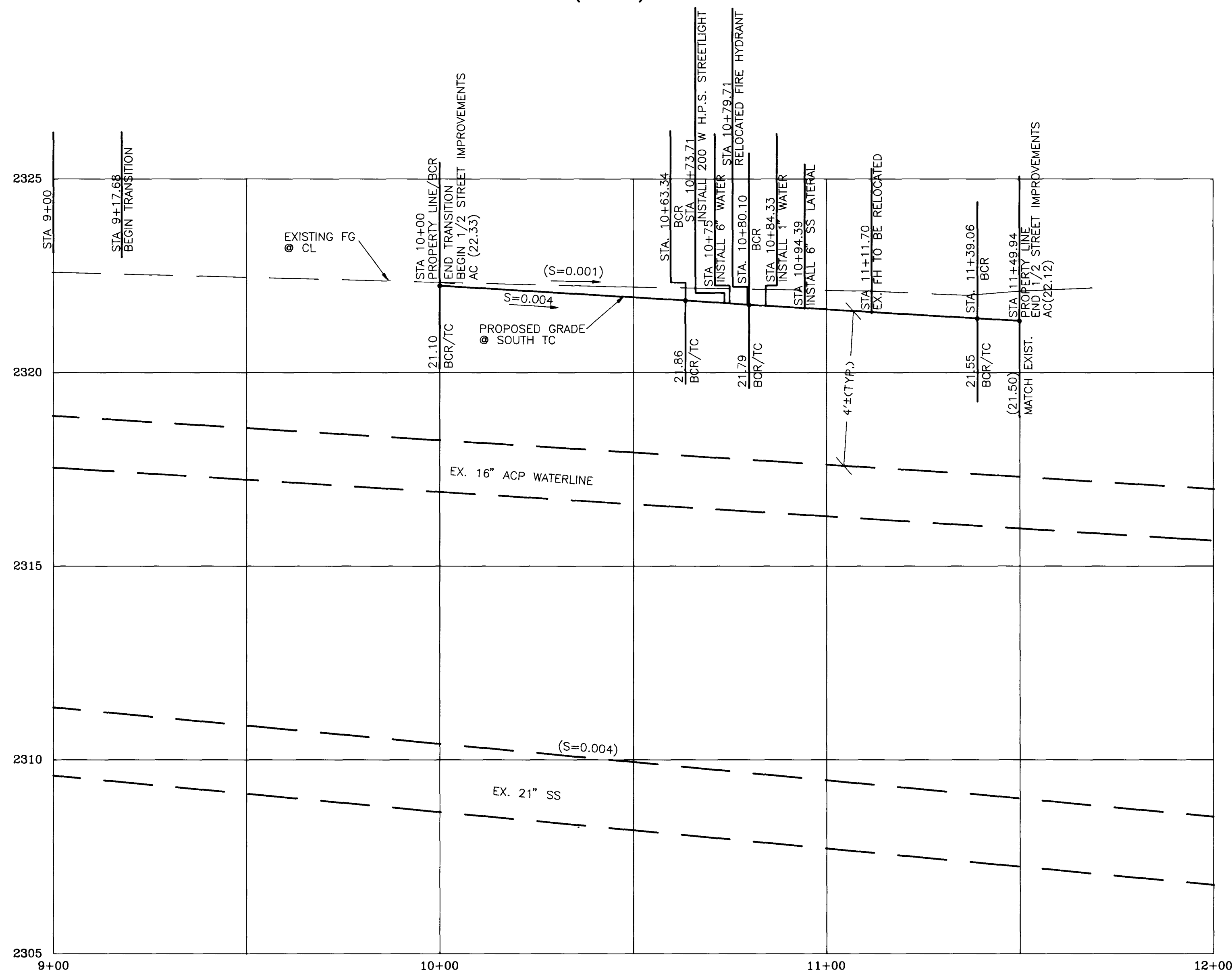
PROFILE: LONE MOUNTAIN ROAD SCALE: (HORIZ.) 1"=20' (VERT.) 1"=2'
