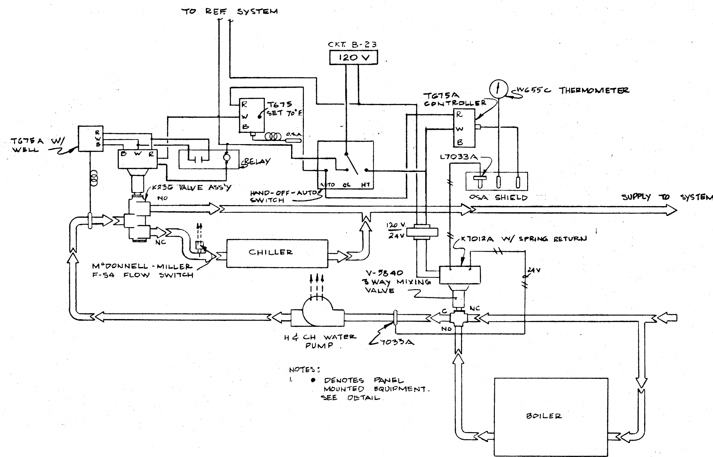
SUMMER - WINTER CHANGEOVER CONTROL NO SCALE
