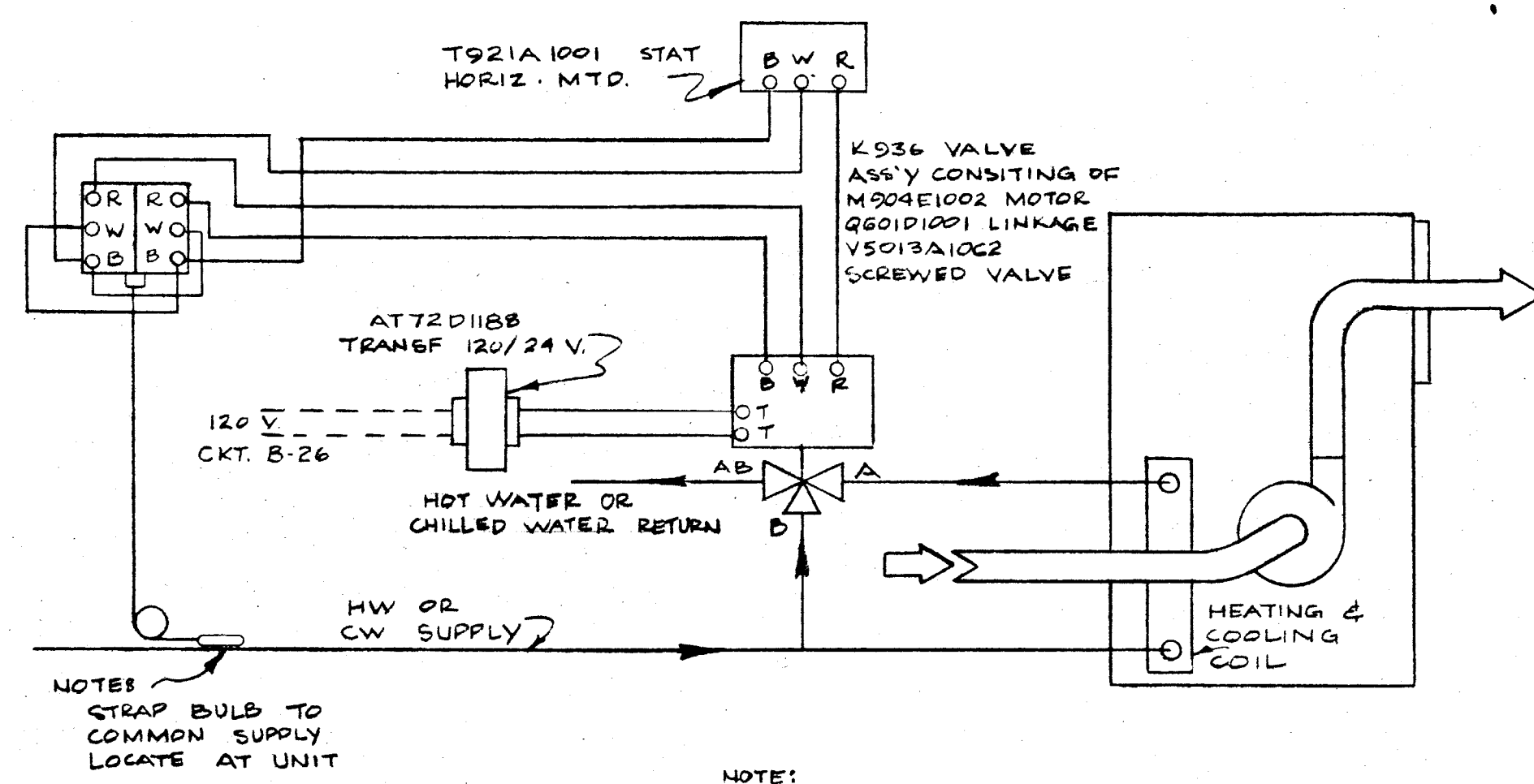
A.C. #1 & #2 CONTROL NO SCALE
