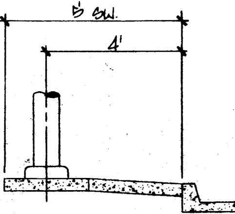
STREET LIGHT DETAIL
