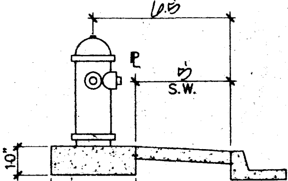
FIRE HYDRANT DETAIL
