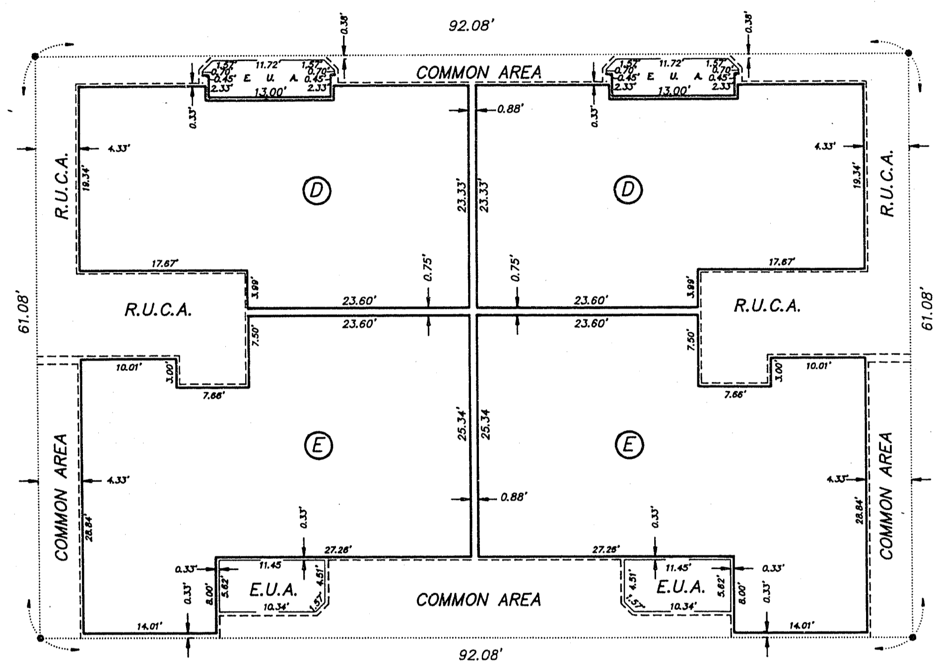
BUILDING TYPE III - SECOND FLOOR
