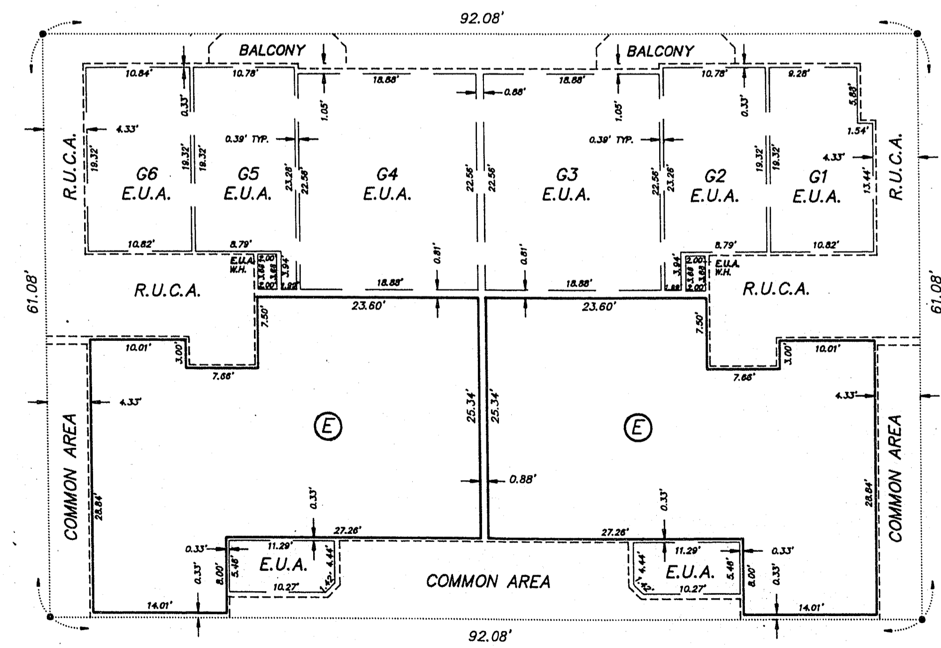
BUILDING TYPE III - FIRST FLOOR
