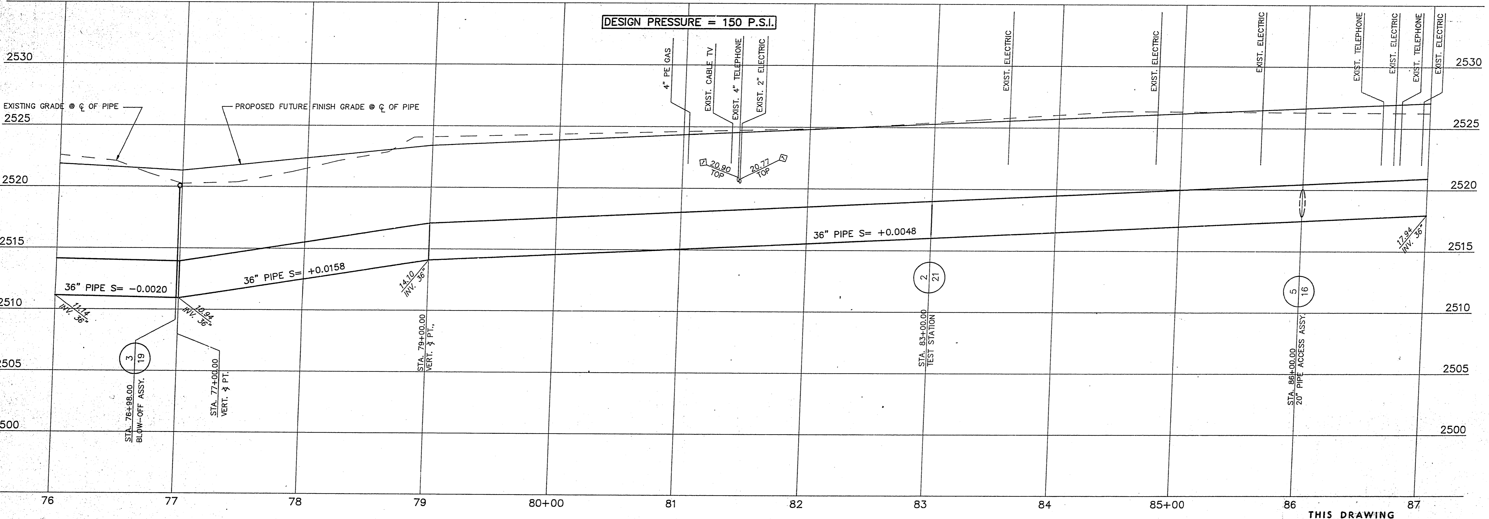
PROFILE HORIZ. 1" = 40' VERT. 1" = 4'
